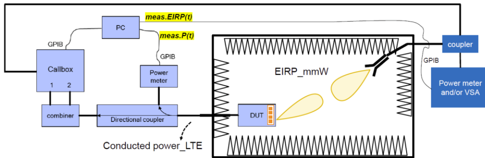
Figure 7-1 mmW NR radiated power measurement setup – Test Setup Photo 10
