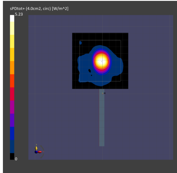
Figure 12-2 4cm 2 psPD distribution measured at input.power.limit of 2.1 dBm on the left edge for n260 beam 14
