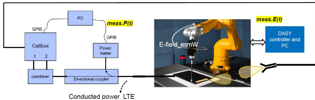
Figure 7-2 Power Density Measurement Setup – Test Setup Photo 11
