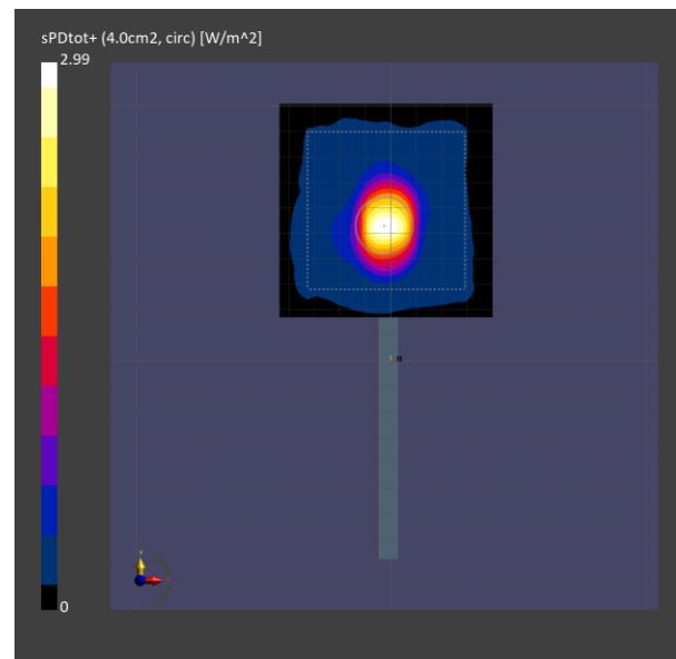
Figure 12-2 4cm 2 psPD distribution measured at input.power.limit of 2.1 dBm on the left edge for n260 beam 14
