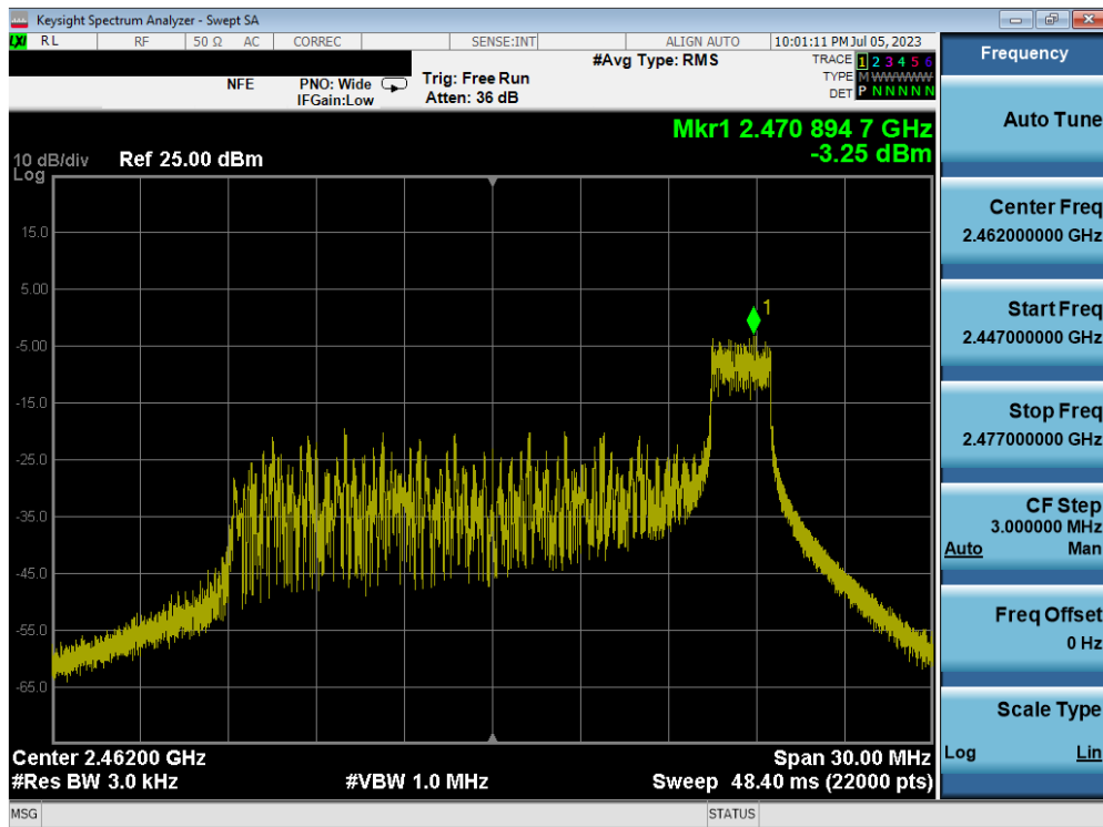
Plot 7-33. Power Spectral Density Plot MIMO ANT2 (802.11ax OFDMA – 26 Tones – Ch. 11) – ANT 2
