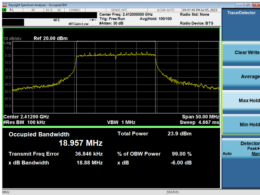
Plot 7-10. 6dB Bandwidth Plot MIMO ANT1 (802.11ax OFDMA – 242 Tones – Ch. 1) – ANT 1
