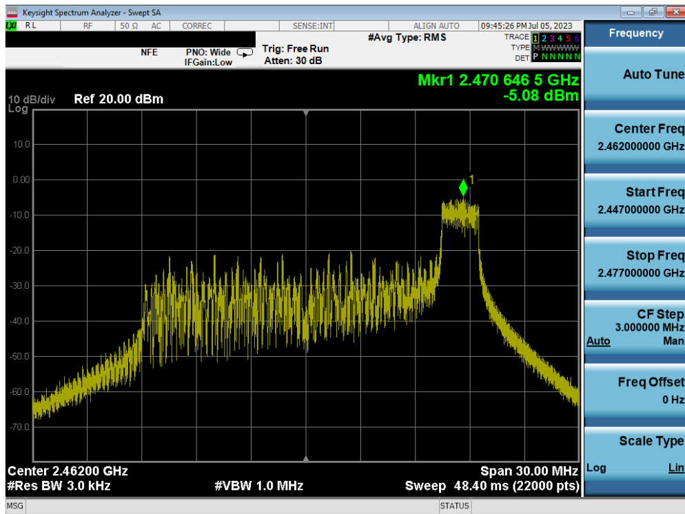
Plot 7-27. Power Spectral Density Plot MIMO ANT1 (802.11ax OFDMA – 26 Tones – Ch. 11) – ANT 1
