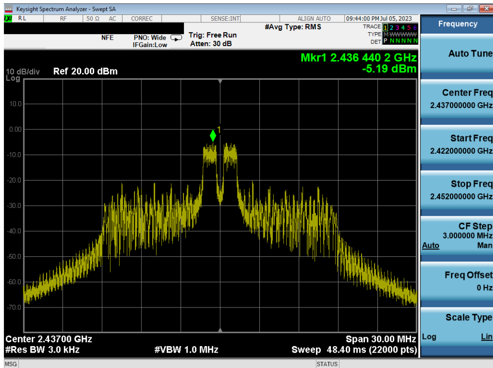
Plot 7-26. Power Spectral Density Plot MIMO ANT1 (802.11ax OFDMA – 26 Tones – Ch. 6) – ANT 1
