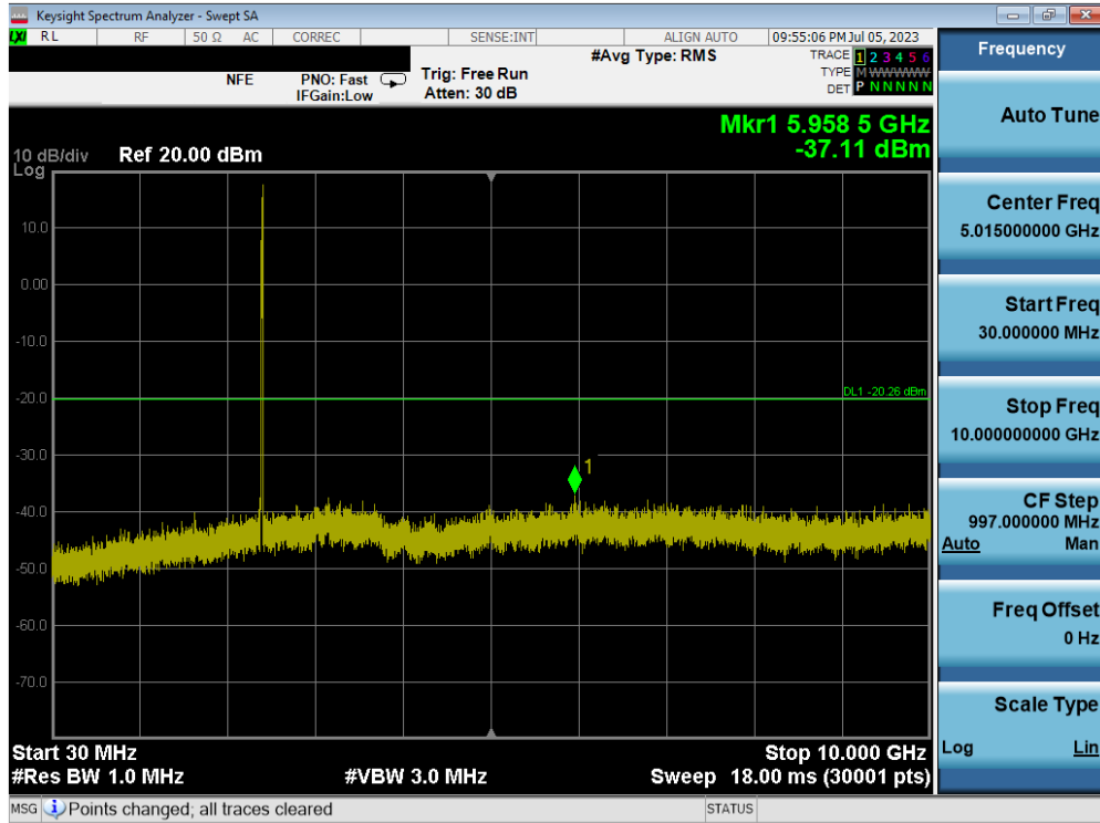
Plot 7-85. Conducted Spurious Plot MIMO ANT2 (802.11ax OFDMA – 26 Tones – Ch. 1) – ANT 2
