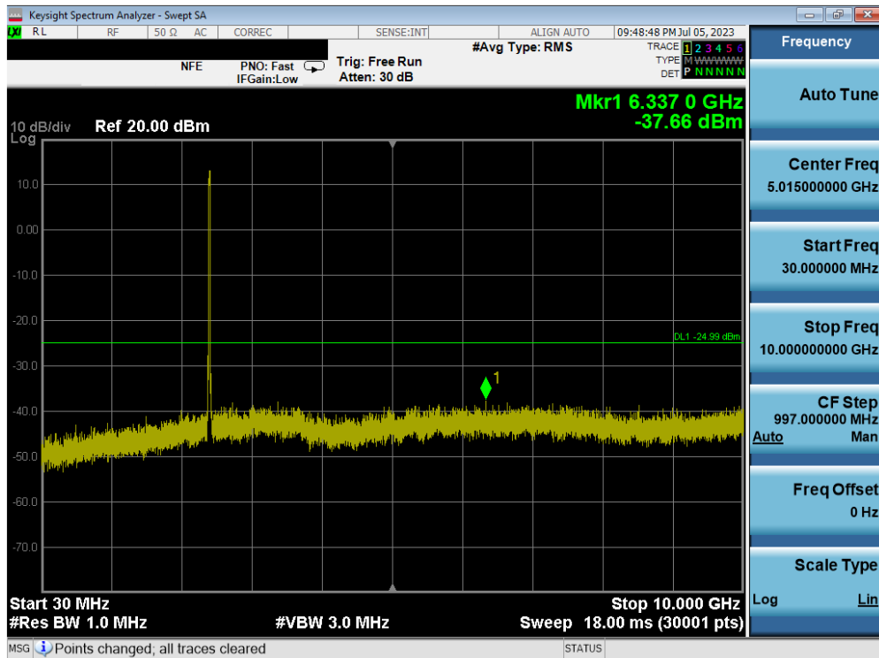
Plot 7-79. Conducted Spurious Plot MIMO ANT1 (802.11ax OFDMA – 242 Tones – Ch. 1) – ANT 1
