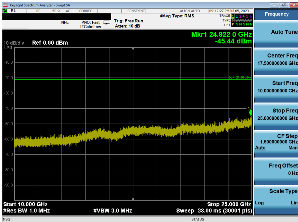
Plot 7-74. Conducted Spurious Plot MIMO ANT1 (802.11ax OFDMA – 26 Tones – Ch. 1) – ANT 1
