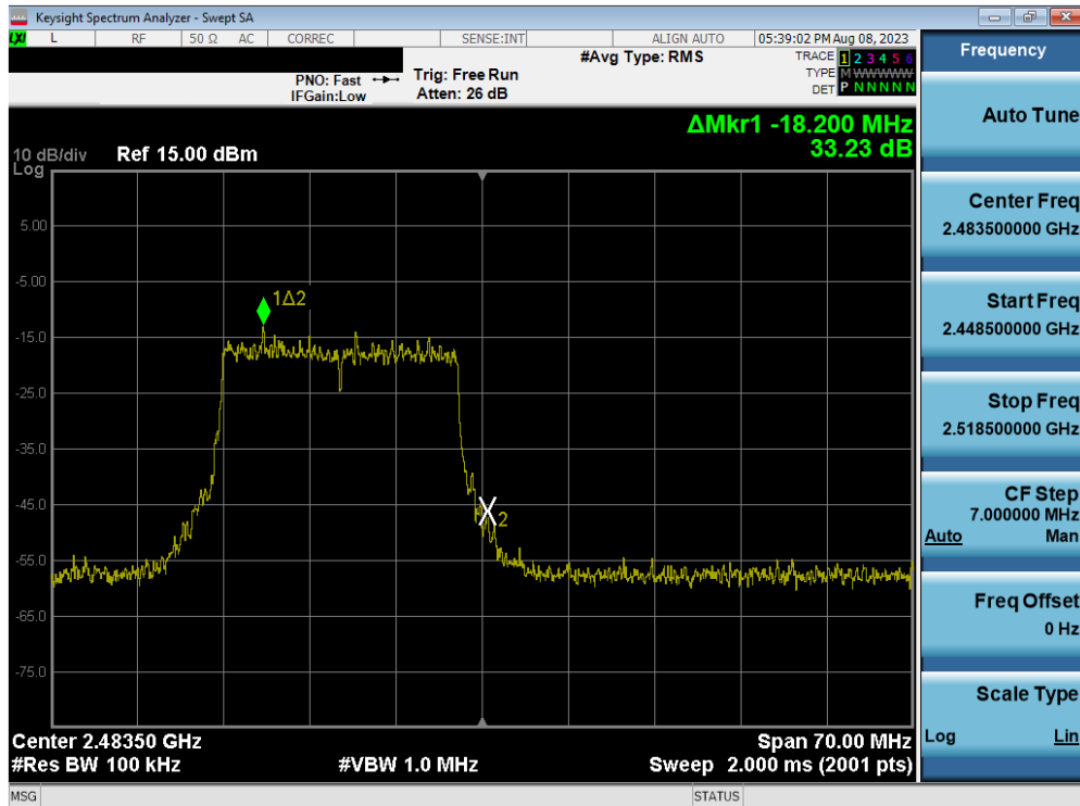
Plot 7-60. Band Edge Plot MIMO ANT2 (802.11ax OFDMA – 242 Tones – Ch. 13) – ANT 2
