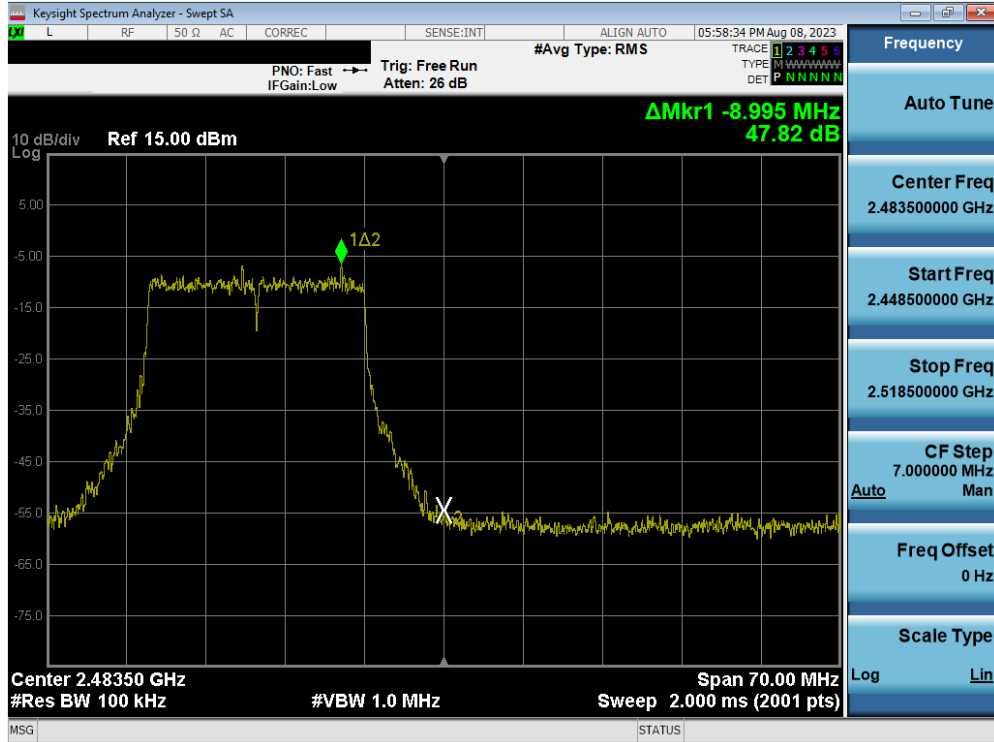
Plot 7-51. Band Edge Plot MIMO ANT1 (802.11ax OFDMA – 242 Tones – Ch. 12) – ANT 1
