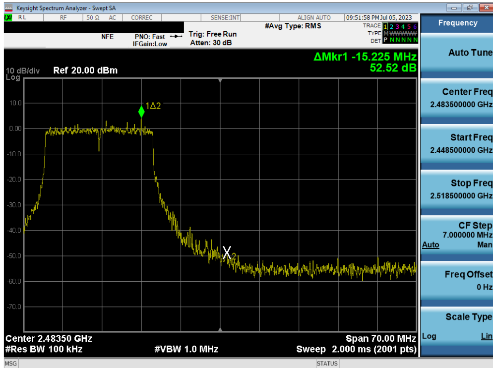
Plot 7-50. Band Edge Plot MIMO ANT1 (802.11ax OFDMA – 242 Tones – Ch. 11) – ANT 1
