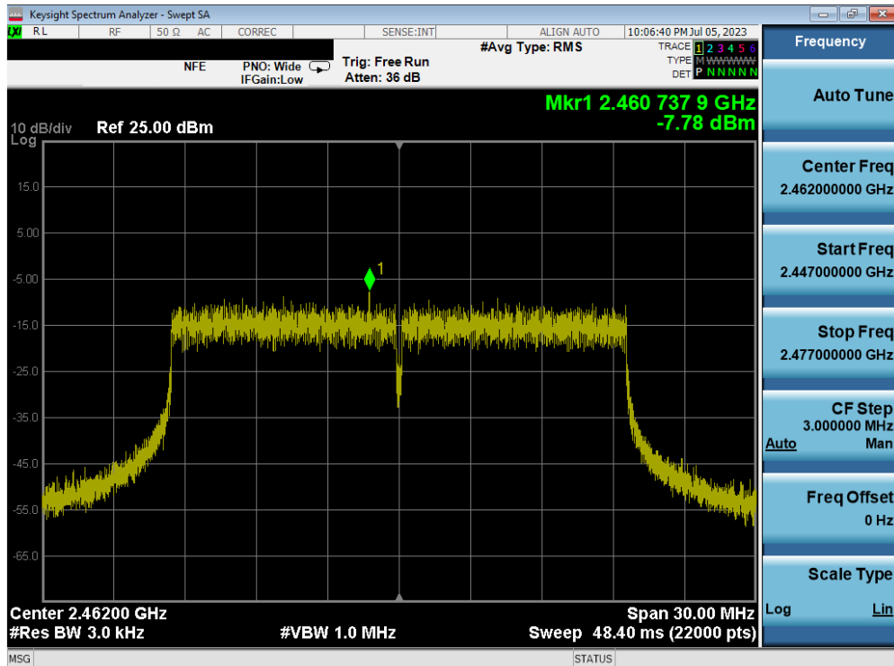
Plot 7-36. Power Spectral Density Plot MIMO ANT2 (802.11ax OFDMA – 242 Tones – Ch. 11) – ANT 2
