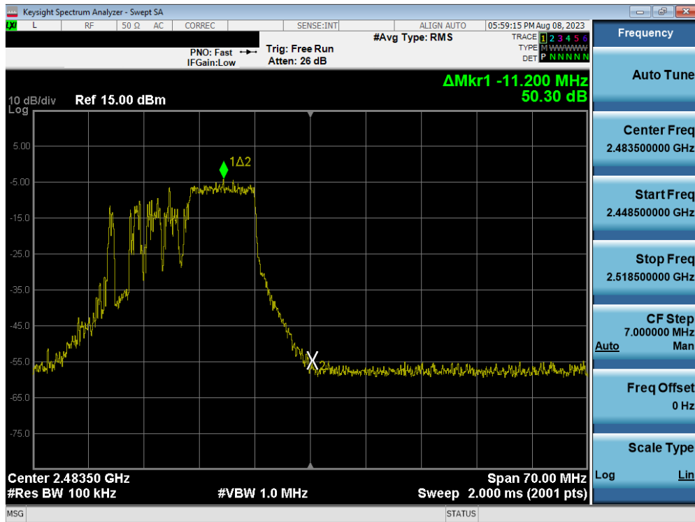
Plot 7-47. Band Edge Plot MIMO ANT1 (802.11ax OFDMA – 106 Tones – Ch. 12) – ANT 1
