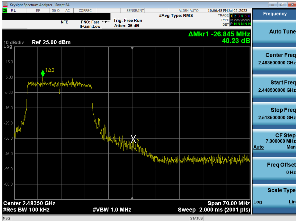
Plot 7-58. Band Edge Plot MIMO ANT2 (802.11ax OFDMA – 242 Tones – Ch. 11) – ANT 2
