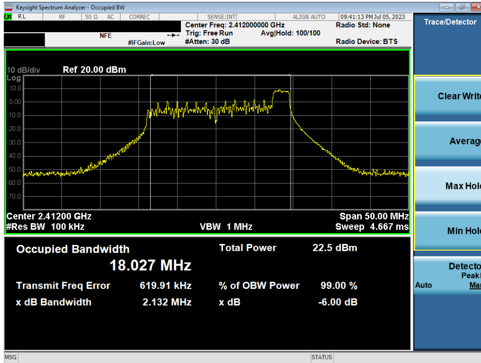
Plot 7-7. 6dB Bandwidth Plot MIMO ANT1 (802.11ax OFDMA – 26 Tones – Ch. 1) – ANT 1
