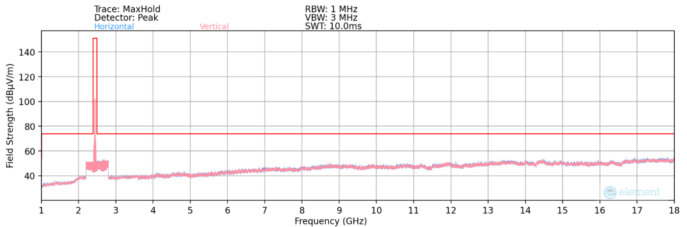
Plot 7-102. Radiated Spurious Plot above 1GHz SISO ANT2 (802.11ax OFDMA – 242 Tones – Ch. 6)
