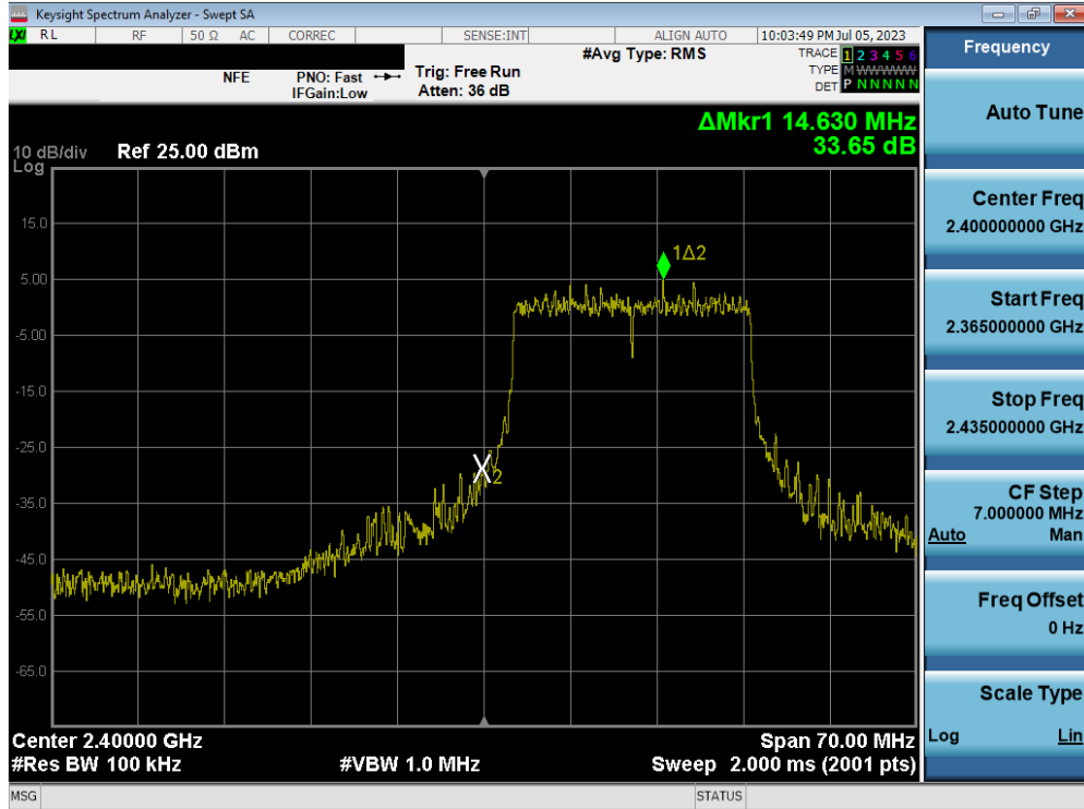
Plot 7-57. Band Edge Plot MIMO ANT2 (802.11ax OFDMA – 242 Tones – Ch. 1) – ANT 2
