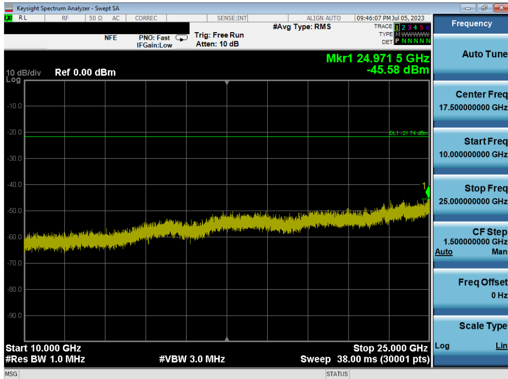
Plot 7-78. Conducted Spurious Plot MIMO ANT1 (802.11ax OFDMA – 26 Tones – Ch. 11) – ANT 1
