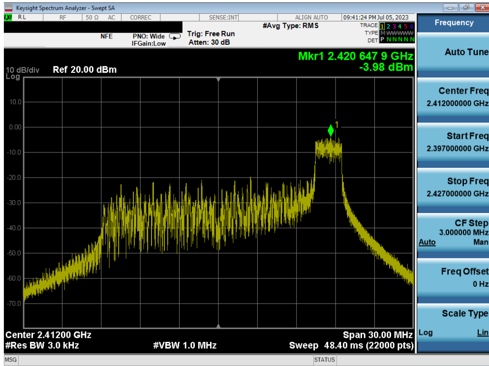
Plot 7-25. Power Spectral Density Plot MIMO ANT1 (802.11ax OFDMA – 26 Tones – Ch. 1) – ANT 1
