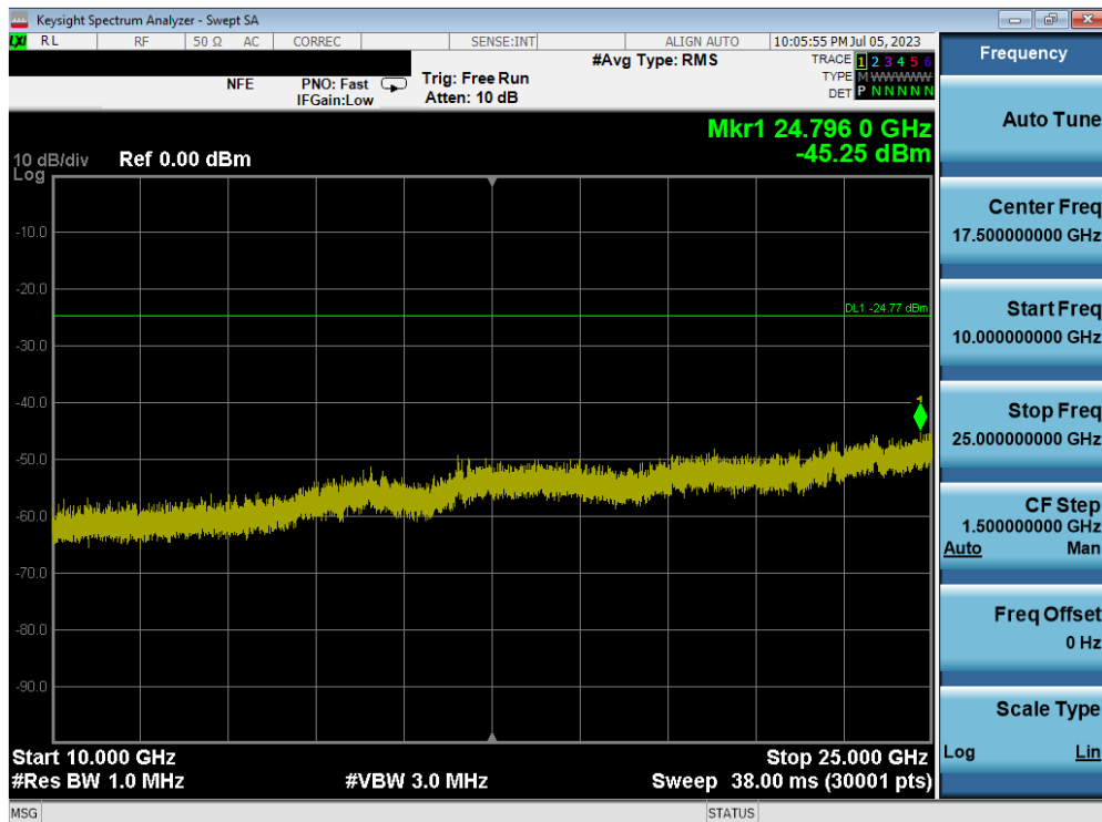
Plot 7-94. Conducted Spurious Plot MIMO ANT2 (802.11ax OFDMA – 242 Tones – Ch. 6) – ANT 2
