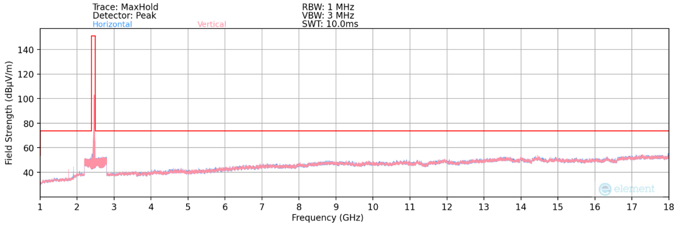
Plot 7-103. Radiated Spurious Plot above 1GHz SISO ANT2 (802.11ax OFDMA – 242 Tones – Ch. 11)
