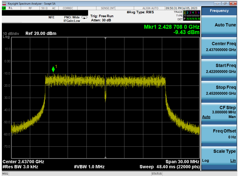
Plot 7-29. Power Spectral Density Plot MIMO ANT1 (802.11ax OFDMA – 242 Tones – Ch. 6) – ANT 1
