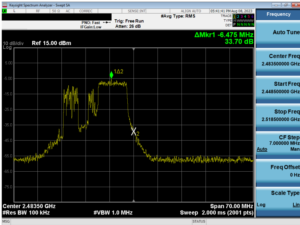
Plot 7-55. Band Edge Plot MIMO ANT2 (802.11ax OFDMA – 106 Tones – Ch. 12) – ANT 2
