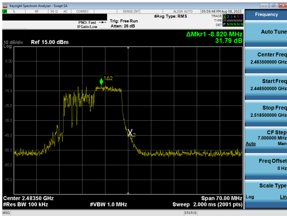
Plot 7-48. Band Edge Plot MIMO ANT1 (802.11ax OFDMA – 106 Tones – Ch. 13) – ANT 1
