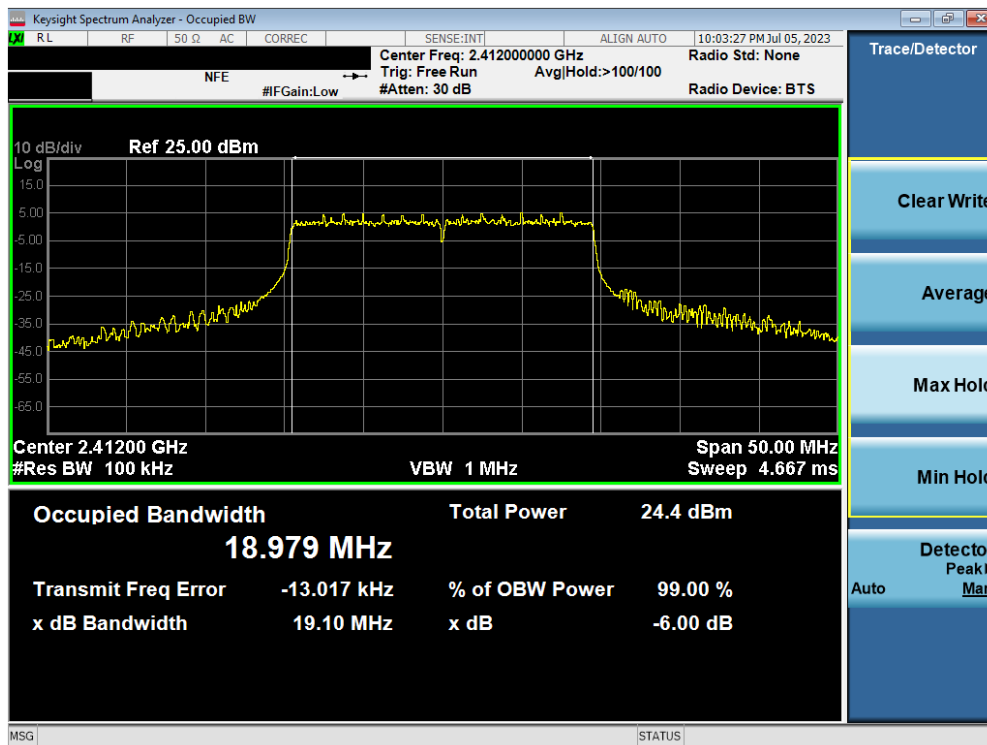
Plot 7-16. 6dB Bandwidth Plot MIMO ANT2 (802.11ax OFDMA – 242 Tones – Ch. 1) – ANT 2
