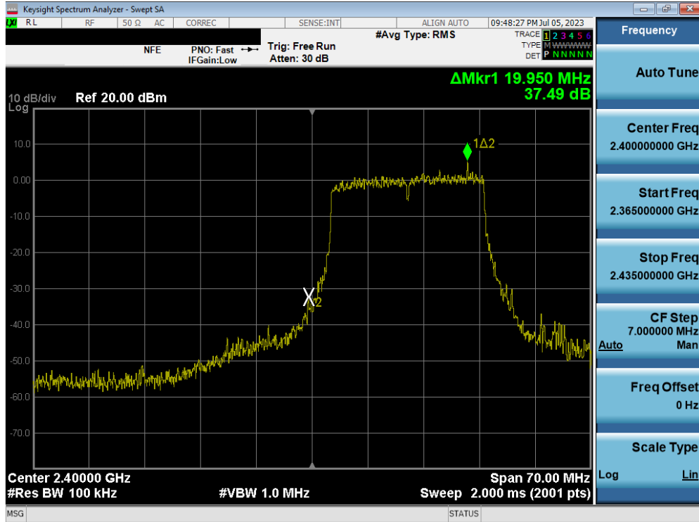
Plot 7-49. Band Edge Plot MIMO ANT1 (802.11ax OFDMA – 242 Tones – Ch. 1) – ANT 1
