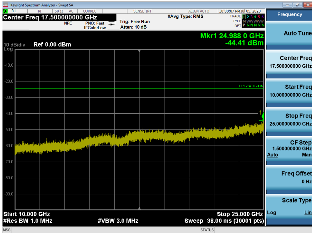
Plot 7-96. Conducted Spurious Plot MIMO ANT2 (802.11ax OFDMA – 242 Tones – Ch. 11) – ANT 2
