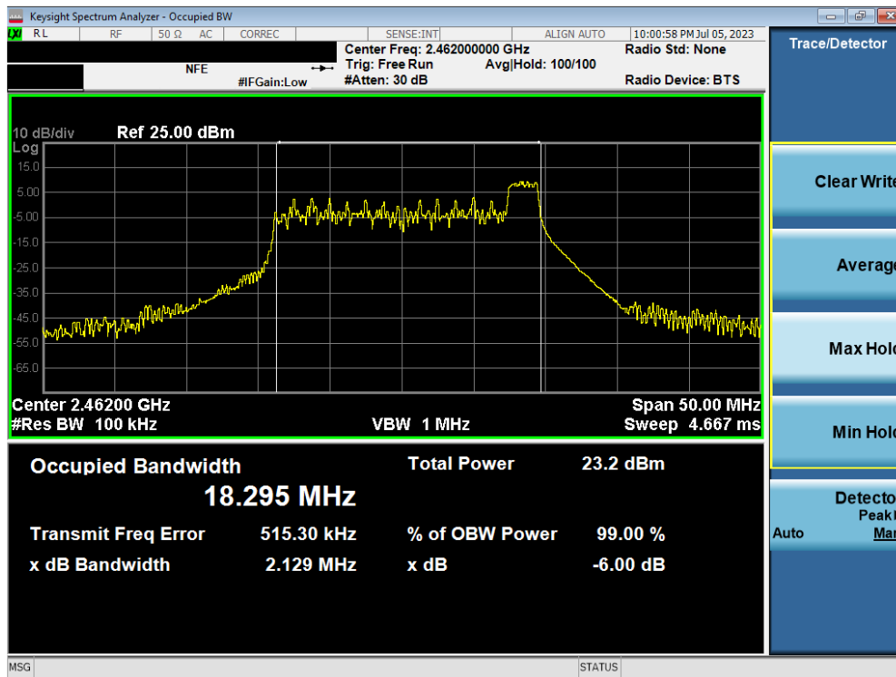
Plot 7-15. 6dB Bandwidth Plot MIMO ANT2 (802.11ax OFDMA – 26 Tones – Ch. 11) – ANT 2
