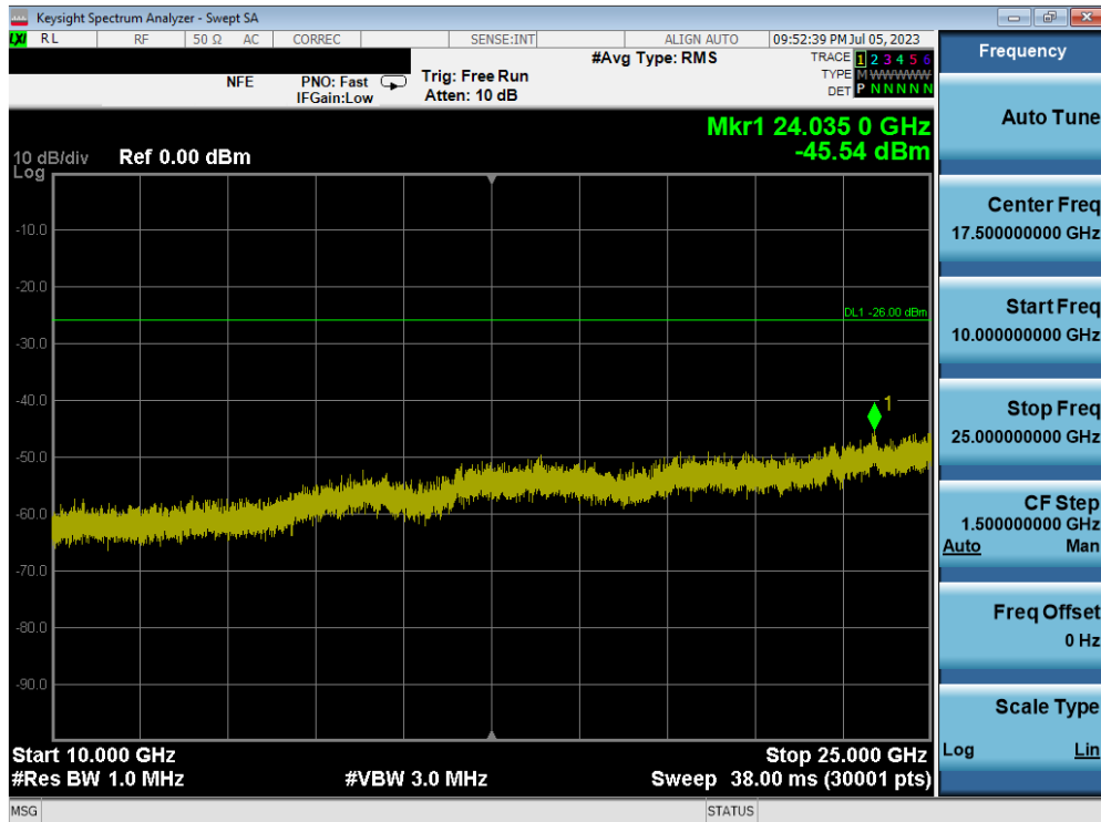
Plot 7-84. Conducted Spurious Plot MIMO ANT1 (802.11ax OFDMA – 242 Tones – Ch. 11) – ANT 1
