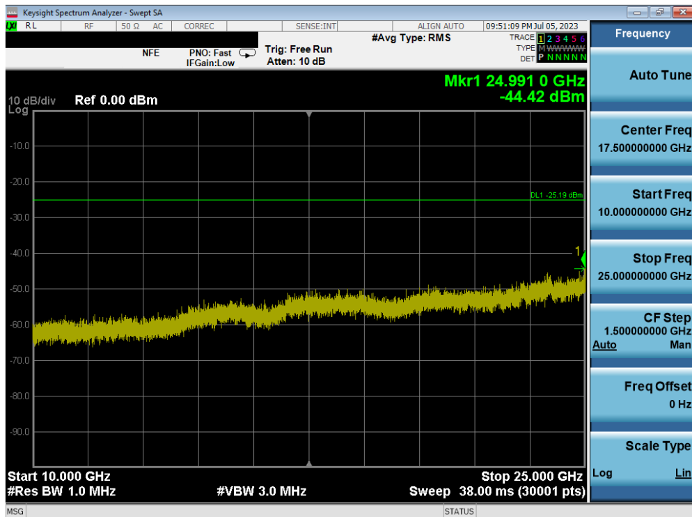
Plot 7-82. Conducted Spurious Plot MIMO ANT1 (802.11ax OFDMA – 242 Tones – Ch. 6) – ANT 1
