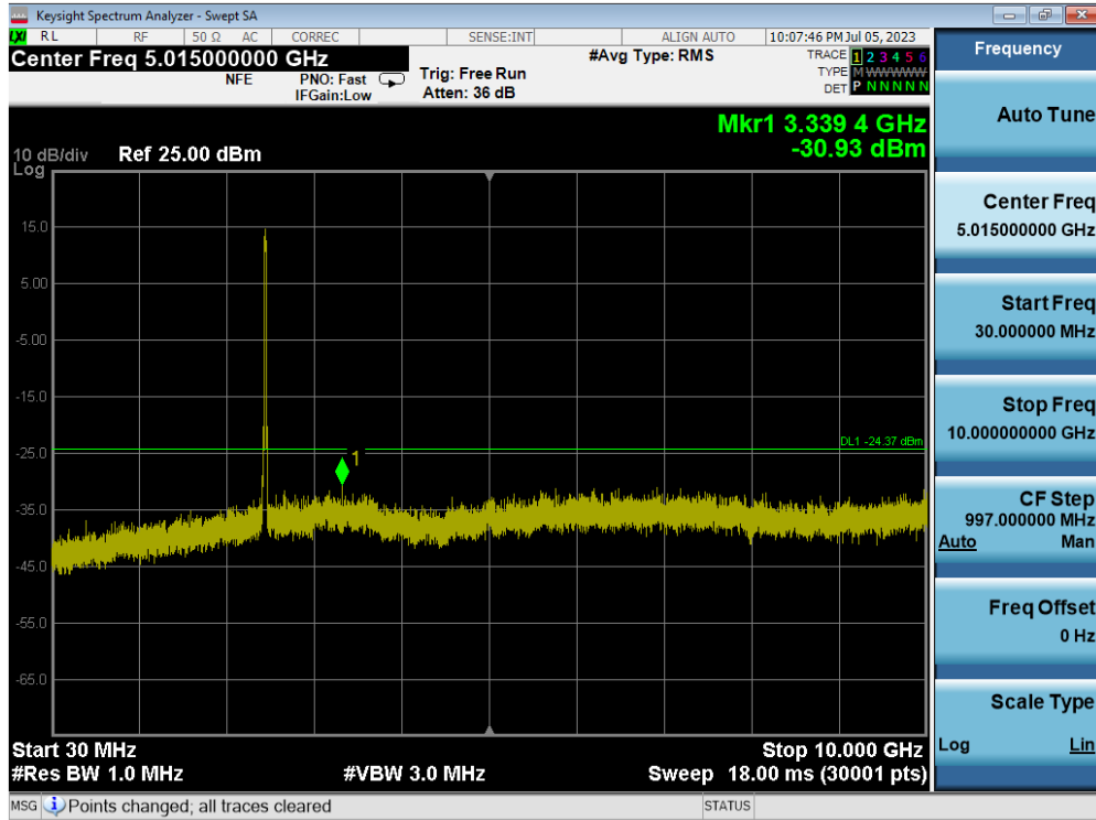
Plot 7-95. Conducted Spurious Plot MIMO ANT2 (802.11ax OFDMA – 242 Tones – Ch. 11) – ANT 2
