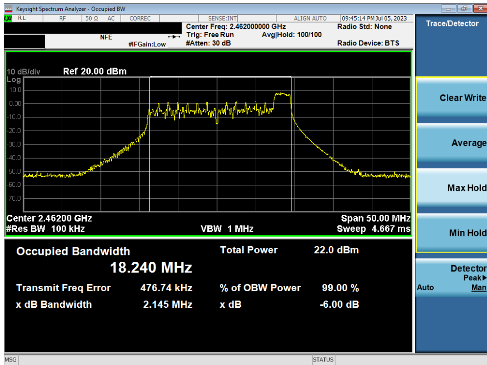
Plot 7-9. 6dB Bandwidth Plot MIMO ANT1 (802.11ax OFDMA – 26 Tones – Ch. 11) – ANT 1
