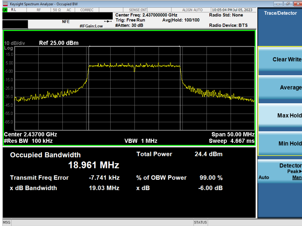
Plot 7-17. 6dB Bandwidth Plot MIMO ANT2 (802.11ax OFDMA – 242 Tones – Ch. 6) – ANT 2
