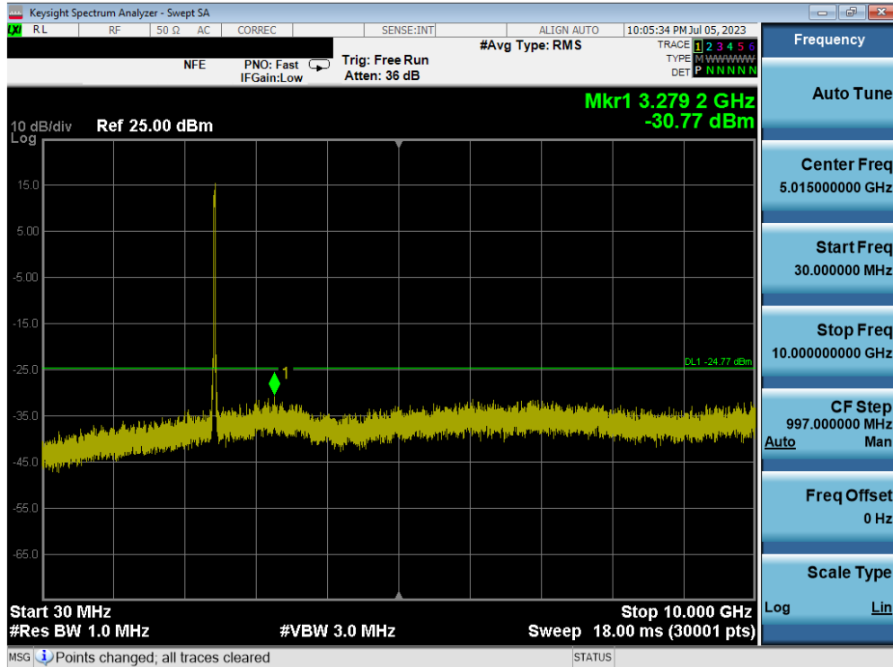
Plot 7-93. Conducted Spurious Plot MIMO ANT2 (802.11ax OFDMA – 242 Tones – Ch. 6) – ANT 2
