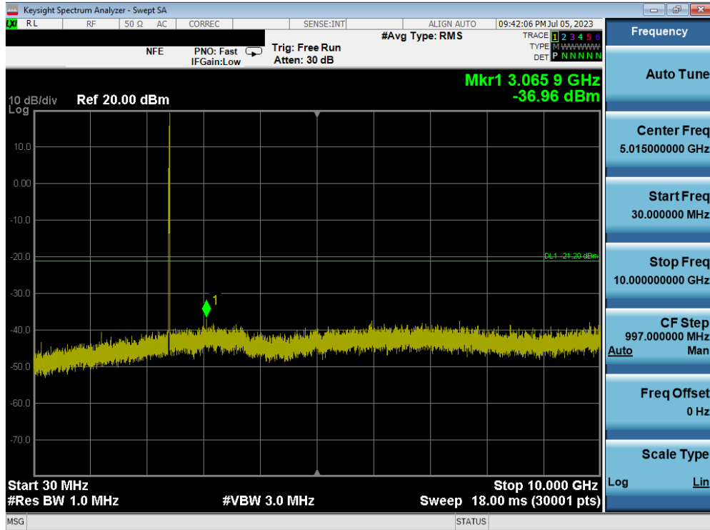
Plot 7-73. Conducted Spurious Plot MIMO ANT1 (802.11ax OFDMA – 26 Tones – Ch. 1) – ANT 1
