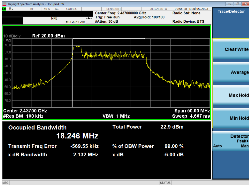
Plot 7-14. 6dB Bandwidth Plot MIMO ANT2 (802.11ax OFDMA – 26 Tones – Ch. 6) – ANT 2
