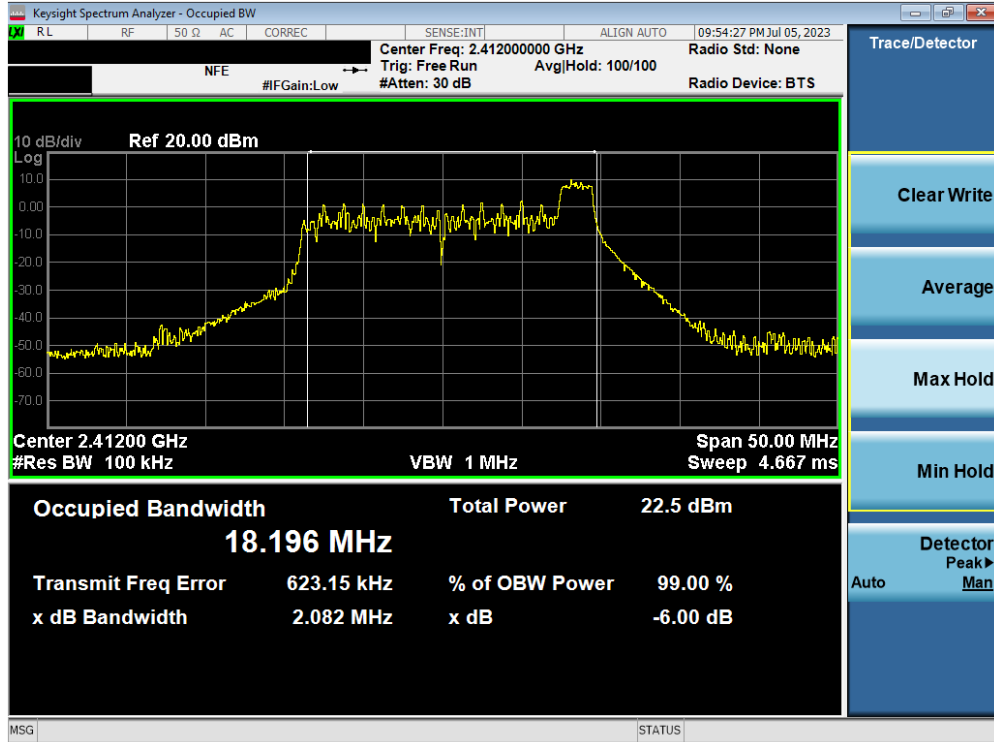
Plot 7-13. 6dB Bandwidth Plot MIMO ANT2 (802.11ax OFDMA – 26 Tones – Ch. 1) – ANT 2
