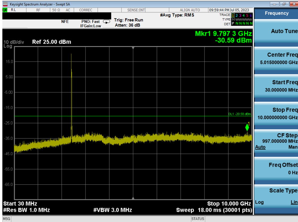
Plot 7-87. Conducted Spurious Plot MIMO ANT2 (802.11ax OFDMA – 26 Tones – Ch. 6) – ANT 2
