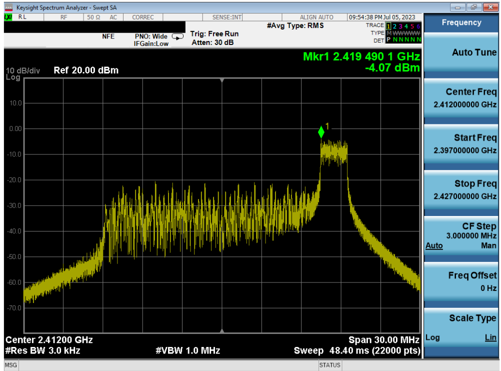
Plot 7-31. Power Spectral Density Plot MIMO ANT2 (802.11ax OFDMA – 26 Tones – Ch. 1) – ANT 2
