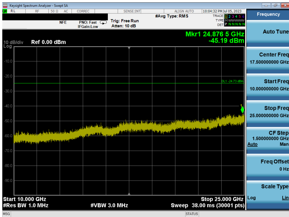
Plot 7-92. Conducted Spurious Plot MIMO ANT2 (802.11ax OFDMA – 242 Tones – Ch. 1) – ANT 2
