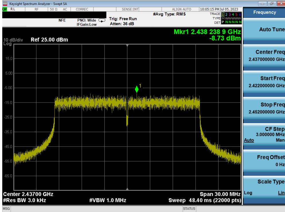
Plot 7-35. Power Spectral Density Plot MIMO ANT2 (802.11ax OFDMA – 242 Tones – Ch. 6) – ANT 2
