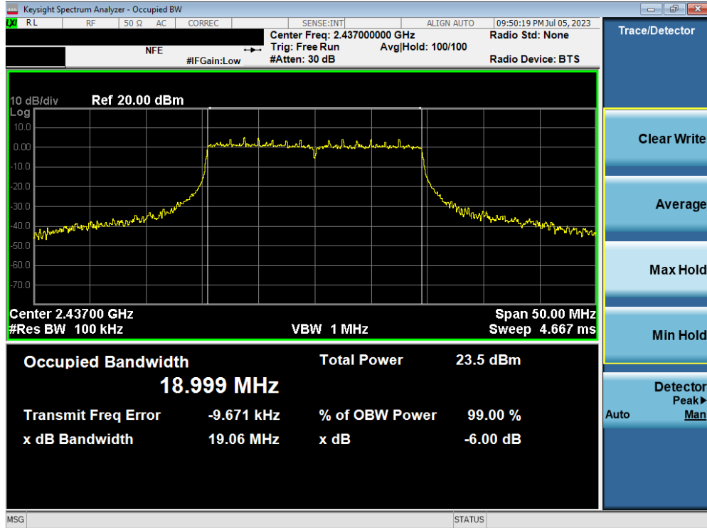
Plot 7-11. 6dB Bandwidth Plot MIMO ANT1 (802.11ax OFDMA – 242 Tones – Ch. 6) – ANT 1
