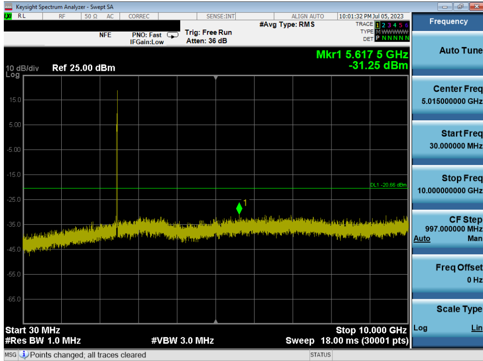
Plot 7-89. Conducted Spurious Plot MIMO ANT2 (802.11ax OFDMA – 26 Tones – Ch. 11) – ANT 2
