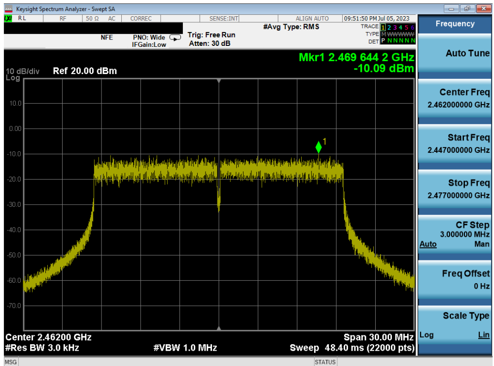
Plot 7-30. Power Spectral Density Plot MIMO ANT1 (802.11ax OFDMA – 242 Tones – Ch. 11) – ANT 1
