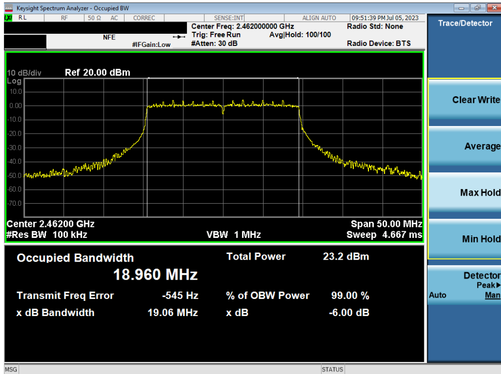
Plot 7-12. 6dB Bandwidth Plot MIMO ANT1 (802.11ax OFDMA – 242 Tones – Ch. 11) – ANT 1
