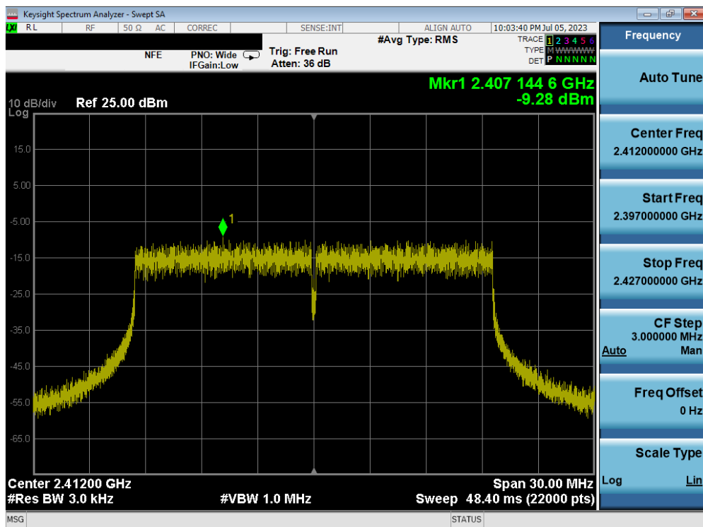
Plot 7-34. Power Spectral Density Plot MIMO ANT2 (802.11ax OFDMA – 242 Tones – Ch. 1) – ANT 2
