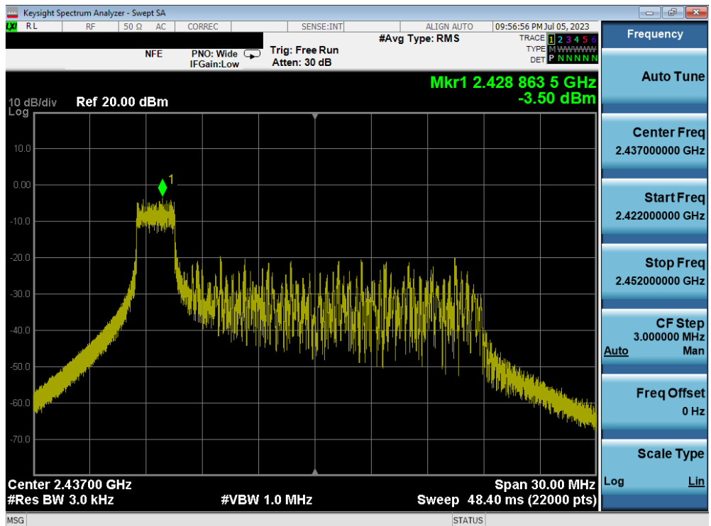
Plot 7-32. Power Spectral Density Plot MIMO ANT2 (802.11ax OFDMA – 26 Tones – Ch. 6) – ANT 2
