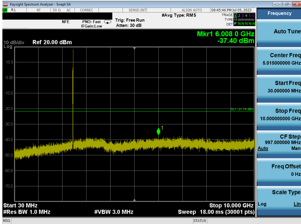
Plot 7-77. Conducted Spurious Plot MIMO ANT1 (802.11ax OFDMA – 26 Tones – Ch. 11) – ANT 1
