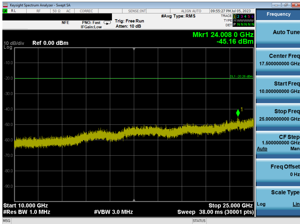
Plot 7-86. Conducted Spurious Plot MIMO ANT2 (802.11ax OFDMA – 26 Tones – Ch. 1) – ANT 2
