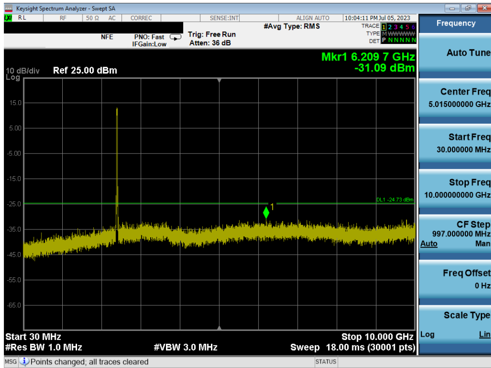
Plot 7-91. Conducted Spurious Plot MIMO ANT2 (802.11ax OFDMA – 242 Tones – Ch. 1) – ANT 2
