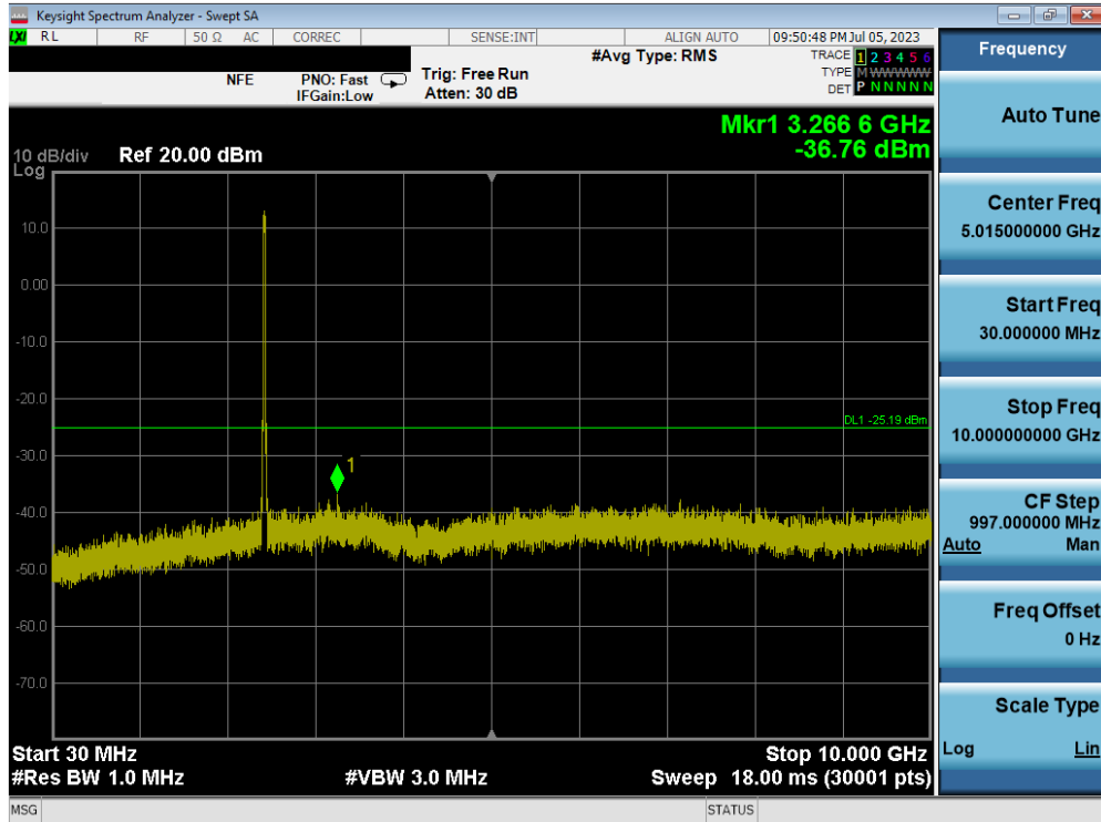
Plot 7-81. Conducted Spurious Plot MIMO ANT1 (802.11ax OFDMA – 242 Tones – Ch. 6) – ANT 1
