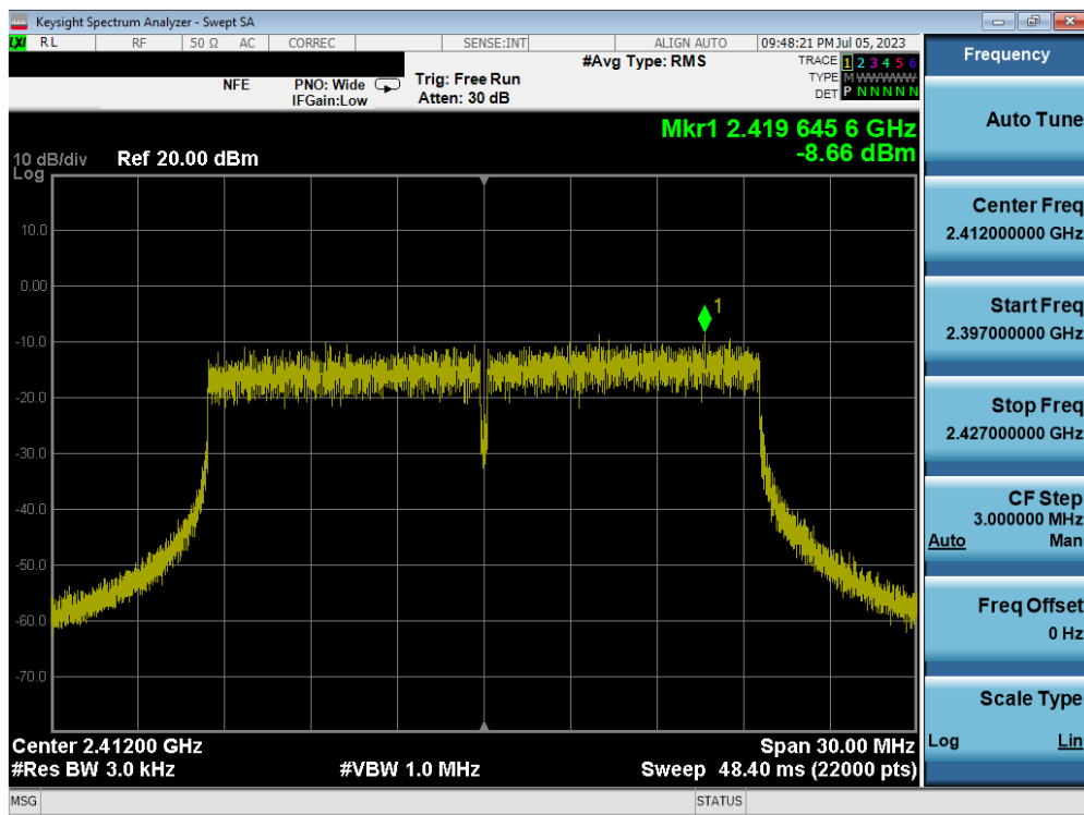
Plot 7-28. Power Spectral Density Plot MIMO ANT1 (802.11ax OFDMA – 242 Tones – Ch. 1) – ANT 1
