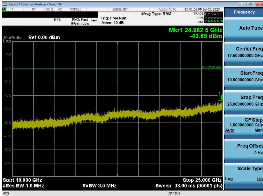
Plot 7-90. Conducted Spurious Plot MIMO ANT2 (802.11ax OFDMA – 26 Tones – Ch. 11) – ANT 2
