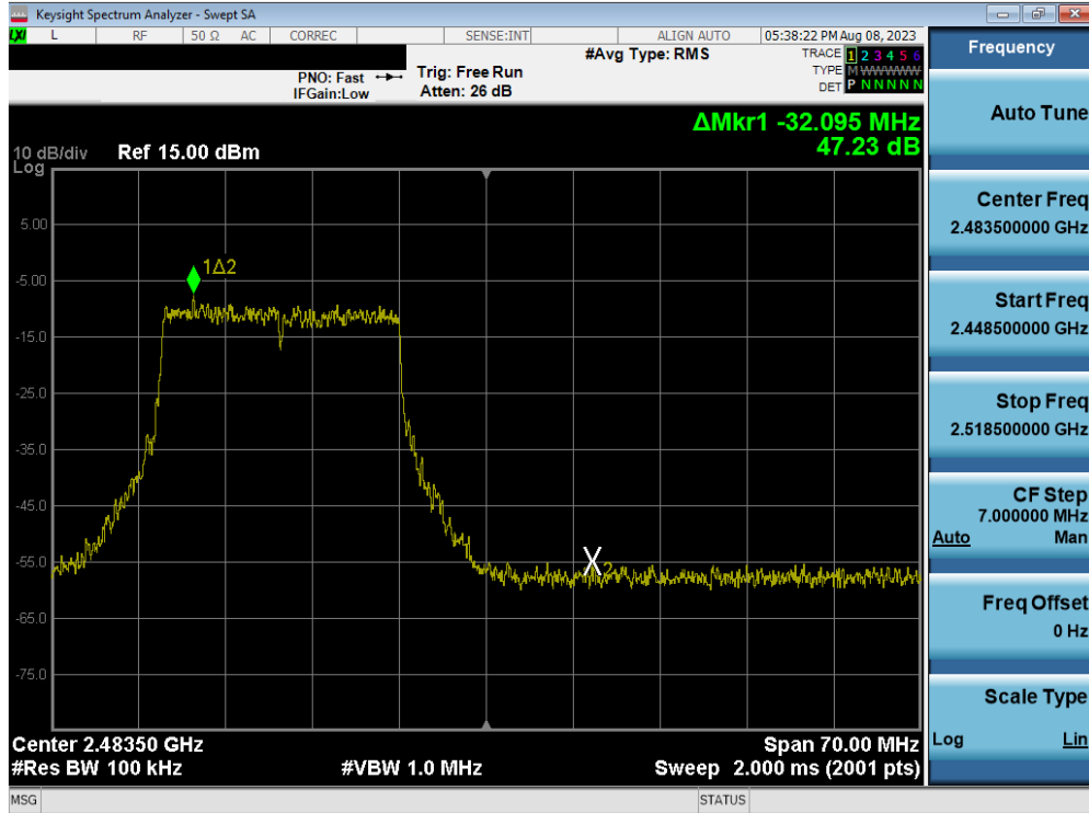
Plot 7-59. Band Edge Plot MIMO ANT2 (802.11ax OFDMA – 242 Tones – Ch. 12) – ANT 2
