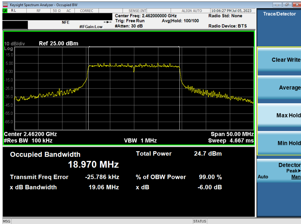
Plot 7-18. 6dB Bandwidth Plot MIMO ANT1 (802.11ax OFDMA – 242 Tones – Ch. 11) – ANT 2
