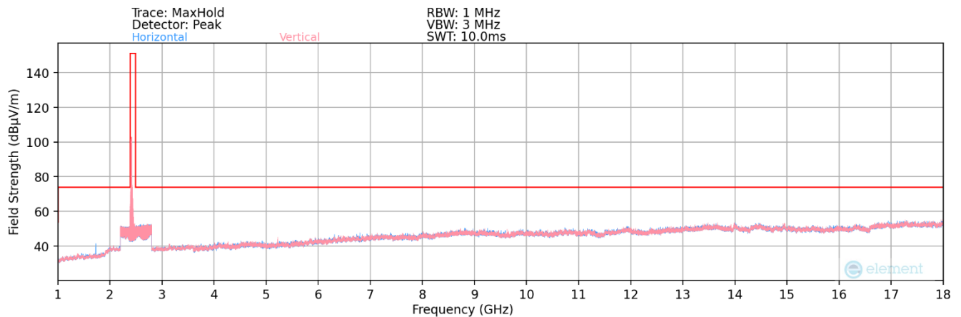
Plot 7-101. Radiated Spurious Plot above 1GHz SISO ANT2 (802.11ax OFDMA – 242 Tones – Ch. 1)
