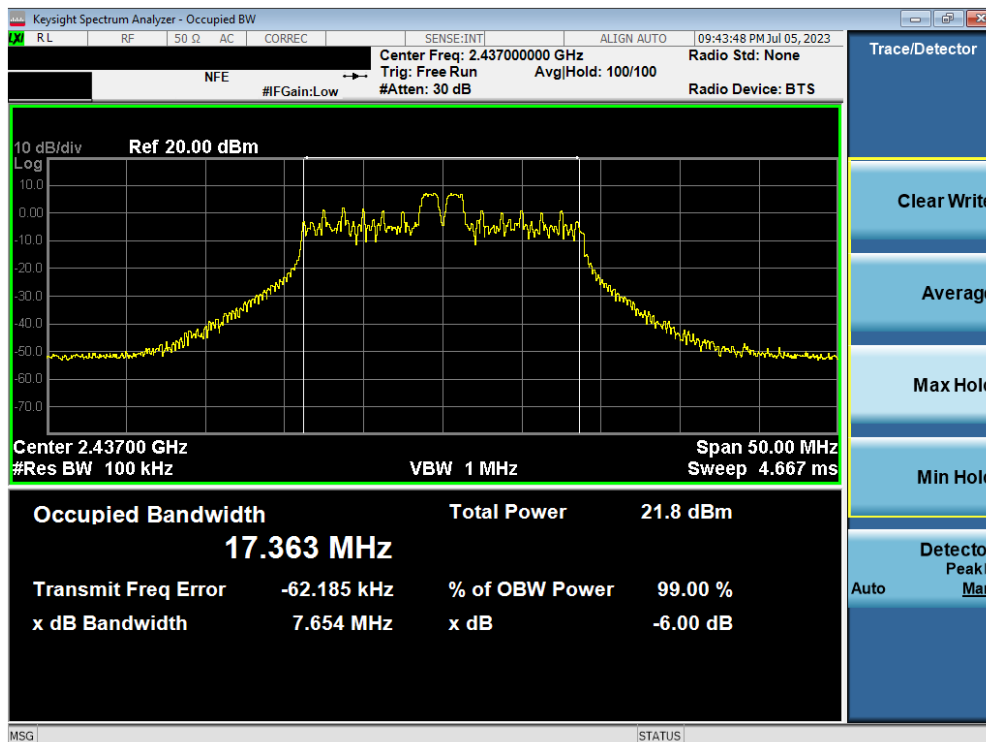
Plot 7-8. 6dB Bandwidth Plot MIMO ANT1 (802.11ax OFDMA – 26 Tones – Ch. 6) – ANT 1
