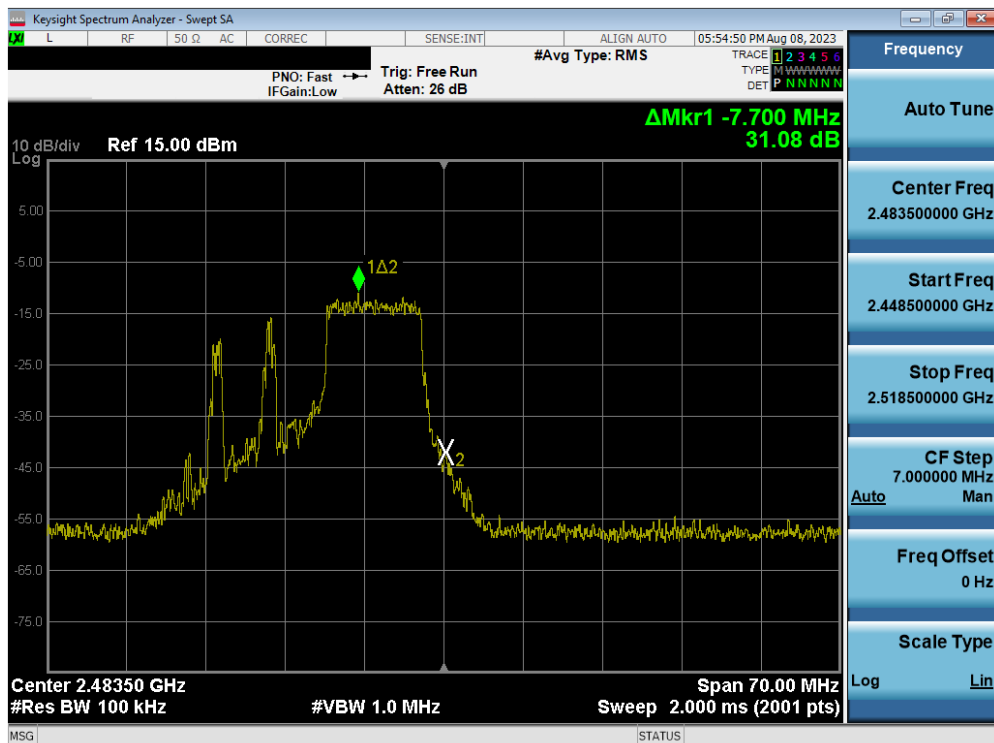
Plot 7-40. Band Edge Plot SISO ANT2 (802.11x OFDMA – 106 Tones – Ch. 13)
