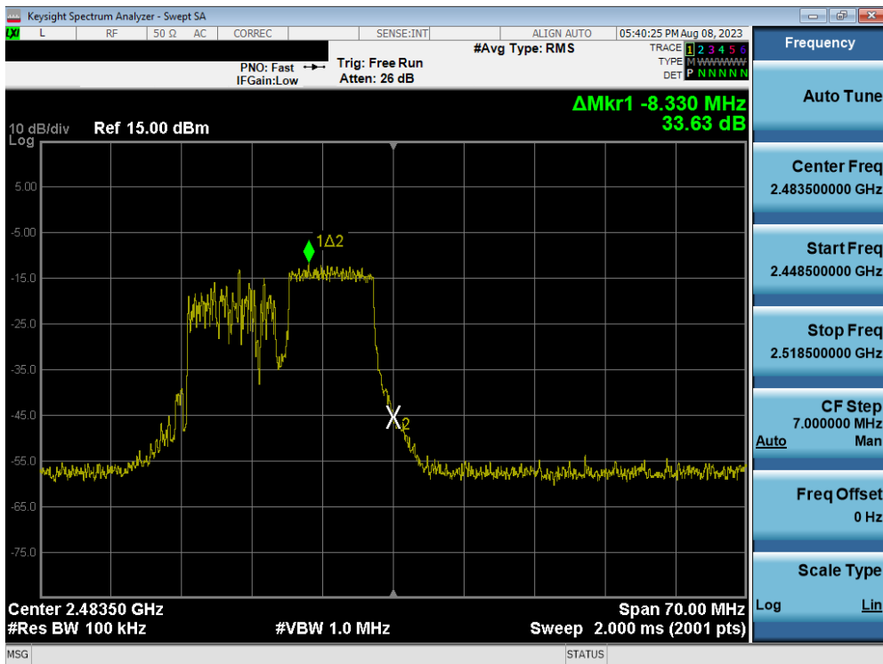
Plot 7-56. Band Edge Plot MIMO ANT2 (802.11ax OFDMA – 106 Tones – Ch. 13) – ANT 2
