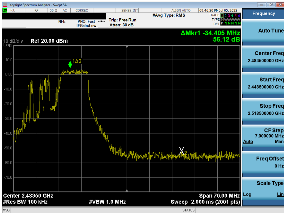
Plot 7-46. Band Edge Plot MIMO ANT1 (802.11ax OFDMA – 106 Tones – Ch. 11) – ANT 1
