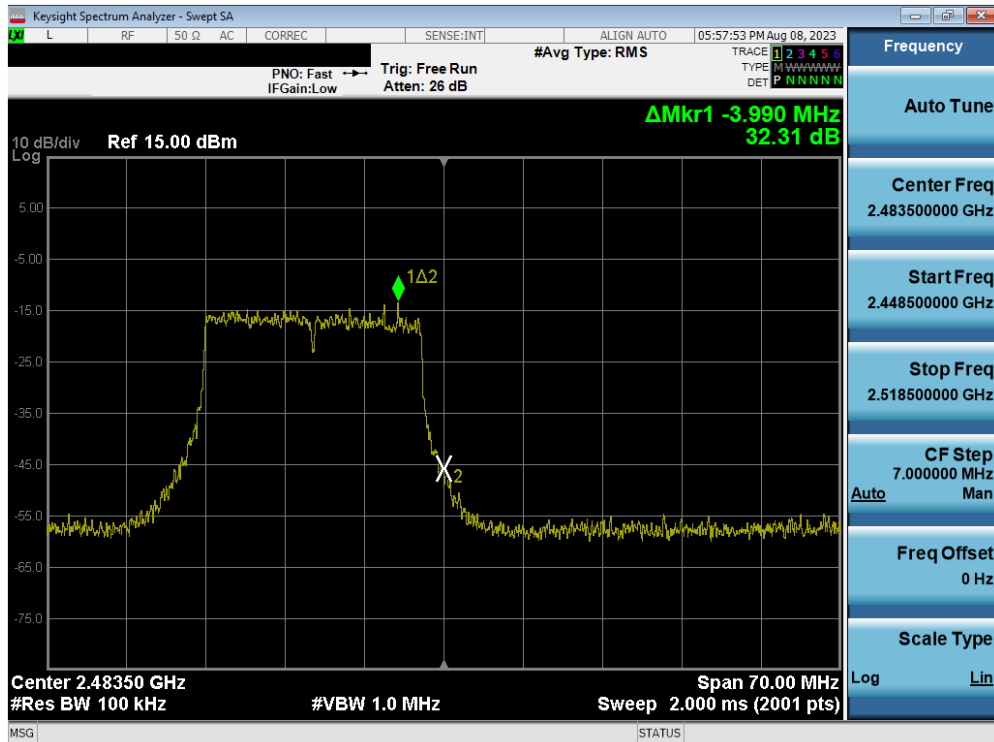
Plot 7-52. Band Edge Plot MIMO ANT1 (802.11ax OFDMA – 242 Tones – Ch. 13) – ANT 1
