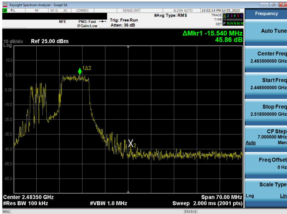
Plot 7-54. Band Edge Plot MIMO ANT2 (802.11ax OFDMA – 106 Tones – Ch. 11) – ANT 2
