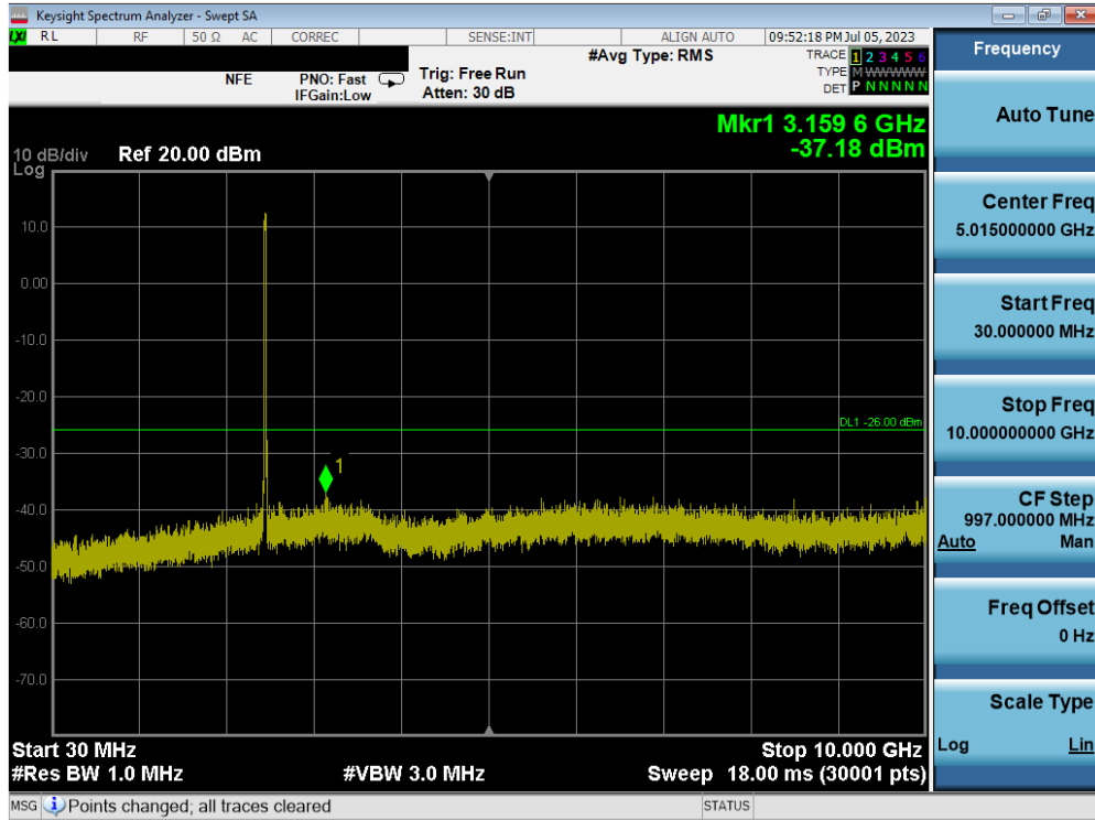
Plot 7-83. Conducted Spurious Plot MIMO ANT1 (802.11ax OFDMA – 242 Tones – Ch. 11) – ANT 1
