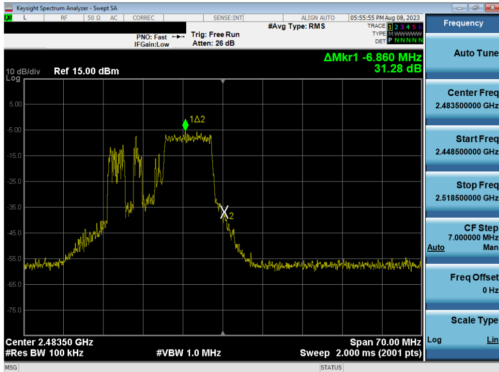
Plot 7-39. Band Edge Plot SISO ANT2 (802.11x OFDMA – 106 Tones – Ch. 12)
