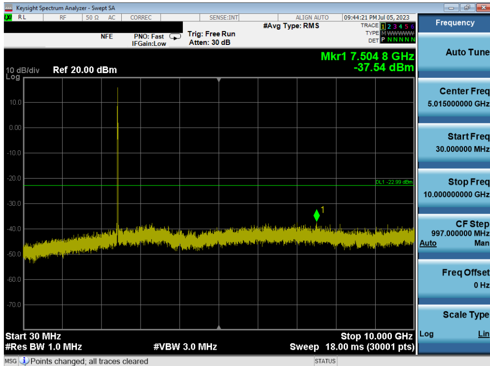
Plot 7-75. Conducted Spurious Plot MIMO ANT1 (802.11ax OFDMA – 26 Tones – Ch. 6) – ANT 1
