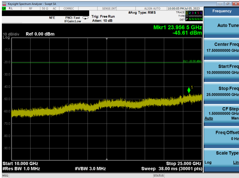
Plot 7-88. Conducted Spurious Plot MIMO ANT2 (802.11ax OFDMA – 26 Tones – Ch. 6) – ANT 2
