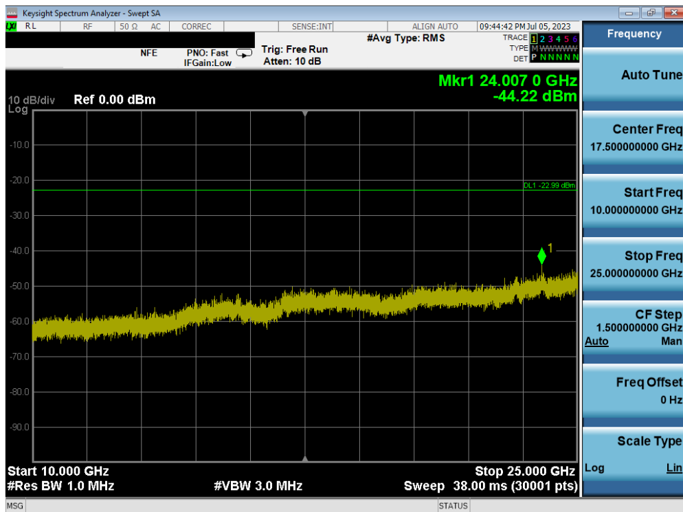
Plot 7-76. Conducted Spurious Plot MIMO ANT1 (802.11ax OFDMA – 26 Tones – Ch. 6) – ANT 1
