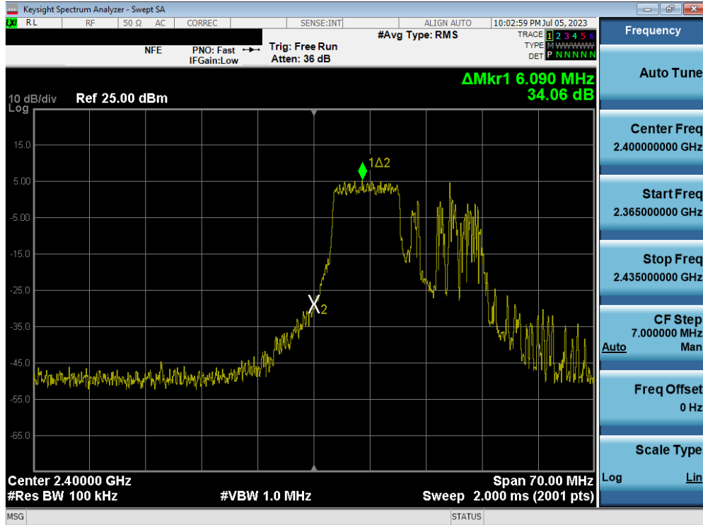
Plot 7-53. Band Edge Plot MIMO ANT2 (802.11ax OFDMA – 106 Tones – Ch. 1) – ANT 2
