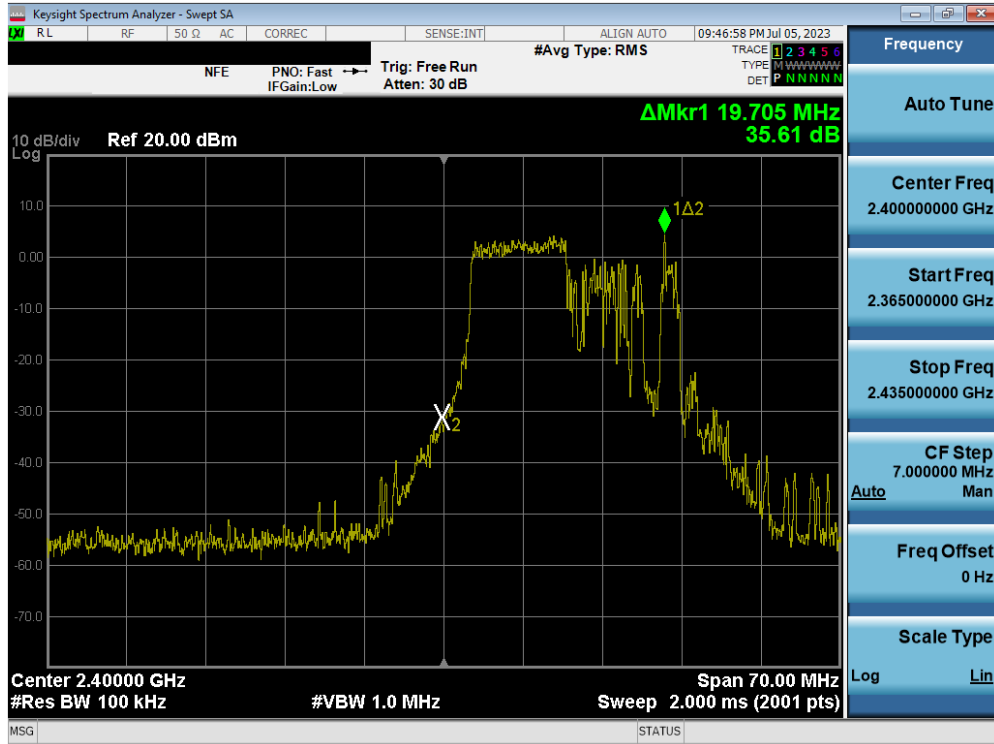
Plot 7-45. Band Edge Plot MIMO ANT1 (802.11ax OFDMA – 106 Tones – Ch. 1) – ANT 1
