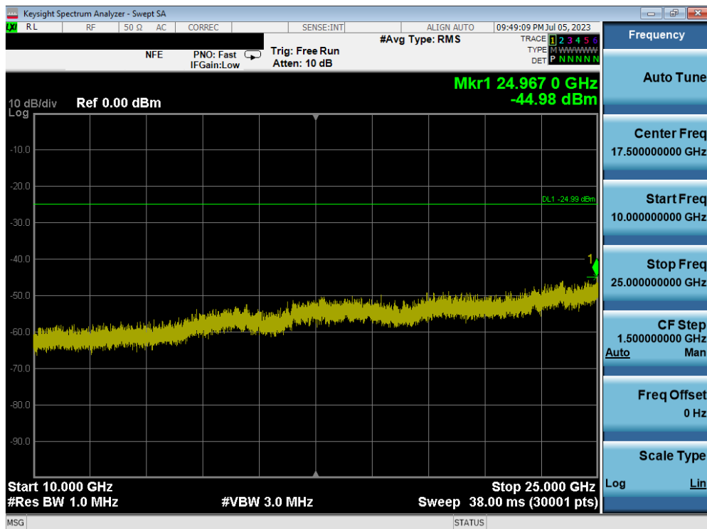
Plot 7-80. Conducted Spurious Plot MIMO ANT1 (802.11ax OFDMA – 242 Tones – Ch. 1) – ANT 1
