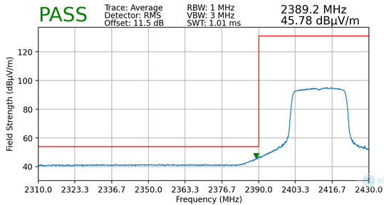
Plot 7-156. Radiated Restricted Lower Band Edge Measurement SISO ANT2 (Average)
