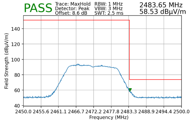
Plot 7-171. Radiated Restricted Upper Band Edge Measurement MIMO (Peak)
