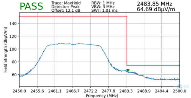
Plot 7-169. Radiated Restricted Upper Band Edge Measurement MIMO (Peak)
