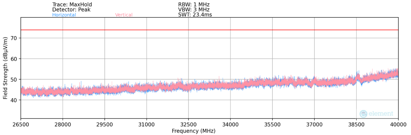
Plot 7-155. Radiated Spurious Plot above 26.5GHz (2.4GHz –6GHz)
