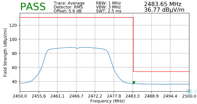
Plot 7-168. Radiated Restricted Upper Band Edge Measurement MIMO (Average)
