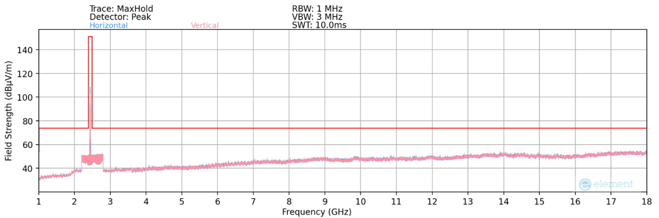
Plot 7-144. Radiated Spurious Plot above 1GHz MIMO (802.11b – Ch. 1)
