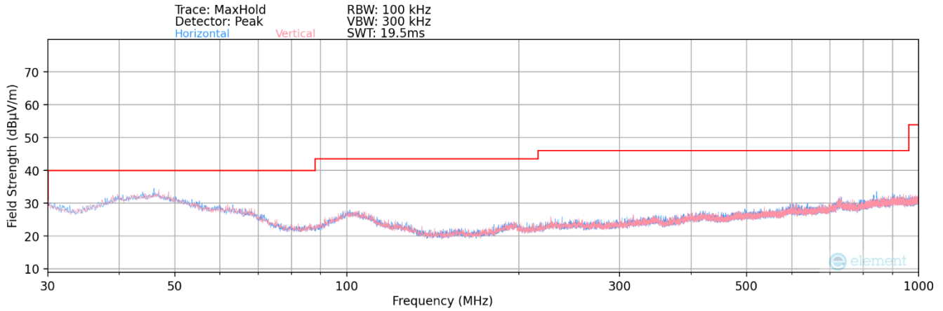
Plot 7-148. Radiated Spurious Plot below 1GHz (2.4GHz – 5GHz)
