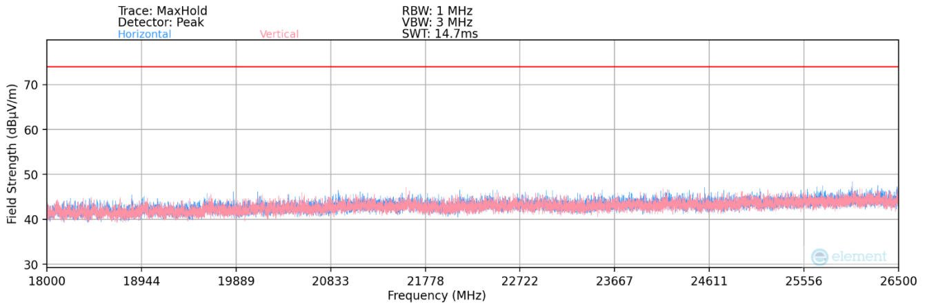
Plot 7-154. Radiated Spurious Plot 18GHz – 26.5GHz (2.4GHz –6GHz)
