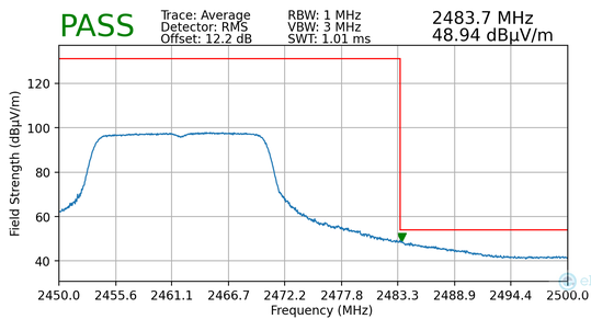
Plot 7-158. Radiated Restricted Upper Band Edge Measurement SISO ANT2 (Average)
