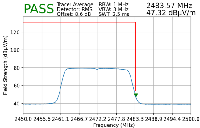
Plot 7-162. Radiated Restricted Upper Band Edge Measurement SISO ANT2 (Average)
