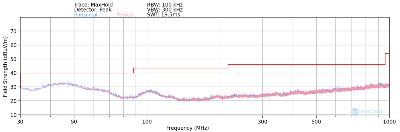
Plot 7-152. Radiated Spurious Plot below 1GHz (2.4GHz -6GHz)
