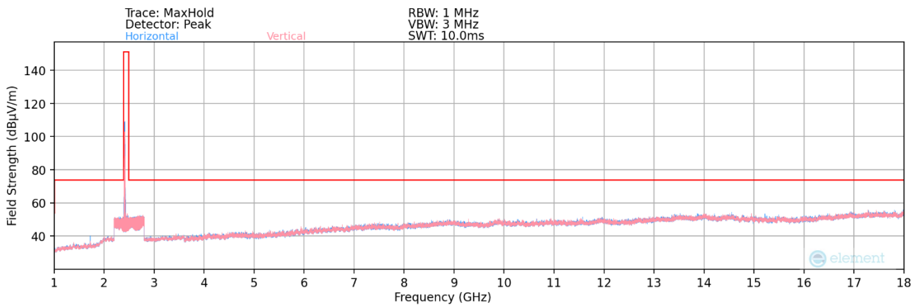
Plot 7-145. Radiated Spurious Plot above 1GHz MIMO (802.11b – Ch. 6)
