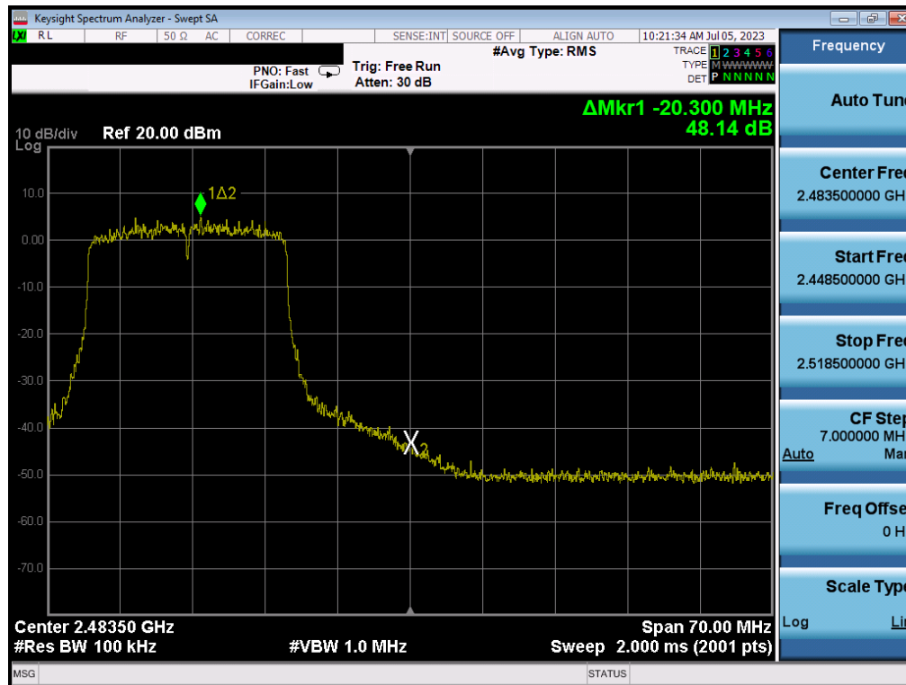
Plot 7-102. Band Edge Plot MIMO ANT1 (802.11ax (2.4GHz) – Ch. 11)
