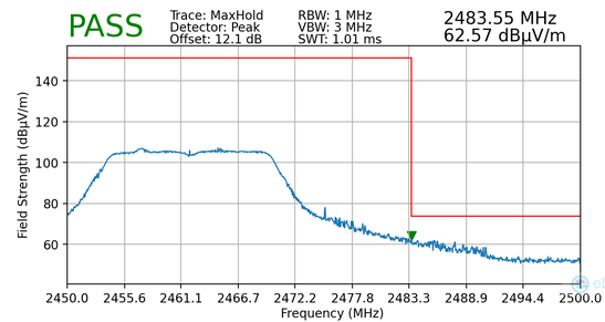
Plot 7-159. Radiated Restricted Upper Band Edge Measurement SISO ANT2 (Peak)
