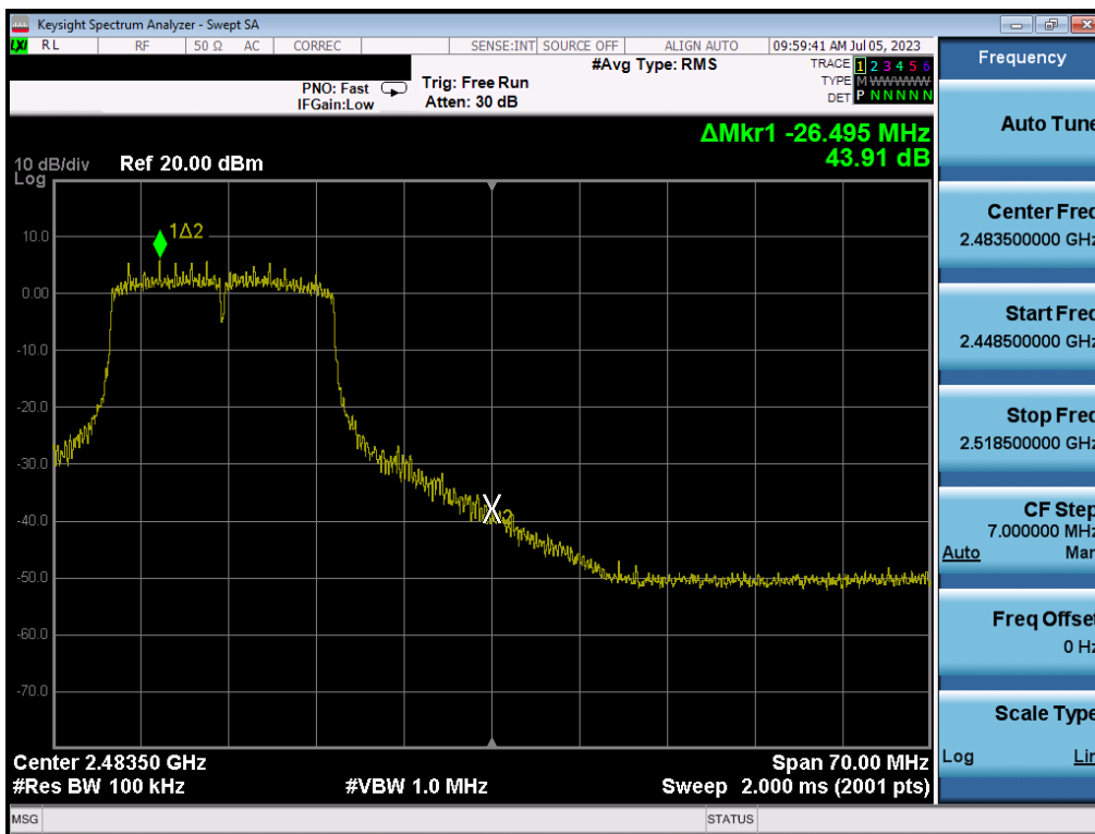
Plot 7-114. Band Edge Plot MIMO ANT2 (802.11n (2.4GHz) – Ch. 11)
