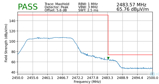
Plot 7-167. Radiated Restricted Upper Band Edge Measurement MIMO (Peak)
