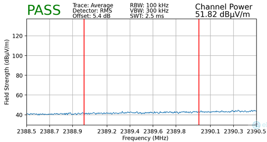
Plot 7-164. Radiated Restricted Lower Band Edge Measurement MIMO (Average)
