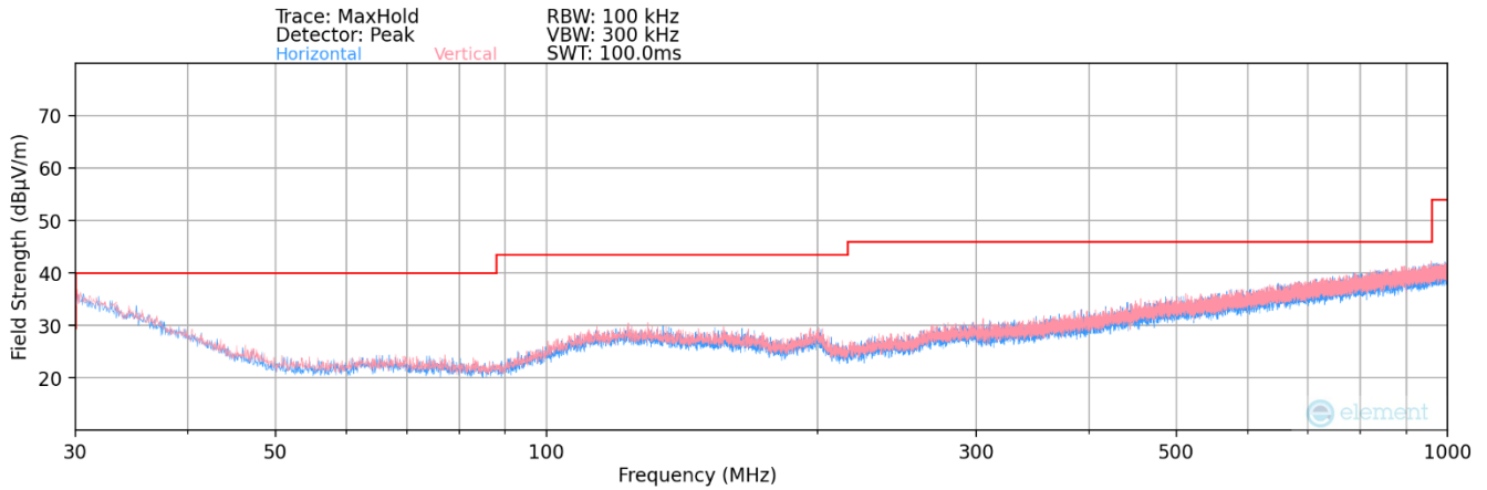
Plot 7-143. Radiated Spurious Plot below 1GHz MIMO
