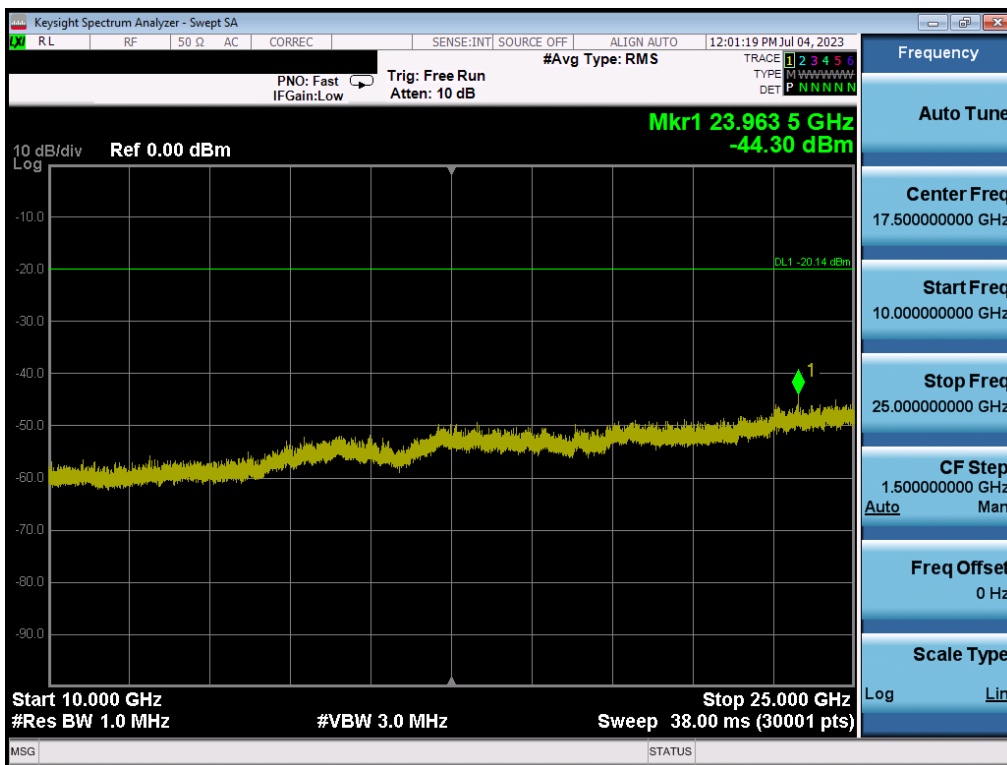
Plot 7-124. Conducted Spurious Plot SISO ANT2 (802.11b – Ch. 6)
