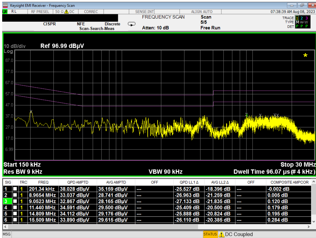
Plot 7-172. Line Conducted Plot with 802.11b (L1)
