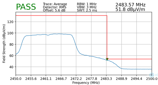
Plot 7-166. Radiated Restricted Upper Band Edge Measurement MIMO (Average)
