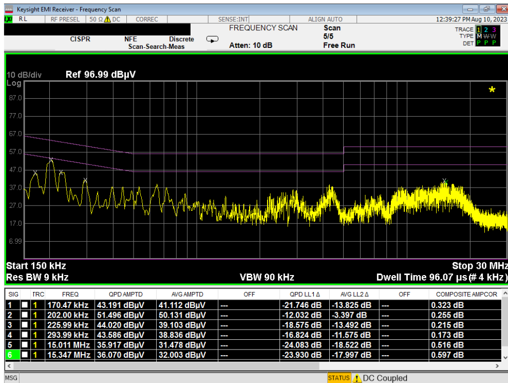
Plot 7-173. Line Conducted Plot with 802.11b (N)
