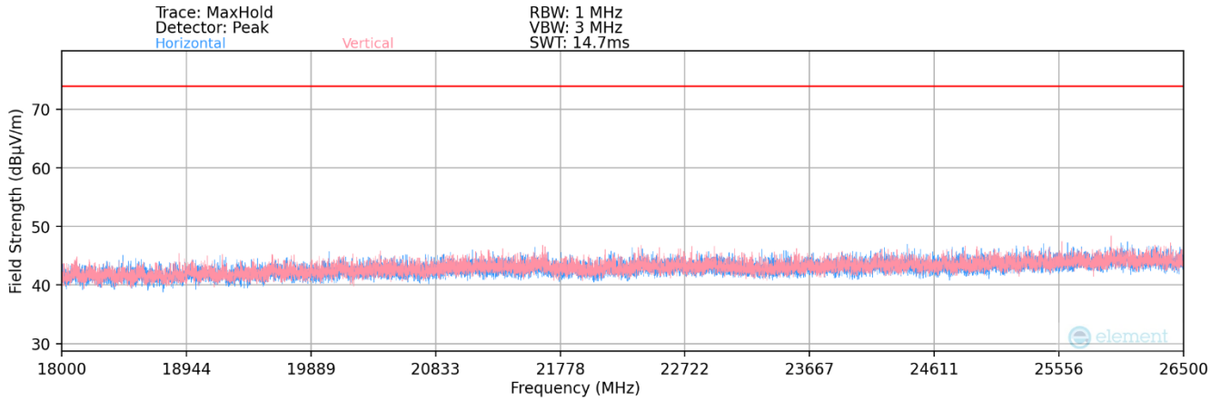
Plot 7-150. Radiated Spurious Plot 18GHz – 26.5GHz (2.4GHz – 5GHz)
