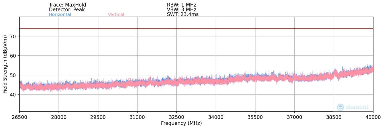
Plot 7-151. Radiated Spurious Plot above 26.5GHz (2.4GHz – 5GHz)
