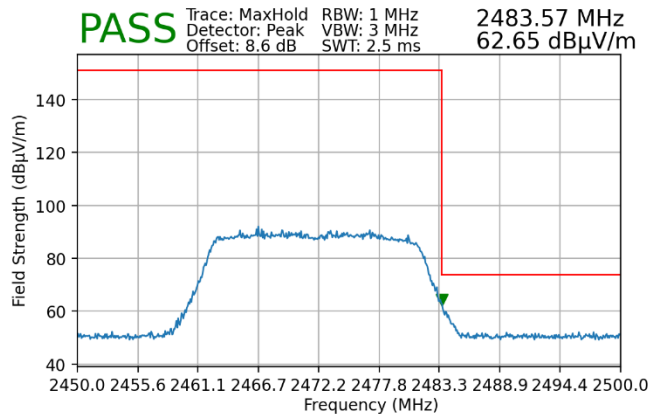
Plot 7-163. Radiated Restricted Upper Band Edge Measurement SISO ANT2 (Peak)
