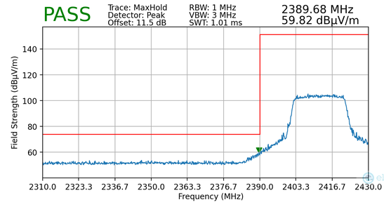
Plot 7-157. Radiated Restricted Lower Band Edge Measurement SISO ANT2 (Peak)
