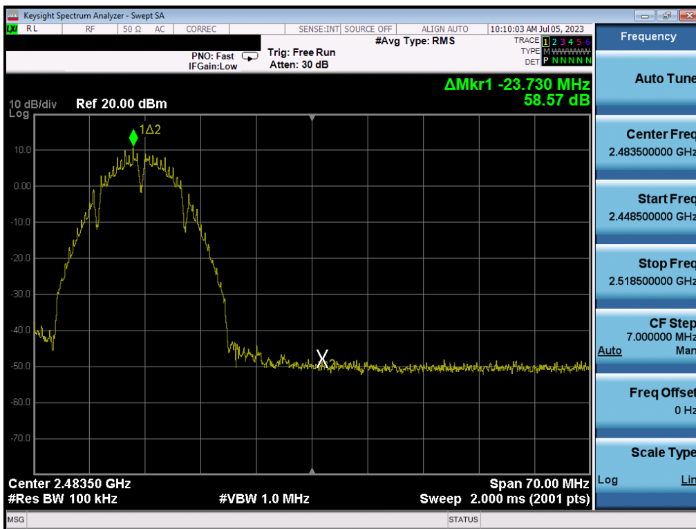
Plot 7-106. Band Edge Plot MIMO ANT2 (802.11b – Ch. 11)
