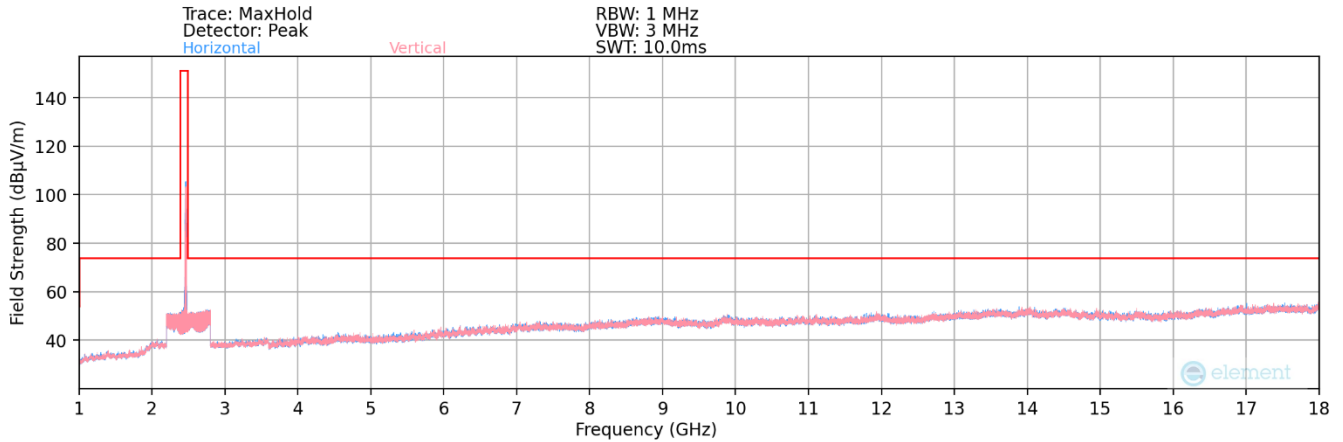
Plot 7-146. Radiated Spurious Plot above 1GHz MIMO (802.11b – Ch. 11)
