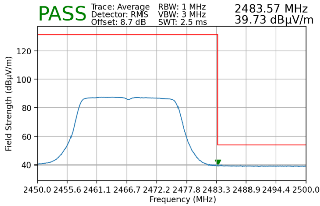
Plot 7-160. Radiated Restricted Upper Band Edge Measurement SISO ANT2 (Average)
