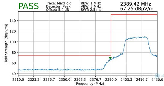
Plot 7-165. Radiated Restricted Lower Band Edge Measurement MIMO (Peak)
