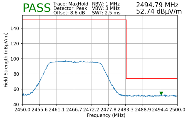
Plot 7-161. Radiated Restricted Upper Band Edge Measurement SISO ANT2 (Peak)
