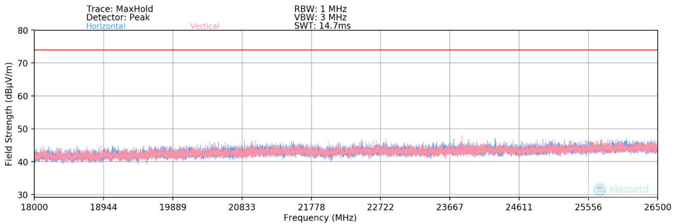
Plot 7-147. Radiated Spurious Plot above 18GHz MIMO
