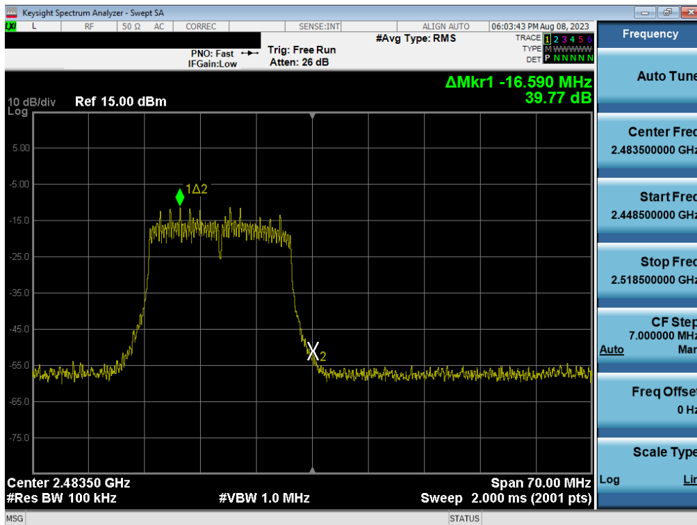
Plot 7-100. Band Edge Plot MIMO ANT1 (802.11n (2.4GHz) – Ch. 13)
