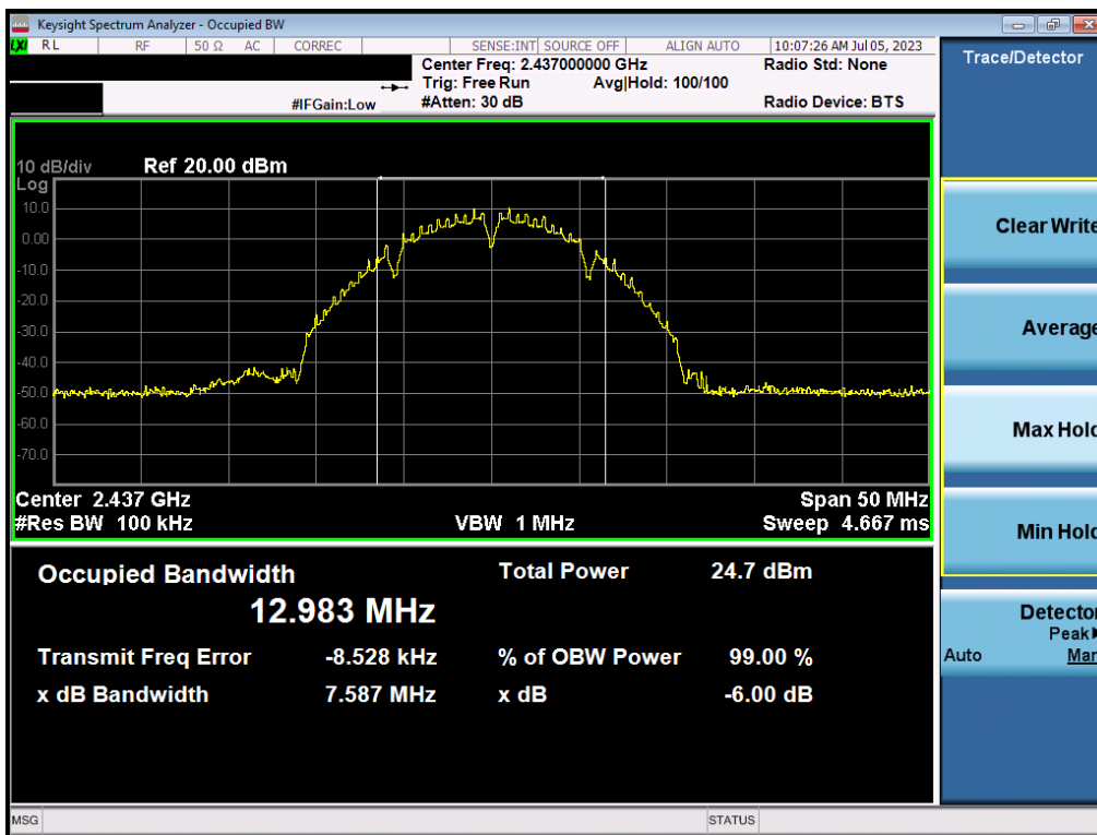
Plot 7-26. 6dB Bandwidth Plot MIMO ANT2 (802.11b – Ch. 6)
