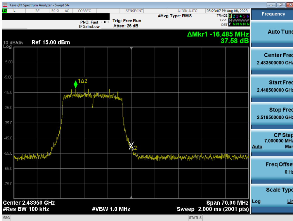
Plot 7-84. Band Edge Plot SISO ANT2 (802.11n (2.4GHz) – Ch. 13)
