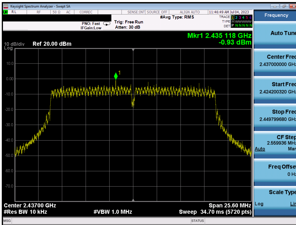
Plot 7-44. Power Spectral Density Plot SISO ANT2 (802.11n (2.4GHz) – Ch. 6)
