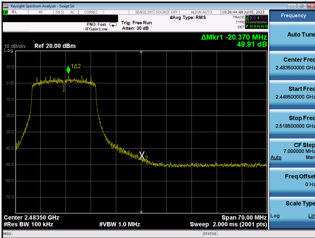
Plot 7-98. Band Edge Plot MIMO ANT1 (802.11n (2.4GHz) – Ch. 11)
