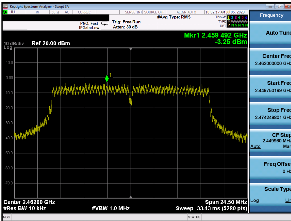
Plot 7-66. Power Spectral Density Plot MIMO ANT2 (802.11g – Ch. 11)
