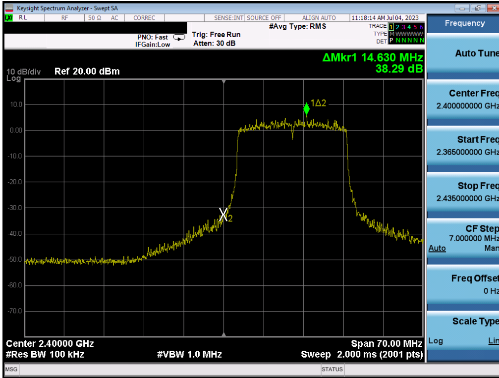
Plot 7-85. Band Edge Plot SISO ANT2 (802.11ax (2.4GHz) – Ch. 1)
