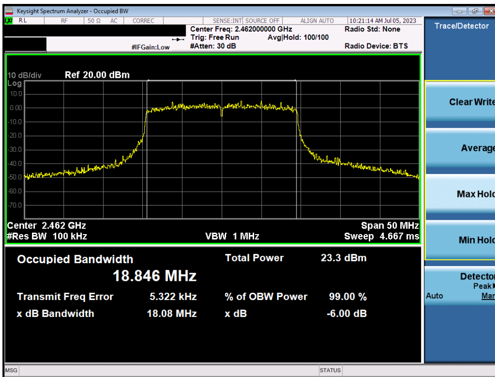
Plot 7-24. 6dB Bandwidth Plot MIMO ANT1 (802.11ax (2.4GHz) – Ch. 11)
