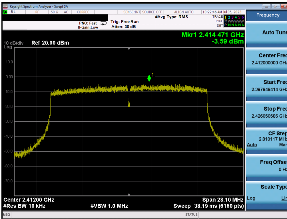
Plot 7-58. Power Spectral Density Plot MIMO ANT1 (802.11ax (2.4GHz) – Ch. 1)
