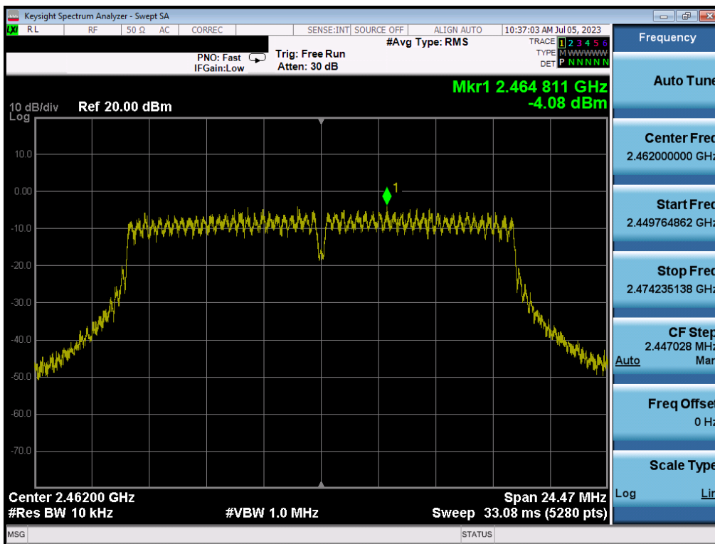
Plot 7-54. Power Spectral Density Plot MIMO ANT1 (802.11g – Ch. 11)
