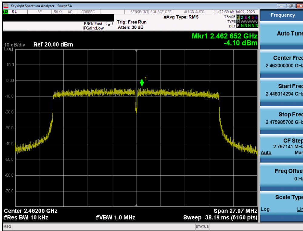
Plot 7-48. Power Spectral Density Plot SISO ANT2 (802.11ax (2.4GHz) – Ch. 11)
