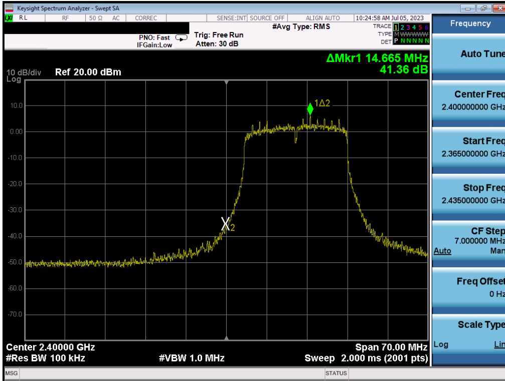
Plot 7-97. Band Edge Plot MIMO ANT1 (802.11n (2.4GHz) – Ch. 1)
