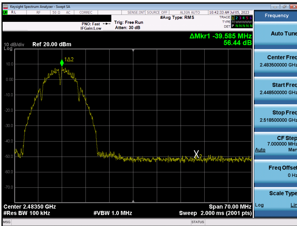
Plot 7-90. Band Edge Plot MIMO ANT1 (802.11b – Ch. 11)
