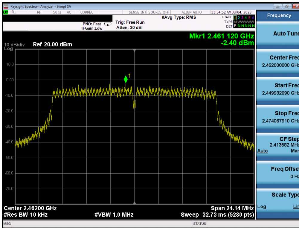
Plot 7-42. Power Spectral Density Plot SISO ANT2 (802.11g – Ch. 11)
