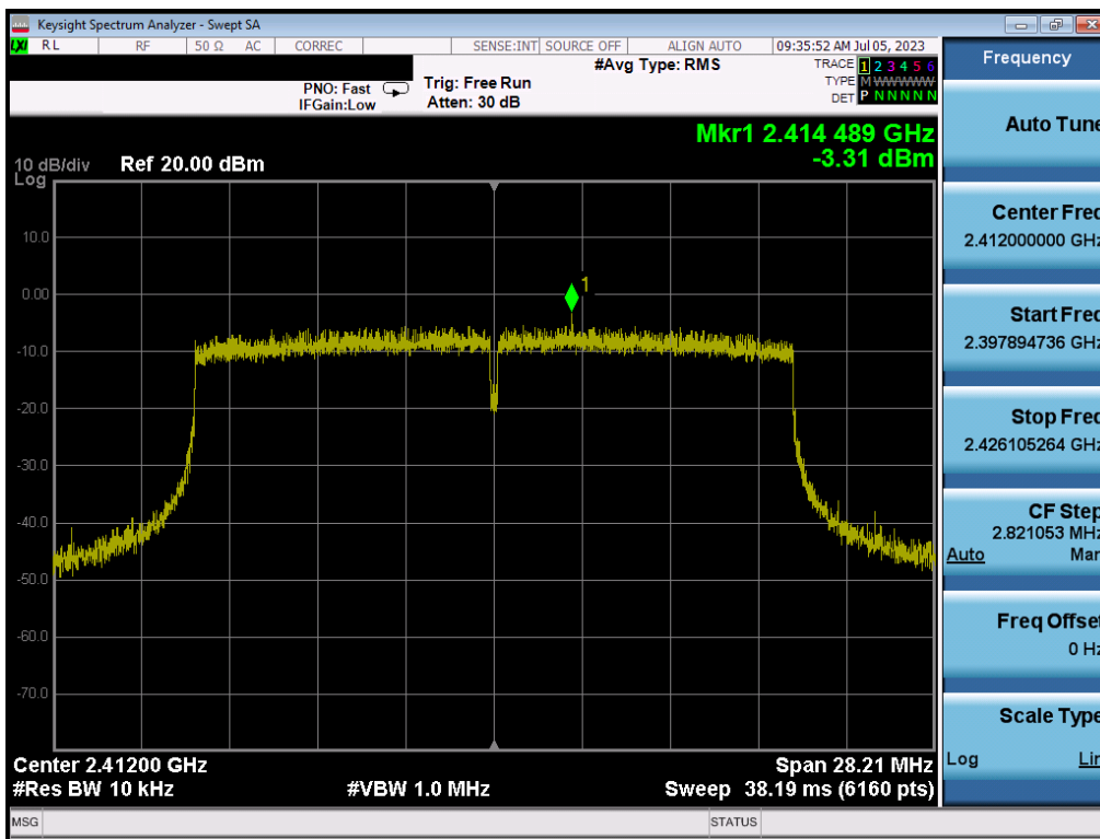
Plot 7-70. Power Spectral Density Plot MIMO ANT2 (802.11ax (2.4GHz) – Ch. 1)
