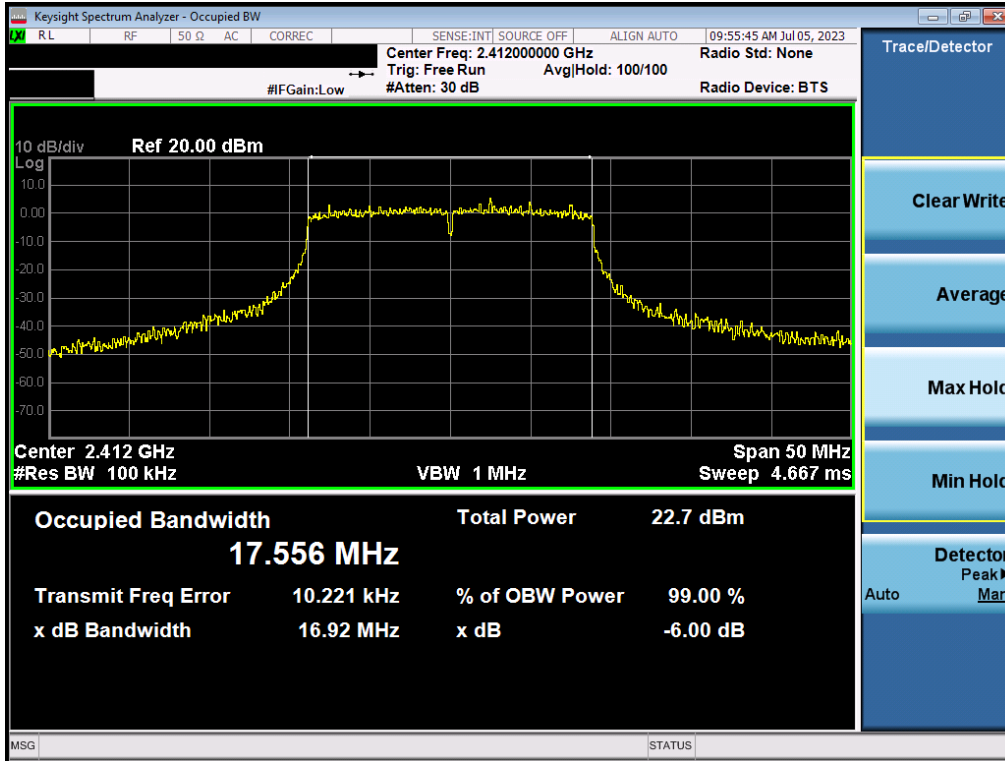
Plot 7-31. 6dB Bandwidth Plot MIMO ANT2 (802.1n (2.4GHz) – Ch. 1)
