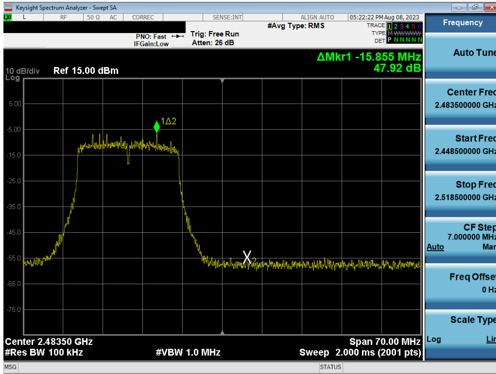
Plot 7-83. Band Edge Plot SISO ANT2 (802.11n (2.4GHz) – Ch. 12)
