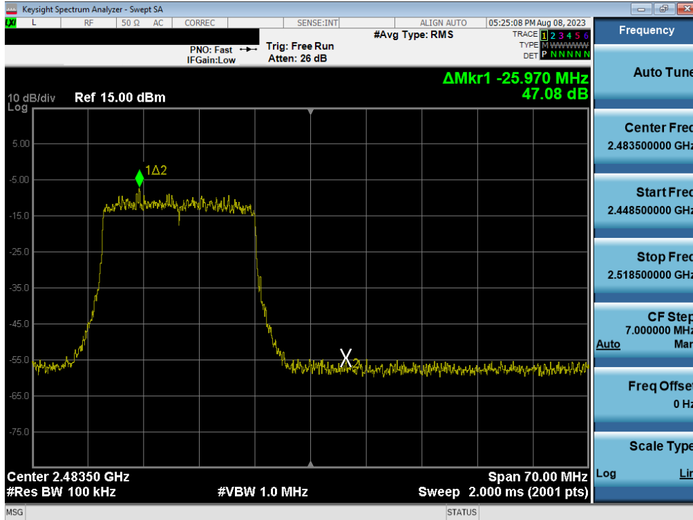
Plot 7-87. Band Edge Plot SISO ANT2 (802.11ax (2.4GHz) – Ch. 12)
