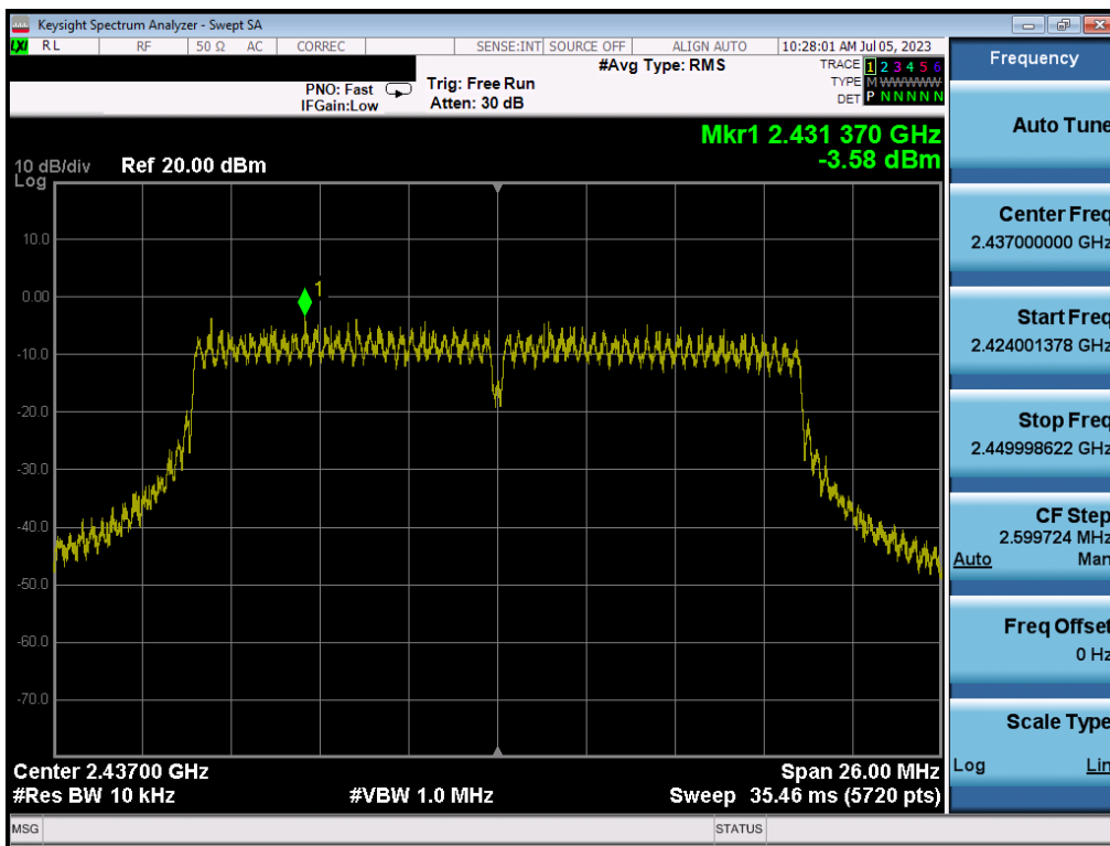
Plot 7-56. Power Spectral Density Plot MIMO ANT1 (802.11n (2.4GHz) – Ch. 6)
