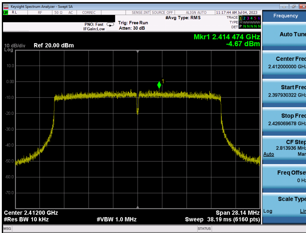
Plot 7-46. Power Spectral Density Plot SISO ANT2 (802.11ax (2.4GHz) – Ch. 1)
