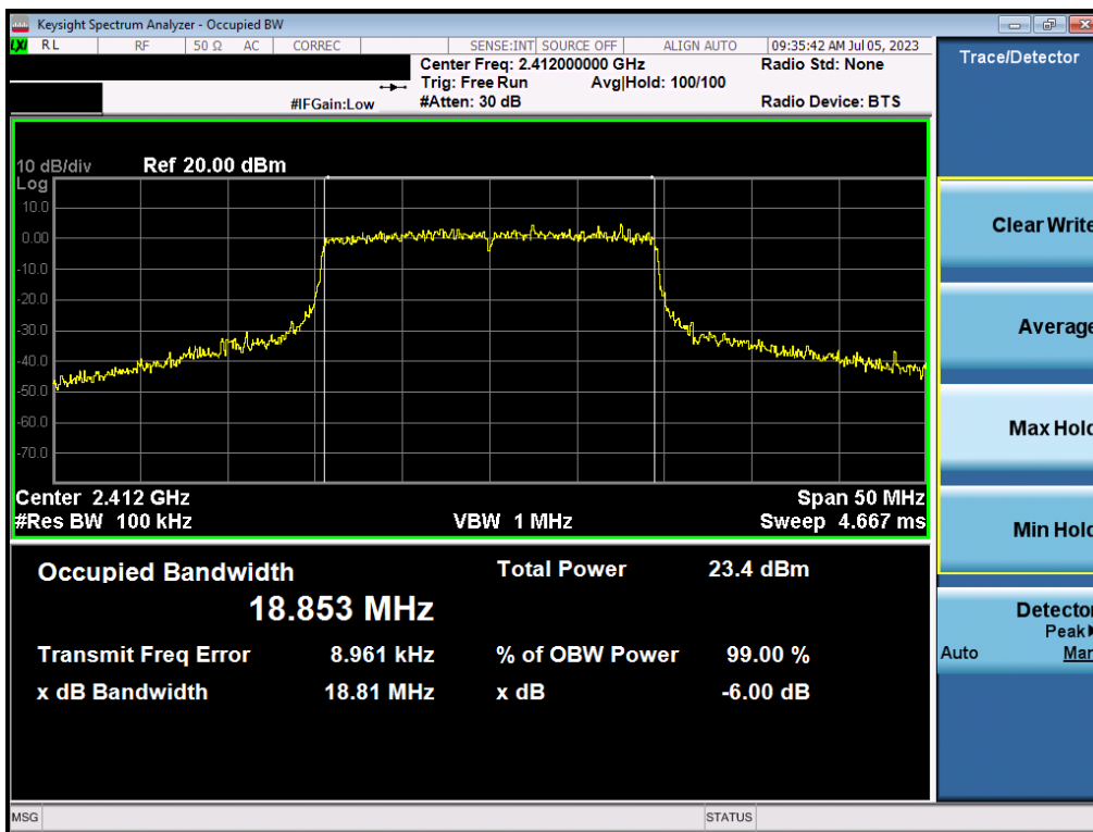
Plot 7-34. 6dB Bandwidth Plot MIMO ANT2 (802.1ax (2.4GHz) – Ch. 1)
