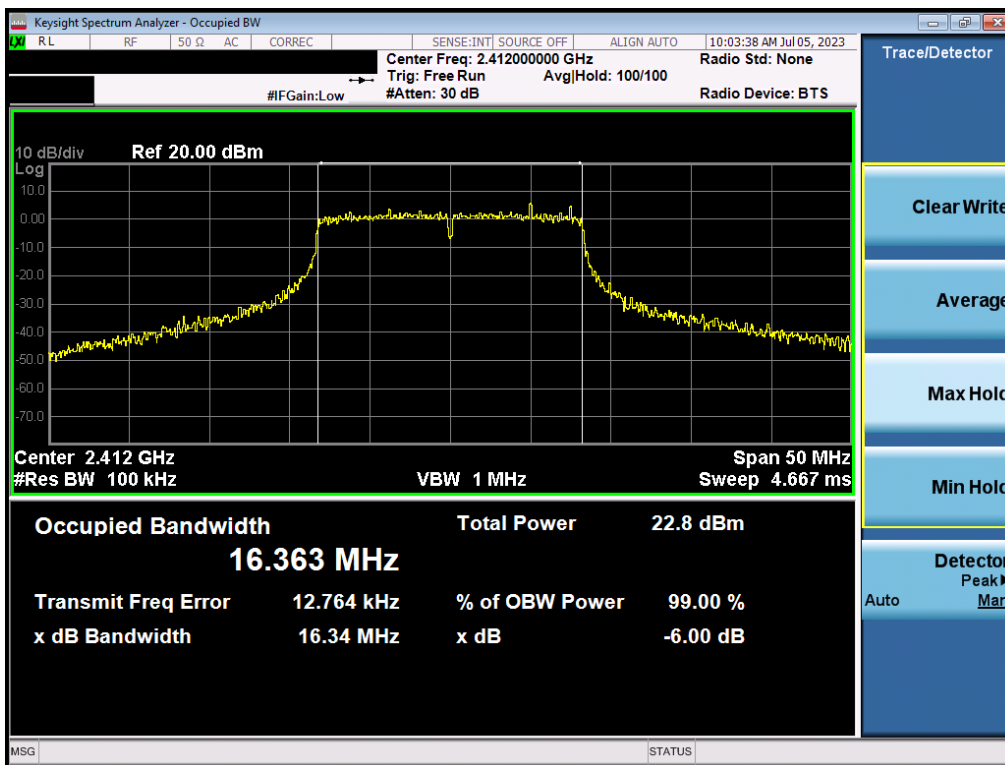
Plot 7-28. 6dB Bandwidth Plot MIMO ANT2 (802.1g – Ch. 1)
