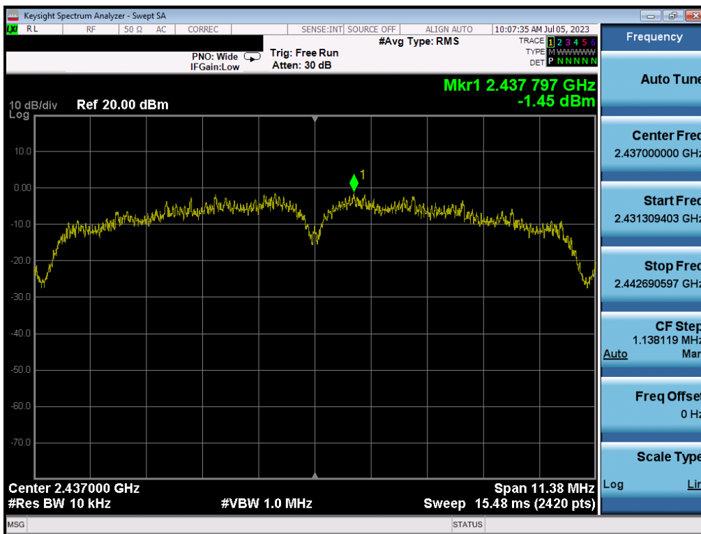
Plot 7-62. Power Spectral Density Plot MIMO ANT2 (802.11b – Ch. 6)
