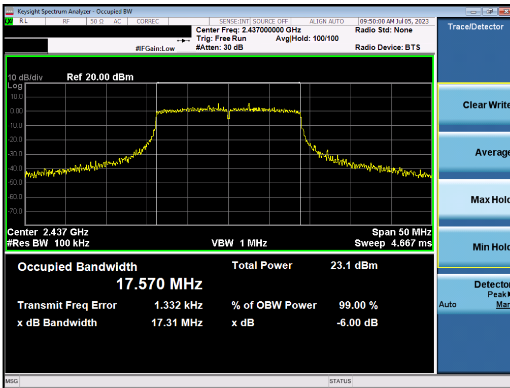
Plot 7-32. 6dB Bandwidth Plot MIMO ANT2 (802.11n (2.4GHz) – Ch. 6)
