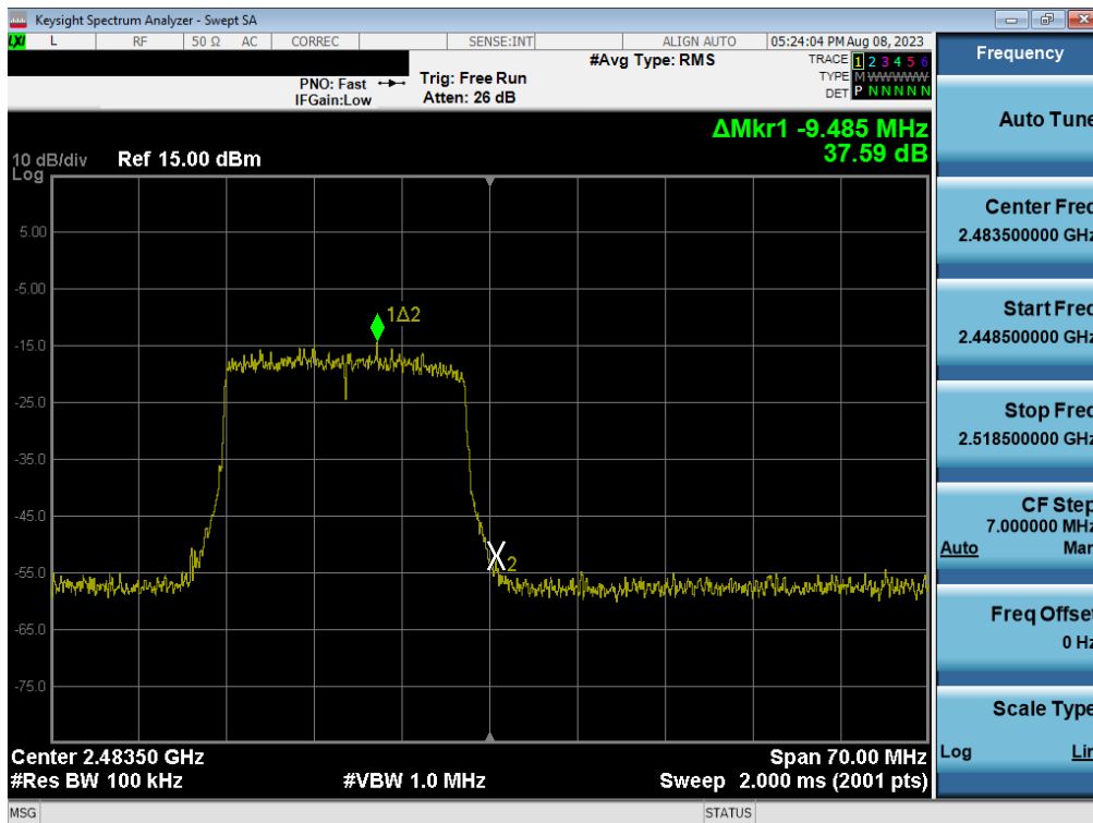
Plot 7-88. Band Edge Plot SISO ANT2 (802.11ax (2.4GHz) – Ch. 13)
