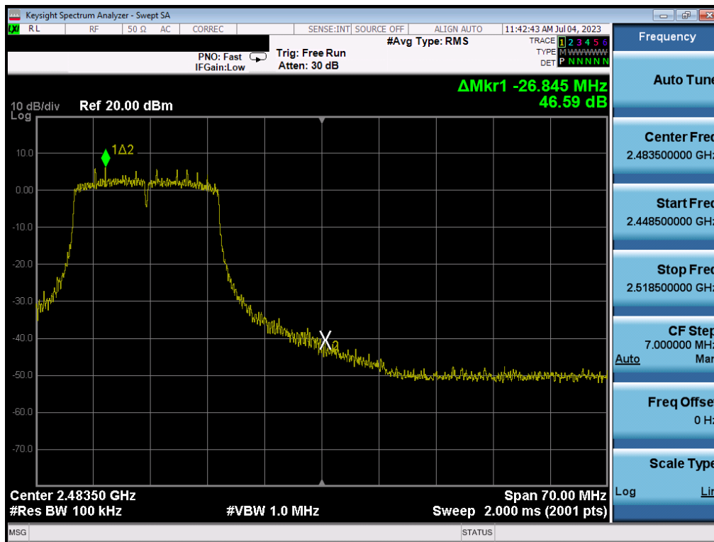
Plot 7-82. Band Edge Plot SISO ANT2 (802.11n (2.4GHz) – Ch. 11)
