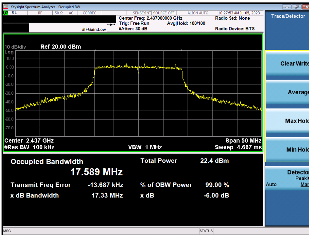
Plot 7-20. 6dB Bandwidth Plot MIMO ANT1 (802.11n (2.4GHz) – Ch. 6)
