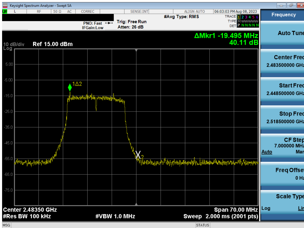
Plot 7-96. Band Edge Plot MIMO ANT1 (802.11g – Ch. 13)
