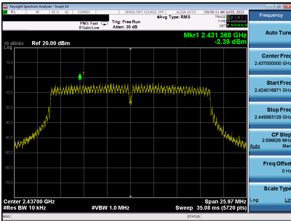
Plot 7-68. Power Spectral Density Plot MIMO ANT2 (802.11n (2.4GHz) – Ch. 6)
