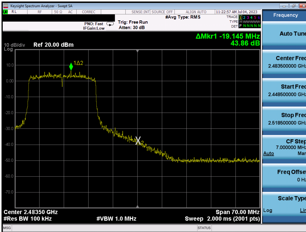
Plot 7-86. Band Edge Plot SISO ANT2 (802.11ax (2.4GHz) – Ch. 11)
