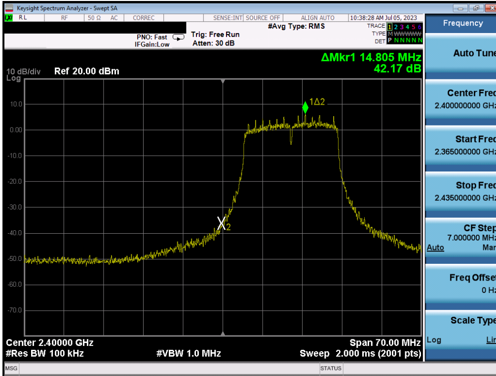
Plot 7-93. Band Edge Plot MIMO ANT1 (802.11g – Ch. 1)
