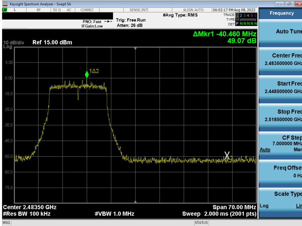
Plot 7-95. Band Edge Plot MIMO ANT1 (802.11g – Ch. 12)
