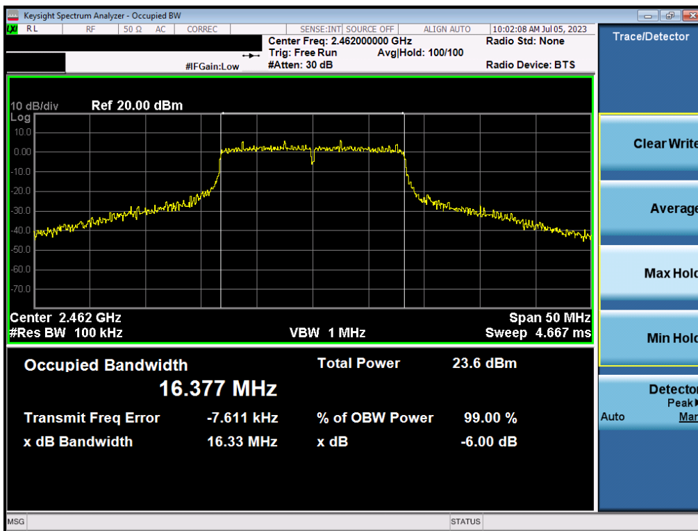
Plot 7-30. 6dB Bandwidth Plot MIMO ANT2 (802.11g – Ch. 11)
