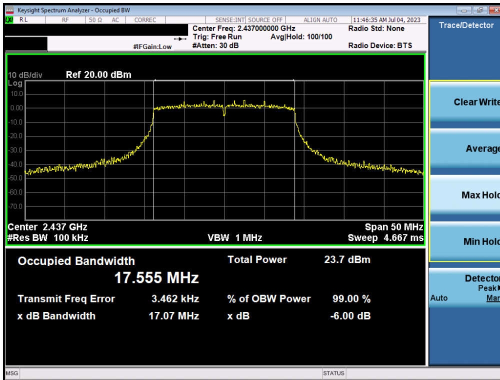
Plot 7-8. 6dB Bandwidth Plot SISO ANT2 (802.11n (2.4GHz) – Ch. 6)
