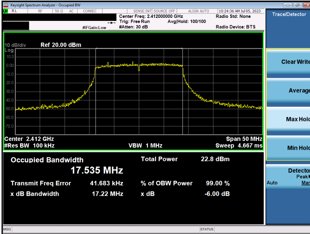
Plot 7-19. 6dB Bandwidth Plot MIMO ANT1 (802.1n (2.4GHz) – Ch. 1)
