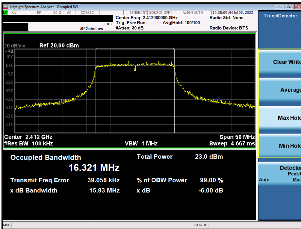
Plot 7-16. 6dB Bandwidth Plot MIMO ANT1 (802.1g – Ch. 1)
