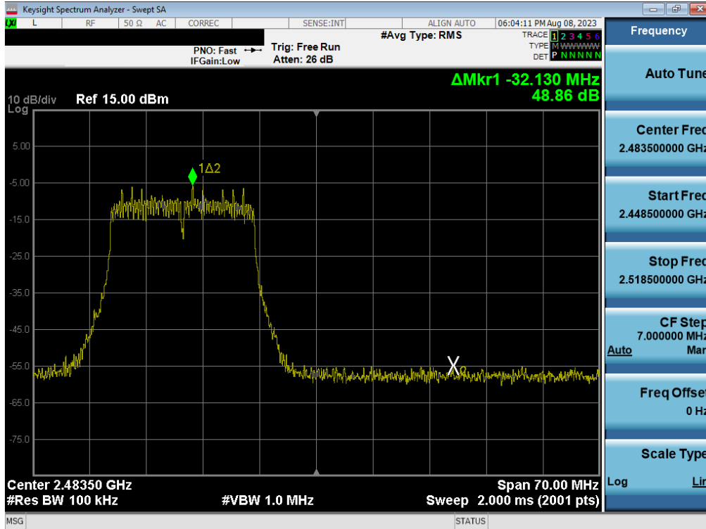
Plot 7-99. Band Edge Plot MIMO ANT1 (802.11n (2.4GHz) – Ch. 12)
