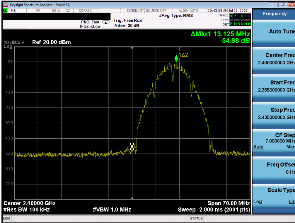
Plot 7-89. Band Edge Plot MIMO ANT1 (802.11b – Ch. 1)
