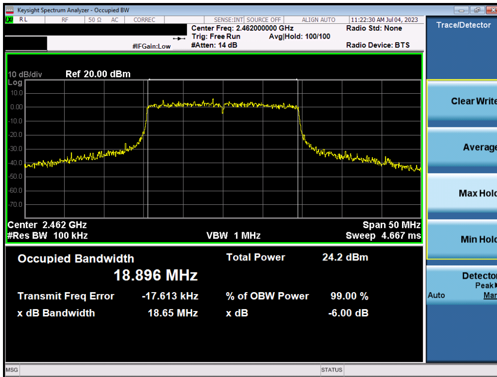
Plot 7-12. 6dB Bandwidth Plot SISO ANT2 (802.11ax (2.4GHz) – Ch. 11)
