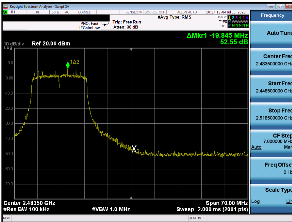
Plot 7-94. Band Edge Plot MIMO ANT1 (802.11g - Ch. 11)
