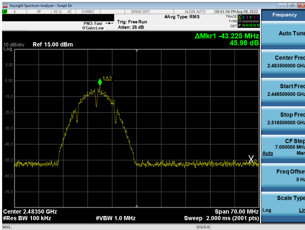
Plot 7-92. Band Edge Plot MIMO ANT1 (802.11b – Ch. 13)
