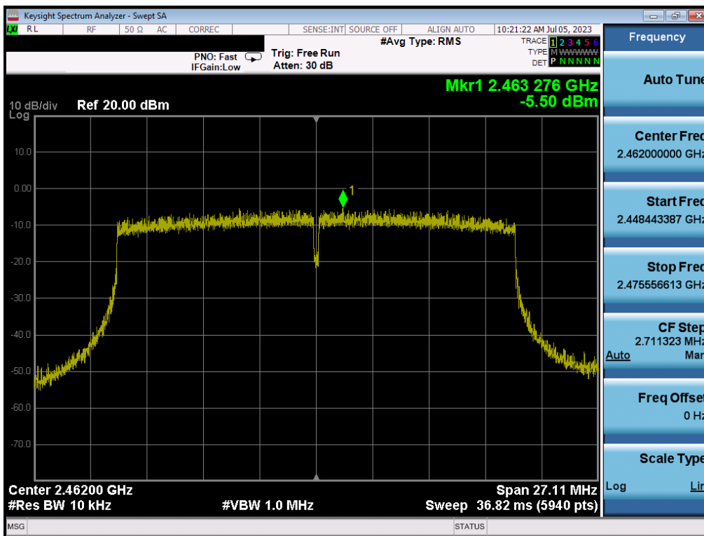
Plot 7-60. Power Spectral Density Plot MIMO ANT1 (802.11ax (2.4GHz) – Ch. 11)
