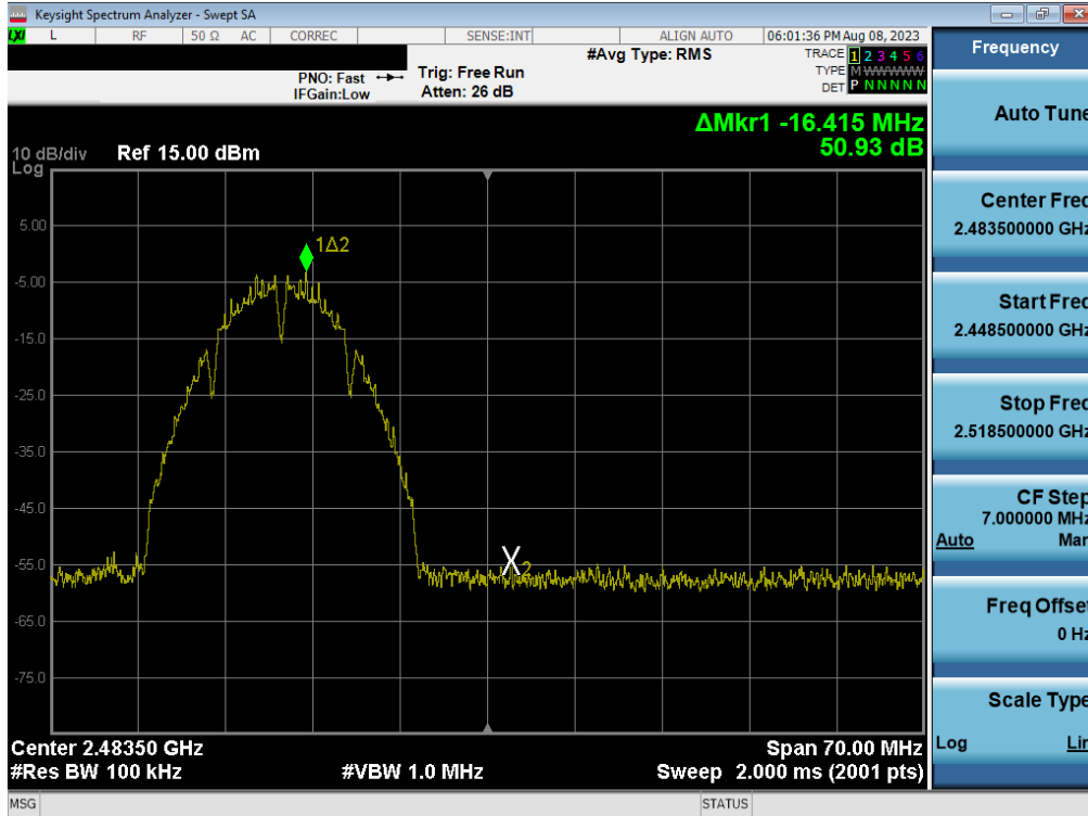
Plot 7-91. Band Edge Plot MIMO ANT1 (802.11b – Ch. 12)
