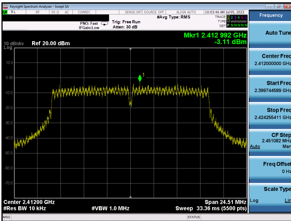
Plot 7-64. Power Spectral Density Plot MIMO ANT2 (802.11g – Ch. 1)
