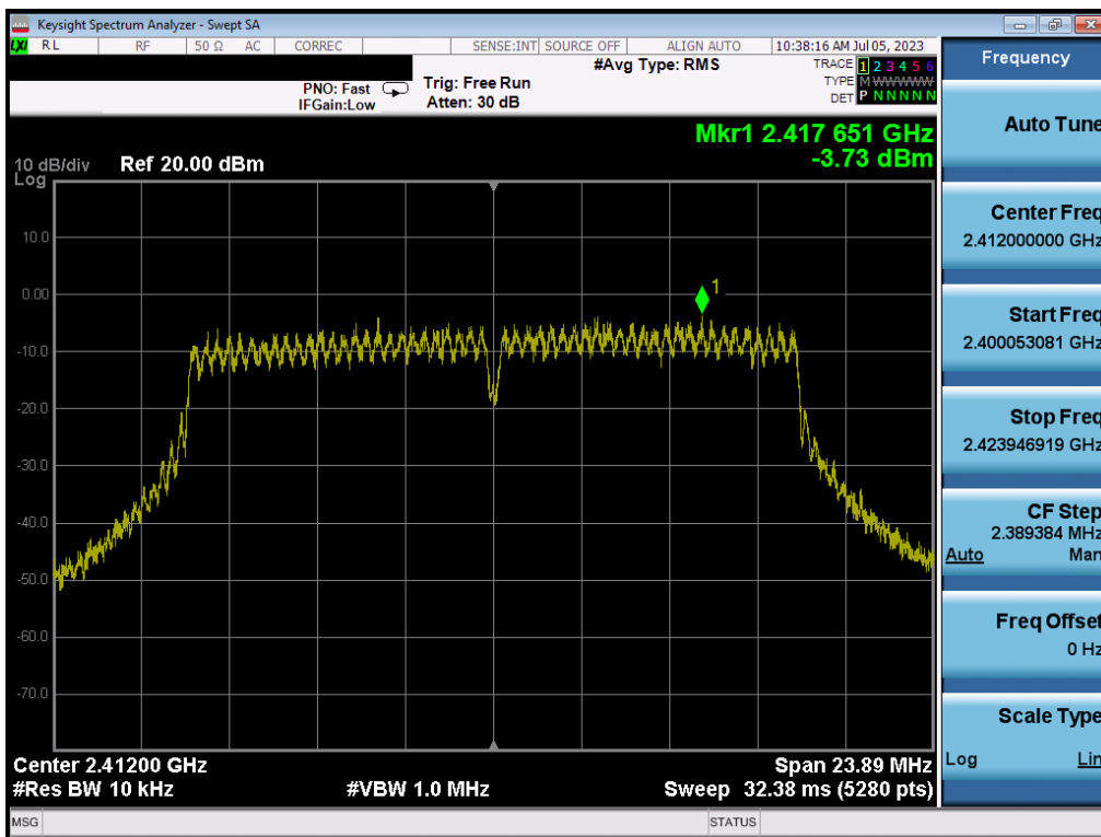
Plot 7-52. Power Spectral Density Plot MIMO ANT1 (802.11g – Ch. 1)
