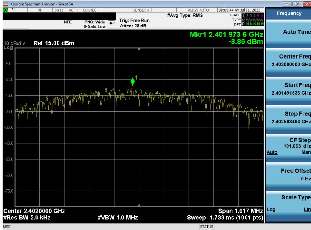
Plot 7-31. Power Spectral Density Plot (Bluetooth (LE), 1Mbps – Ch. 0) – ANT 1
