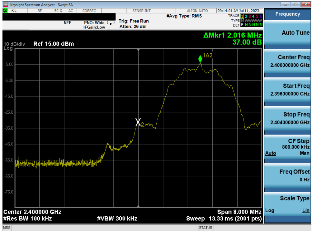
Plot 7-43. Band Edge Plot (Bluetooth (LE), 2Mbps – Ch. 0) – ANT 1
