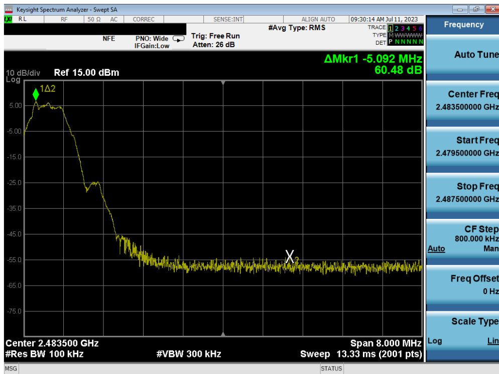
Plot 7-40. Band Edge Plot (Bluetooth (LE), 500kbps – Ch. 39) – ANT 1
