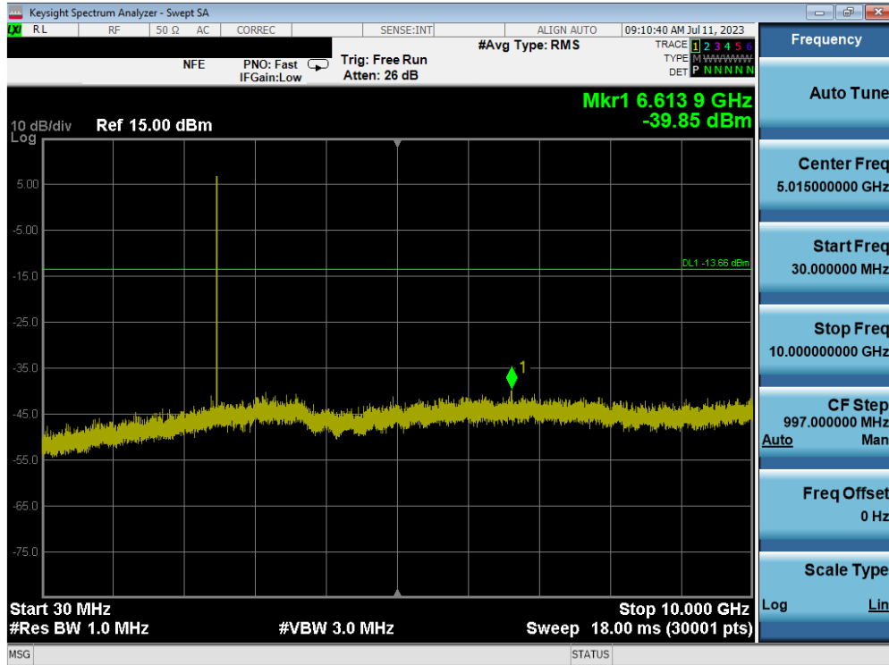
Plot 7-49. Conducted Spurious Plot (Bluetooth (LE), 1Mbps – Ch. 39) – ANT 1
