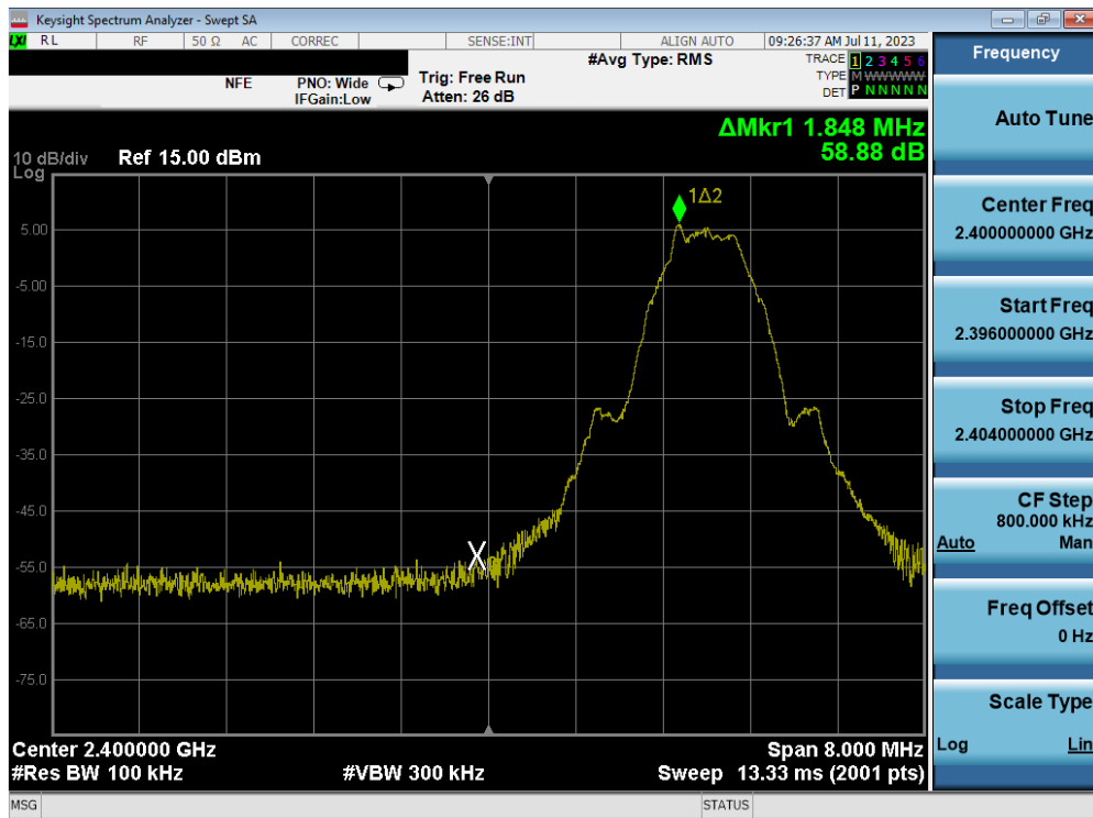
Plot 7-39. Band Edge Plot (Bluetooth (LE), 500kbps – Ch. 0) – ANT 1
