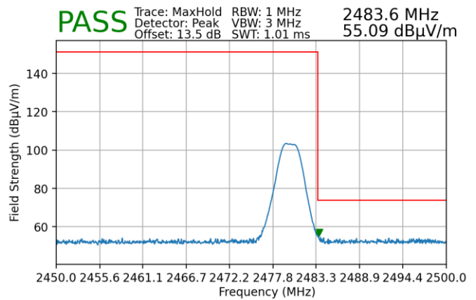
Plot 7-52. Radiated Restricted Upper Band Edge Measurement (Peak) – ANT 1
