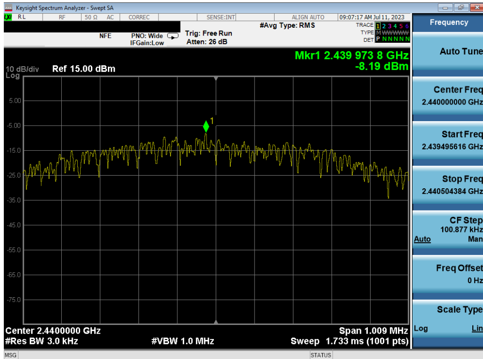
Plot 7-32. Power Spectral Density Plot (Bluetooth (LE), 1Mbps – Ch. 19) – ANT 1
