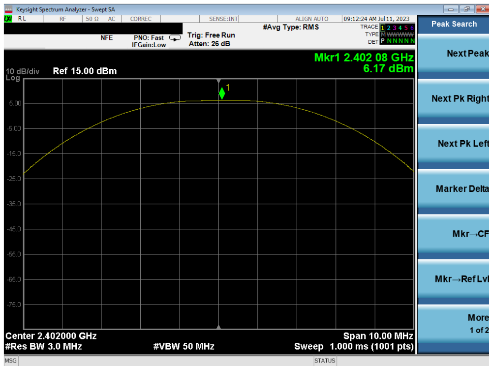
Plot 7-22. Peak Power Plot (Bluetooth (LE), 2Mbps – Ch. 0) – ANT 1
