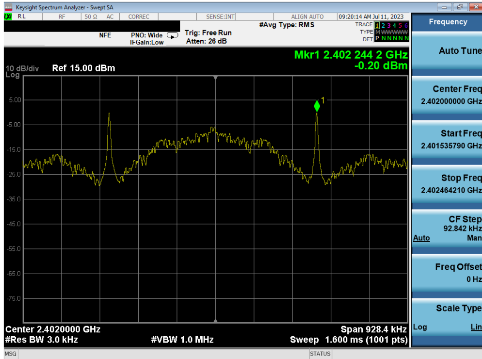
Plot 7-25. Power Spectral Density Plot (Bluetooth (LE), 125kbps – Ch. 0) – ANT 1
