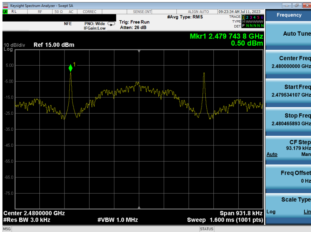
Plot 7-27. Power Spectral Density Plot (Bluetooth (LE), 125kbps – Ch. 39) – ANT 1
