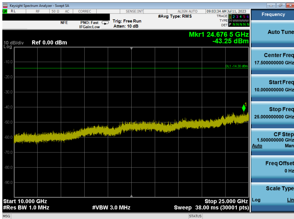
Plot 7-46. Conducted Spurious Plot (Bluetooth (LE), 1Mbps – Ch. 0) – ANT 1
