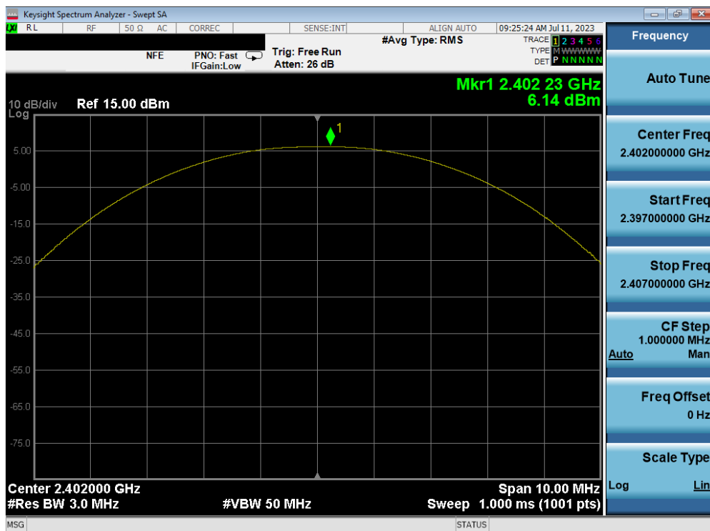
Plot 7-16. Peak Power Plot (Bluetooth (LE), 500kbps – Ch. 0) – ANT 1
