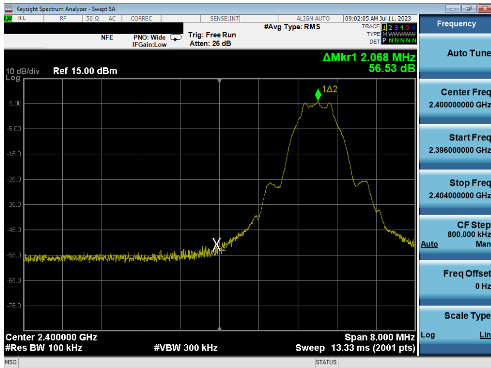
Plot 7-41. Band Edge Plot (Bluetooth (LE), 1Mbps – Ch. 0) – ANT 1
