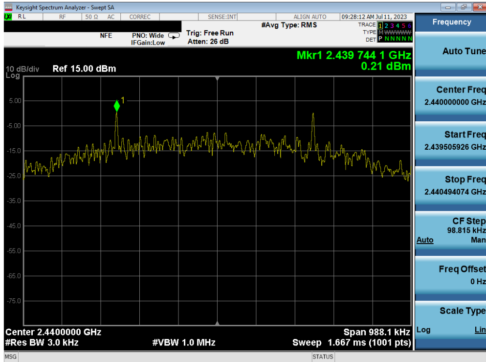
Plot 7-29. Power Spectral Density Plot (Bluetooth (LE), 500kbps – Ch. 19) – ANT 1
