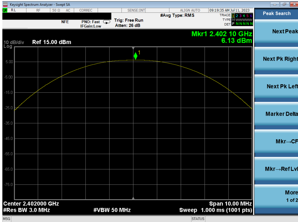
Plot 7-13. Peak Power Plot (Bluetooth (LE), 125kbps – Ch. 0) – ANT 1
