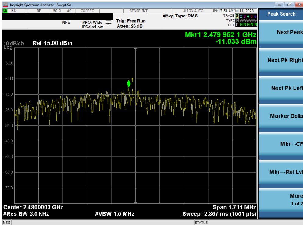
Plot 7-36. Power Spectral Density Plot (Bluetooth (LE), 2Mbps – Ch. 39) – ANT 1
