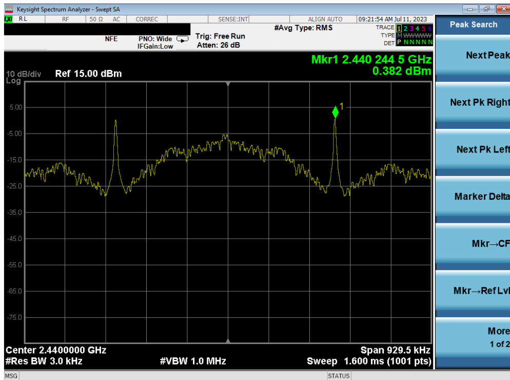
Plot 7-26. Power Spectral Density Plot (Bluetooth (LE), 125kbps – Ch. 19) – ANT 1
