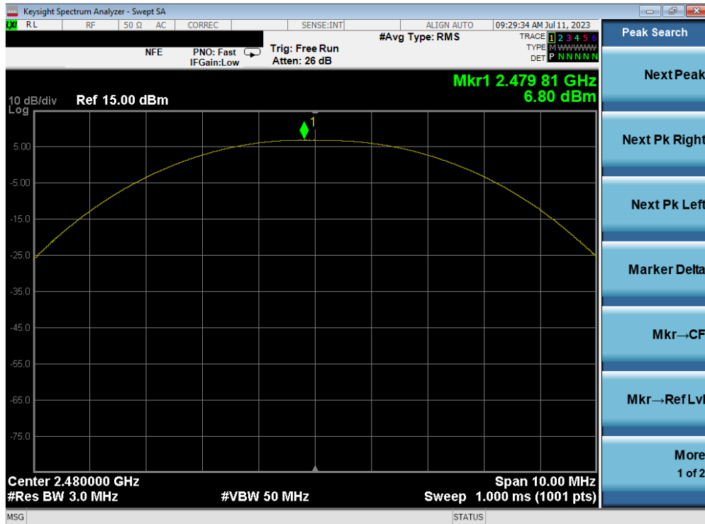
Plot 7-18. Peak Power Plot (Bluetooth (LE), 500kbps – Ch. 39) – ANT 1
