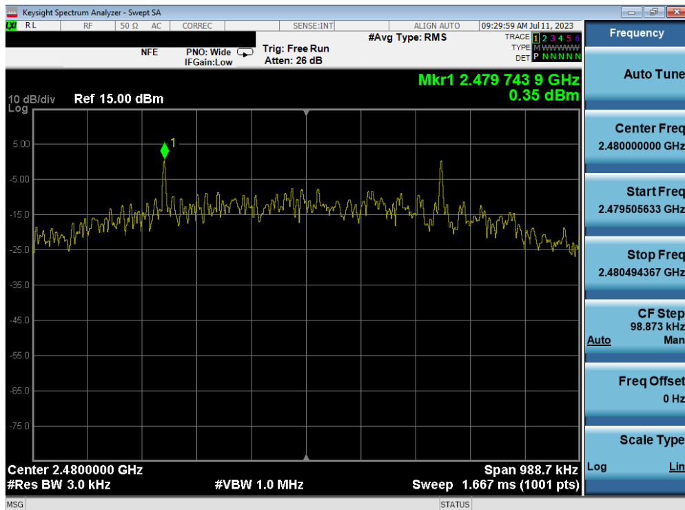
Plot 7-30. Power Spectral Density Plot (Bluetooth (LE), 500kbps – Ch. 39) – ANT 1
