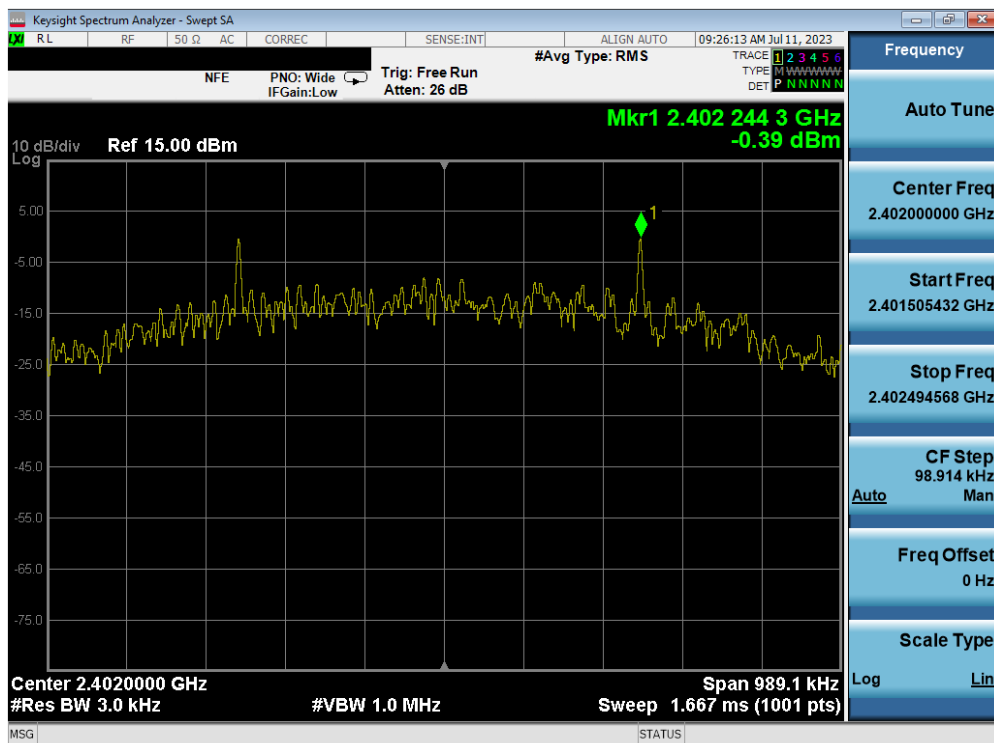
Plot 7-28. Power Spectral Density Plot (Bluetooth (LE), 500kbps – Ch. 0) – ANT 1
