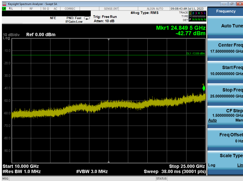
Plot 7-48. Conducted Spurious Plot (Bluetooth (LE), 1Mbps – Ch. 19) – ANT 1
