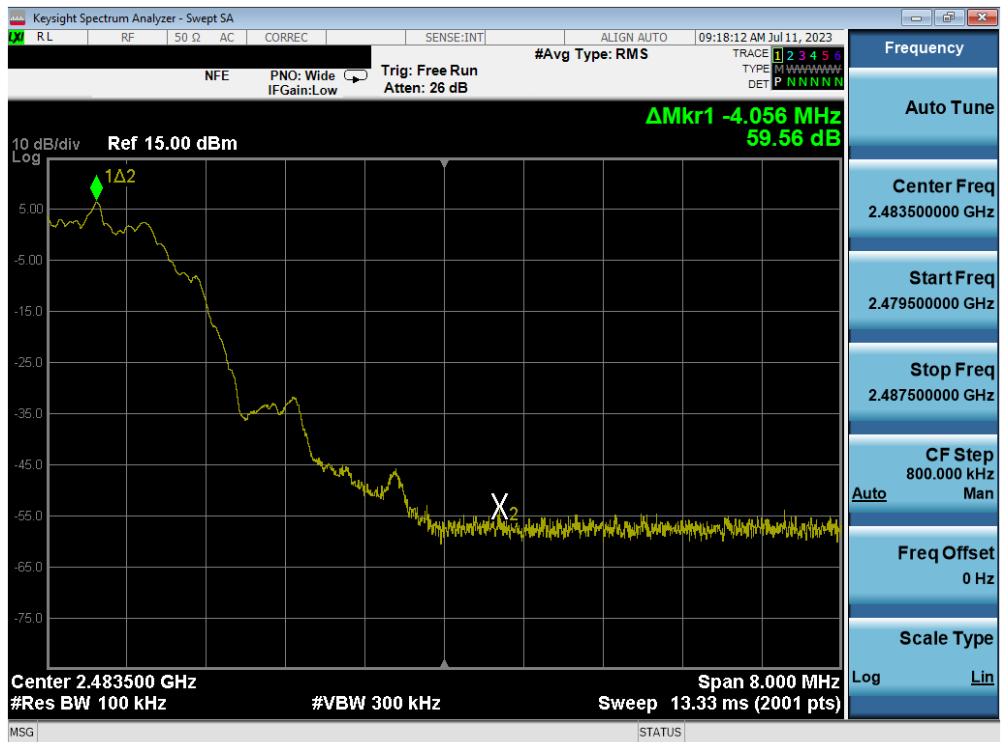
Plot 7-44. Band Edge Plot (Bluetooth (LE), 2Mbps – Ch. 39) – ANT 1
