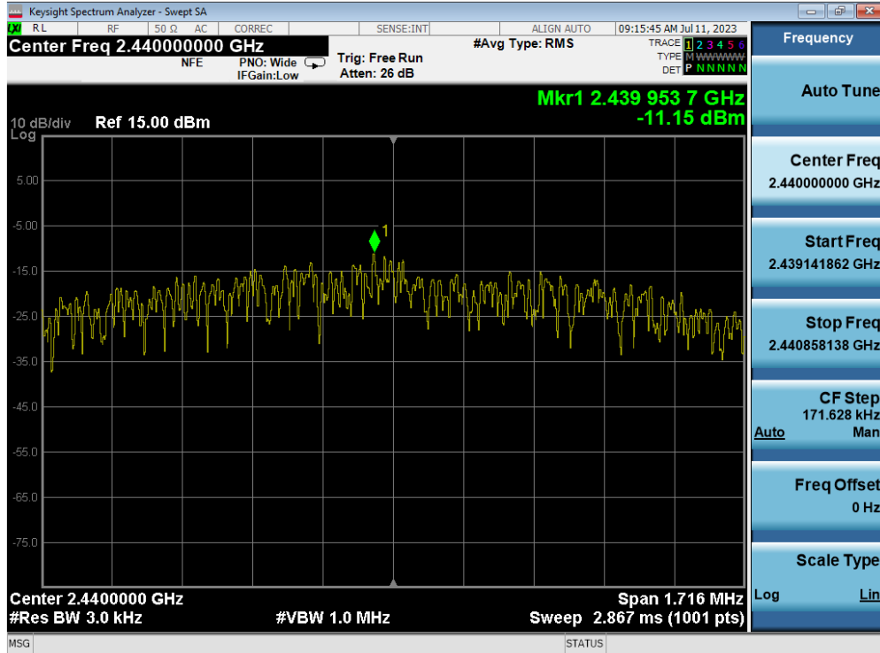
Plot 7-35. Power Spectral Density Plot (Bluetooth (LE), 2Mbps – Ch. 19) – ANT 1
