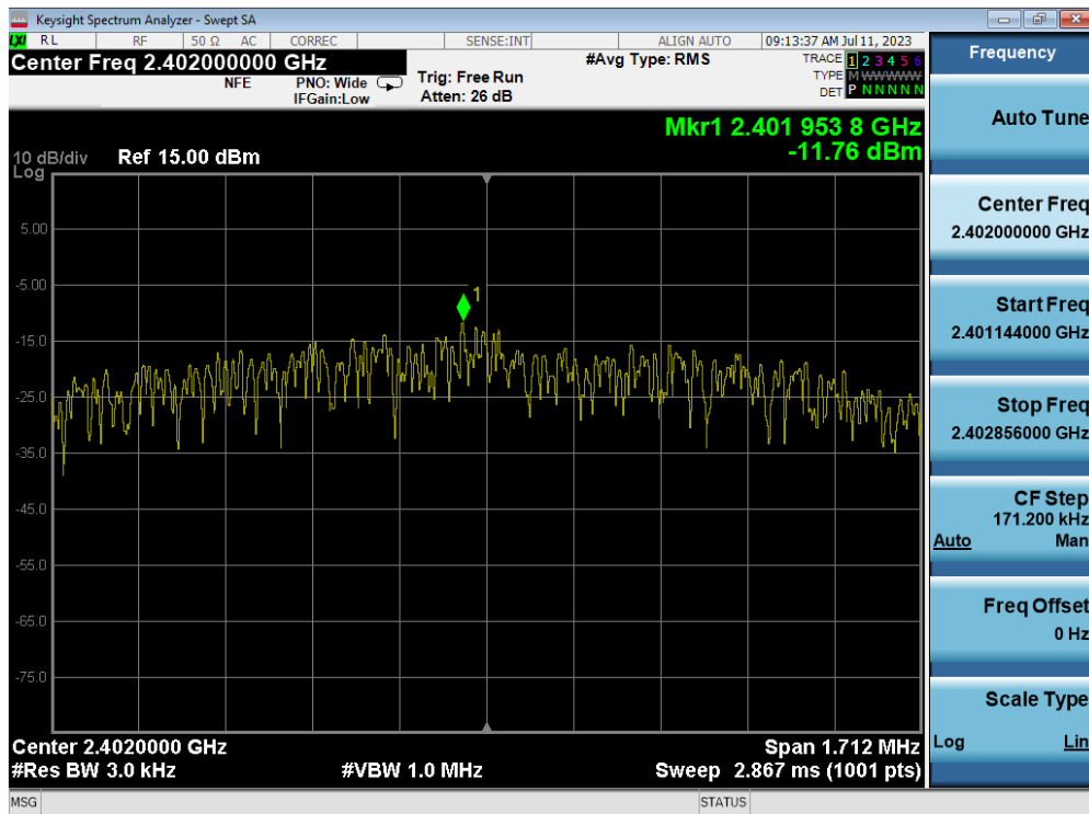
Plot 7-34. Power Spectral Density Plot (Bluetooth (LE), 2Mbps – Ch. 0) – ANT 1
