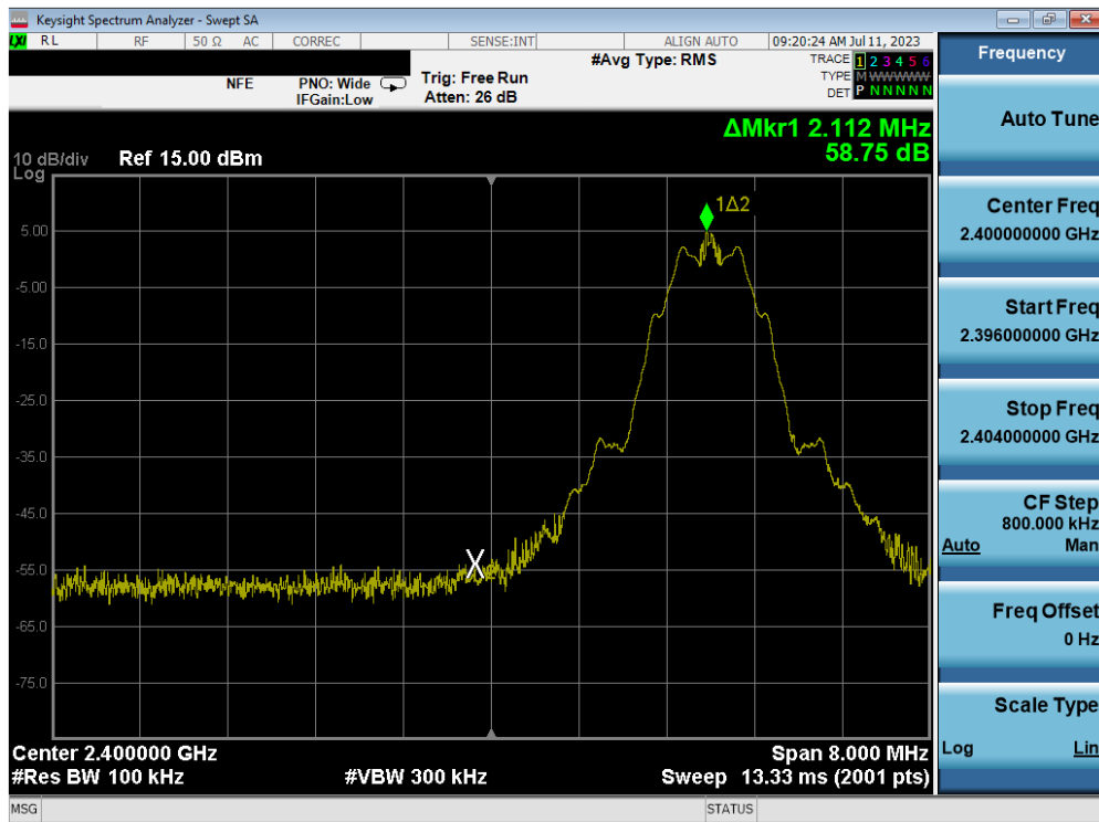
Plot 7-37. Band Edge Plot (Bluetooth (LE), 125kbps – Ch. 0) – ANT 1
