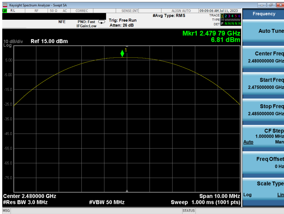
Plot 7-21. Peak Power Plot (Bluetooth (LE), 1Mbps – Ch. 39) – ANT 1
