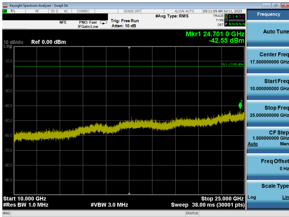
Plot 7-50. Conducted Spurious Plot (Bluetooth (LE), 1Mbps – Ch. 39) – ANT 1
