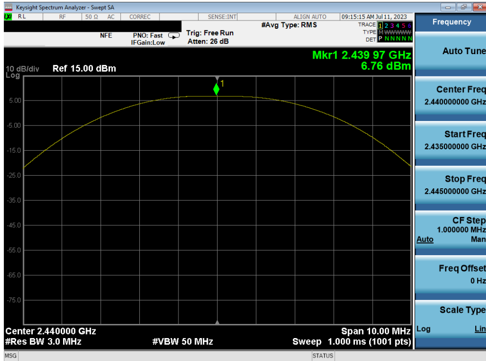
Plot 7-23. Peak Power Plot (Bluetooth (LE), 2Mbps – Ch. 19) – ANT 1
