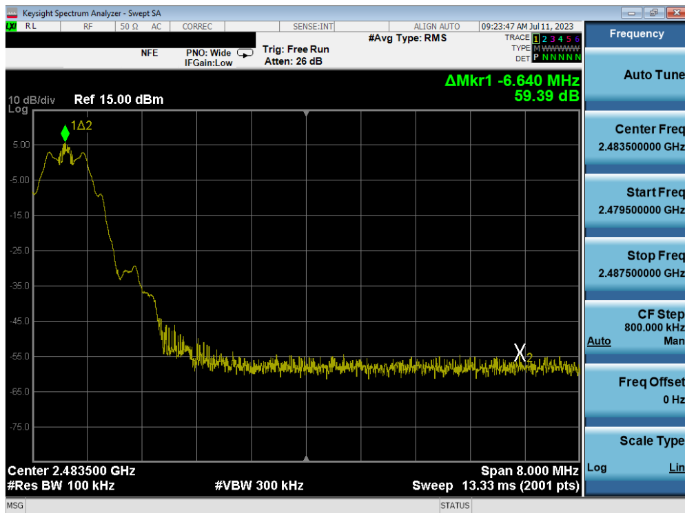
Plot 7-38. Band Edge Plot (Bluetooth (LE), 125kbps – Ch. 39) – ANT 1
