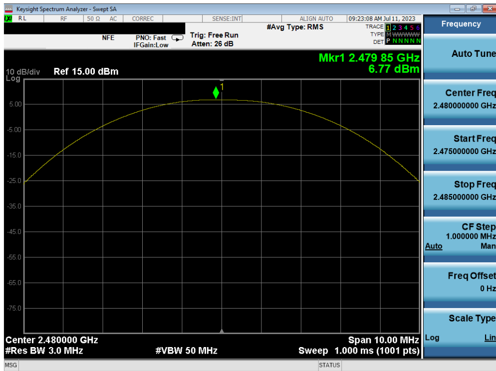
Plot 7-15. Peak Power Plot (Bluetooth (LE), 125kbps – Ch. 39) – ANT 1
