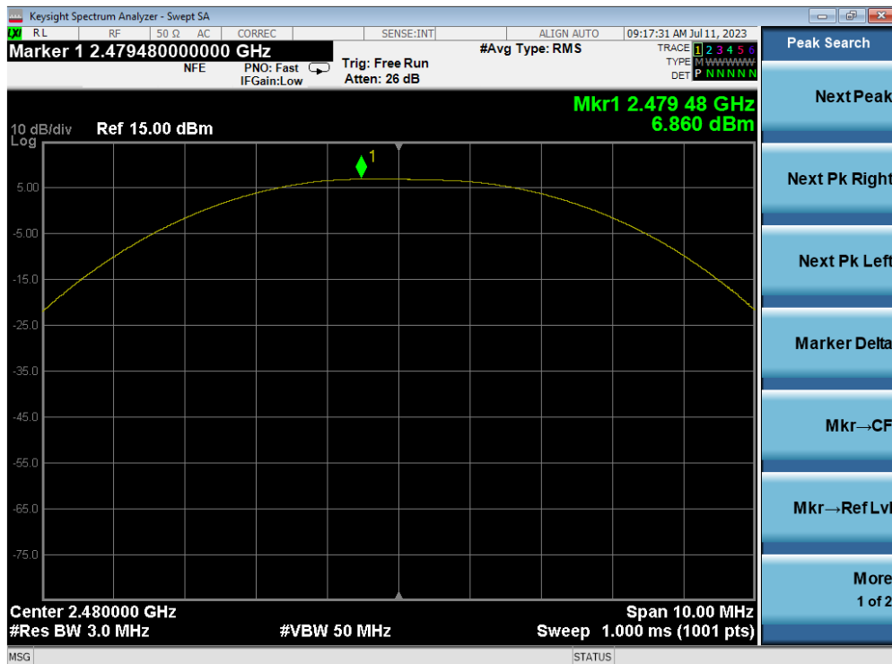
Plot 7-24. Peak Power Plot (Bluetooth (LE), 2Mbps – Ch. 39) – ANT 1
