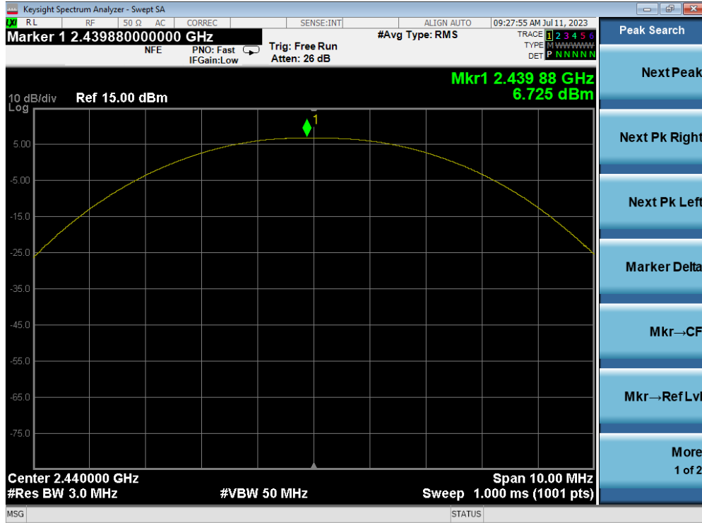
Plot 7-17. Peak Power Plot (Bluetooth (LE), 500kbps – Ch. 19) – ANT 1
