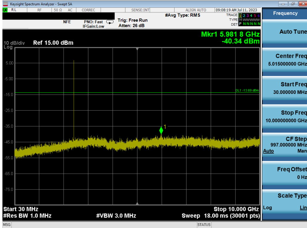
Plot 7-47. Conducted Spurious Plot (Bluetooth (LE), 1Mbps – Ch. 19) – ANT 1
