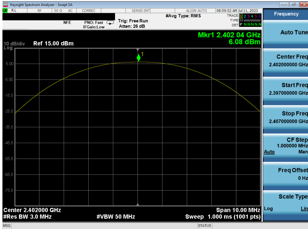
Plot 7-19. Peak Power Plot (Bluetooth (LE), 1Mbps – Ch. 0) – ANT 1
