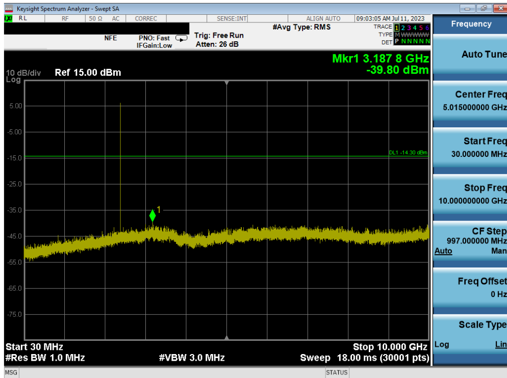
Plot 7-45. Conducted Spurious Plot (Bluetooth (LE), 1Mbps – Ch. 0) – ANT 1
