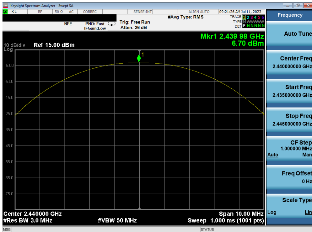
Plot 7-14. Peak Power Plot (Bluetooth (LE), 125kbps – Ch. 19) – ANT 1
