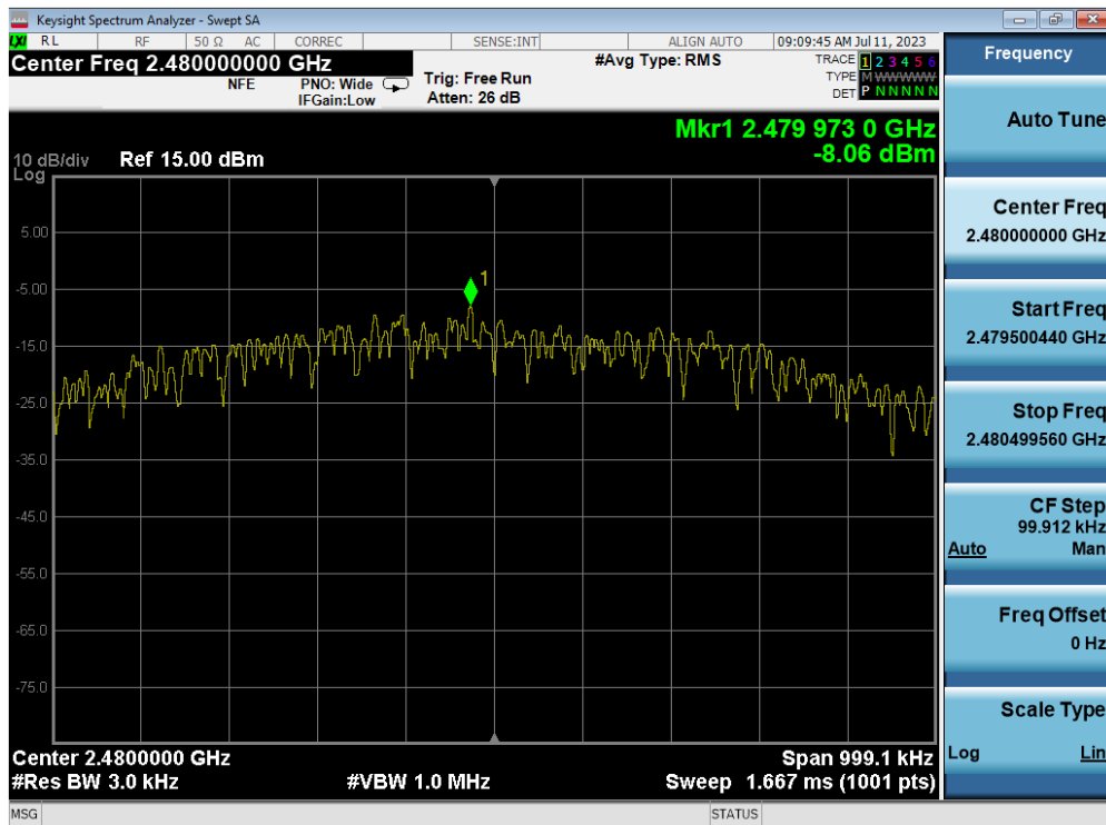
Plot 7-33. Power Spectral Density Plot (Bluetooth (LE), 1Mbps – Ch. 39) – ANT 1
