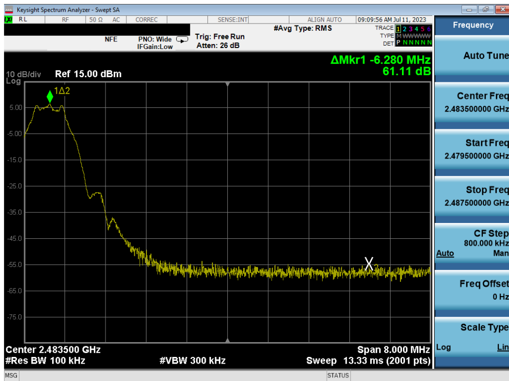
Plot 7-42. Band Edge Plot (Bluetooth (LE), 1Mbps – Ch. 39) – ANT 1
