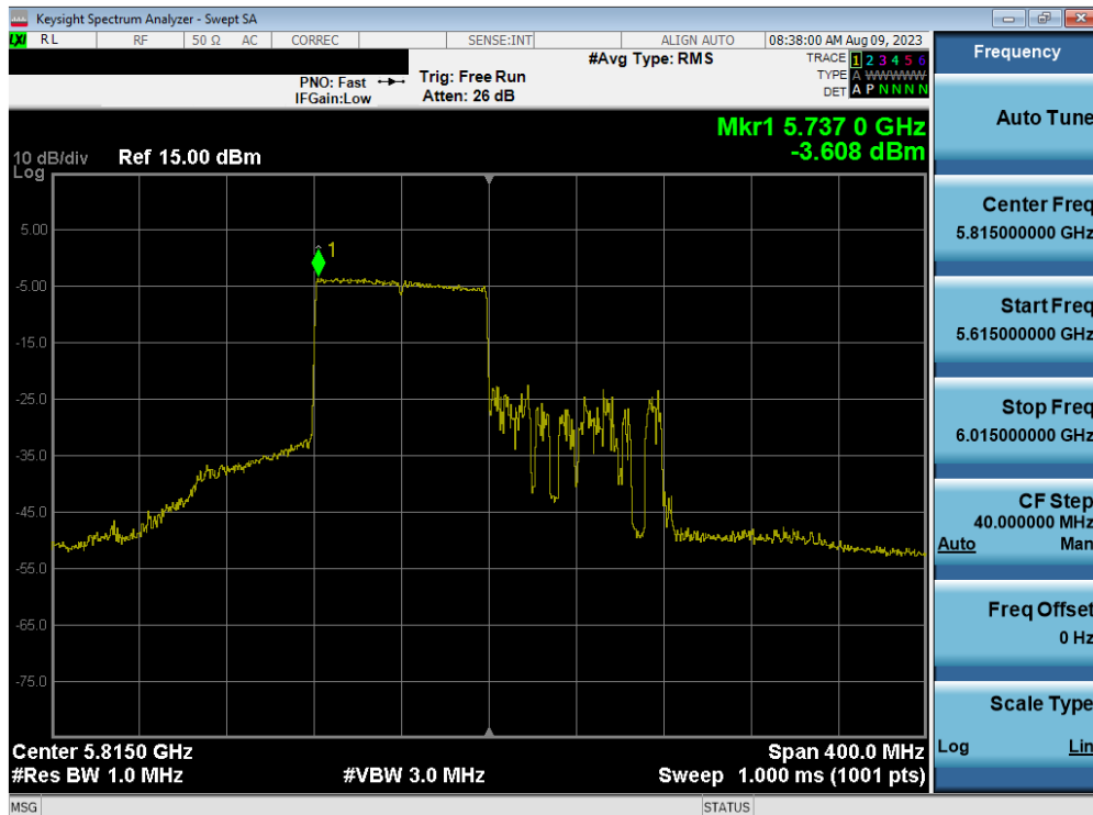
Plot 7-108. Power Spectral Density Plot MIMO ANT1 (160MHz BW 802.11ax – 996 Tones (UNII Band 3/4) – Ch. 163)
