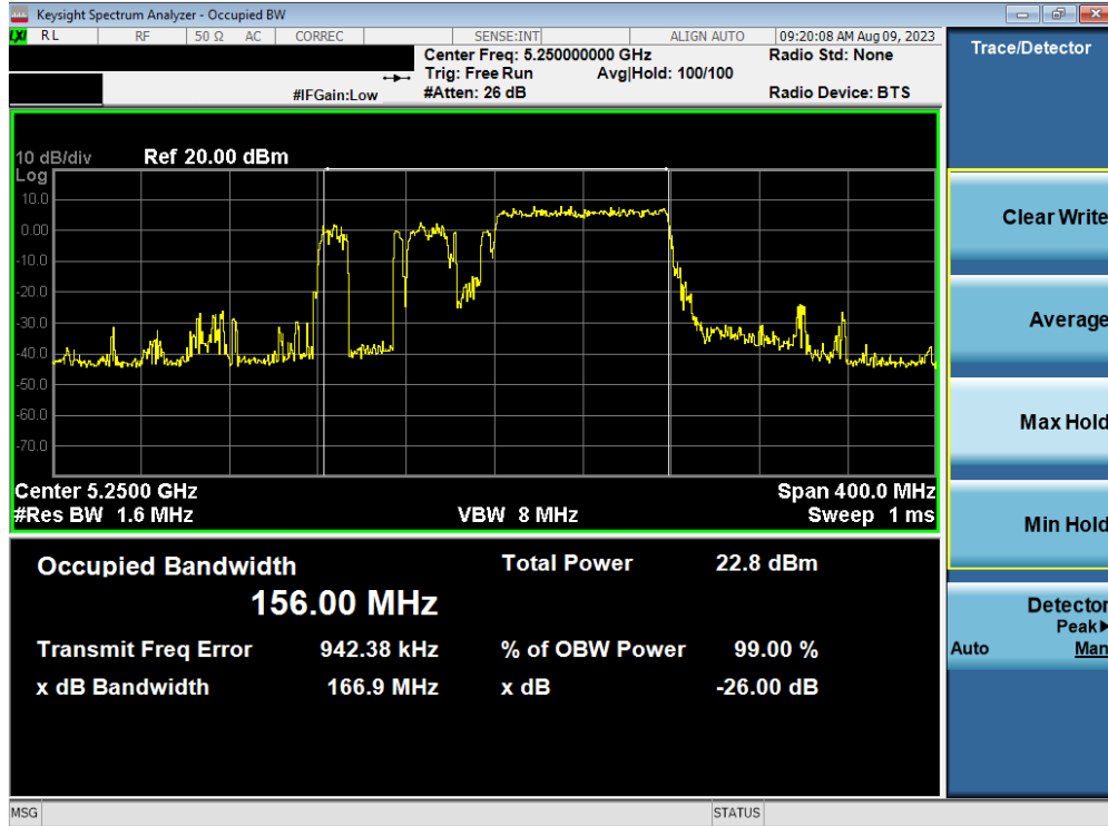
Plot 7-37. 26dB Bandwidth Plot MIMO ANT2 (160MHz BW 802.11ax – 996 Tones (UNII Band 1/2A) – Ch. 50)
