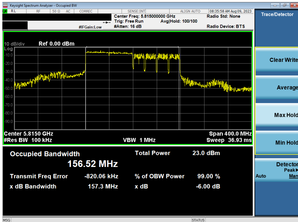
Plot 7-72. 6dB Bandwidth Plot MIMO ANT2 (160MHz BW 802.11ax – 996 Tones (UNII Band 3/4) – Ch. 163)
