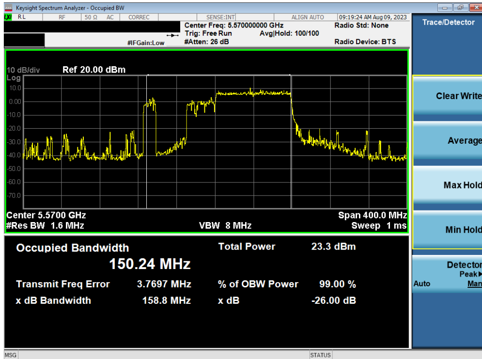
Plot 7-44. 26dB Bandwidth Plot MIMO ANT2 (160MHz BW 802.11ax – 996 Tones (UNII Band 2C) – Ch. 114)
