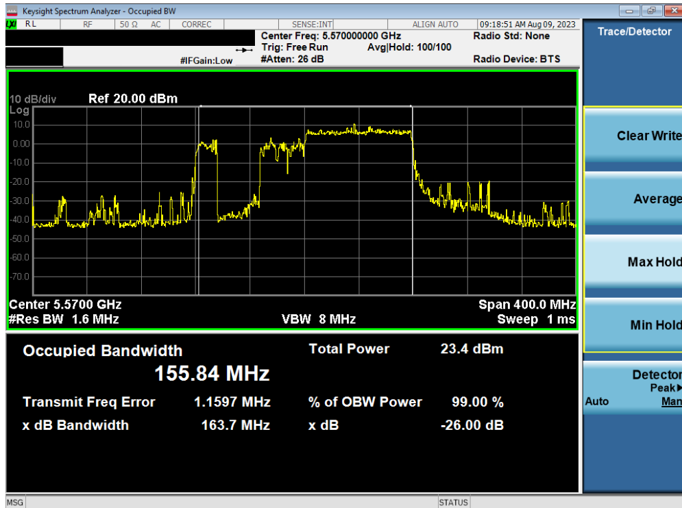
Plot 7-22. 26dB Bandwidth Plot MIMO ANT1 (160MHz BW 802.11ax – 996 Tones (UNII Band 2C) – Ch. 114)
