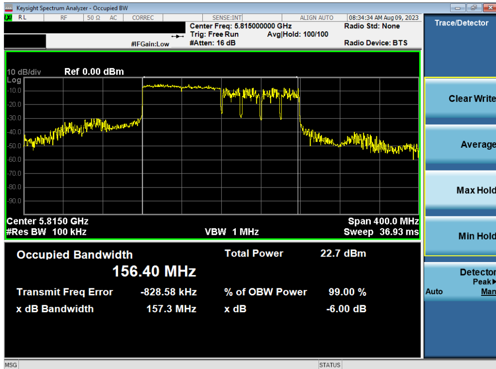
Plot 7-58. 6dB Bandwidth Plot MIMO ANT1 (160MHz BW 802.11ax – 996 Tones (UNII Band 3/4) – Ch. 163)
