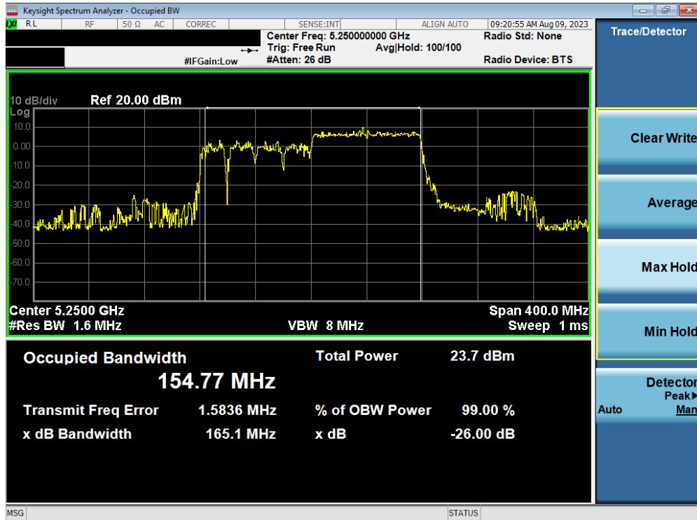
Plot 7-15. 26dB Bandwidth Plot MIMO ANT1 (160MHz BW 802.11ax – 996 Tones (UNII Band 1/2A) – Ch. 50)
