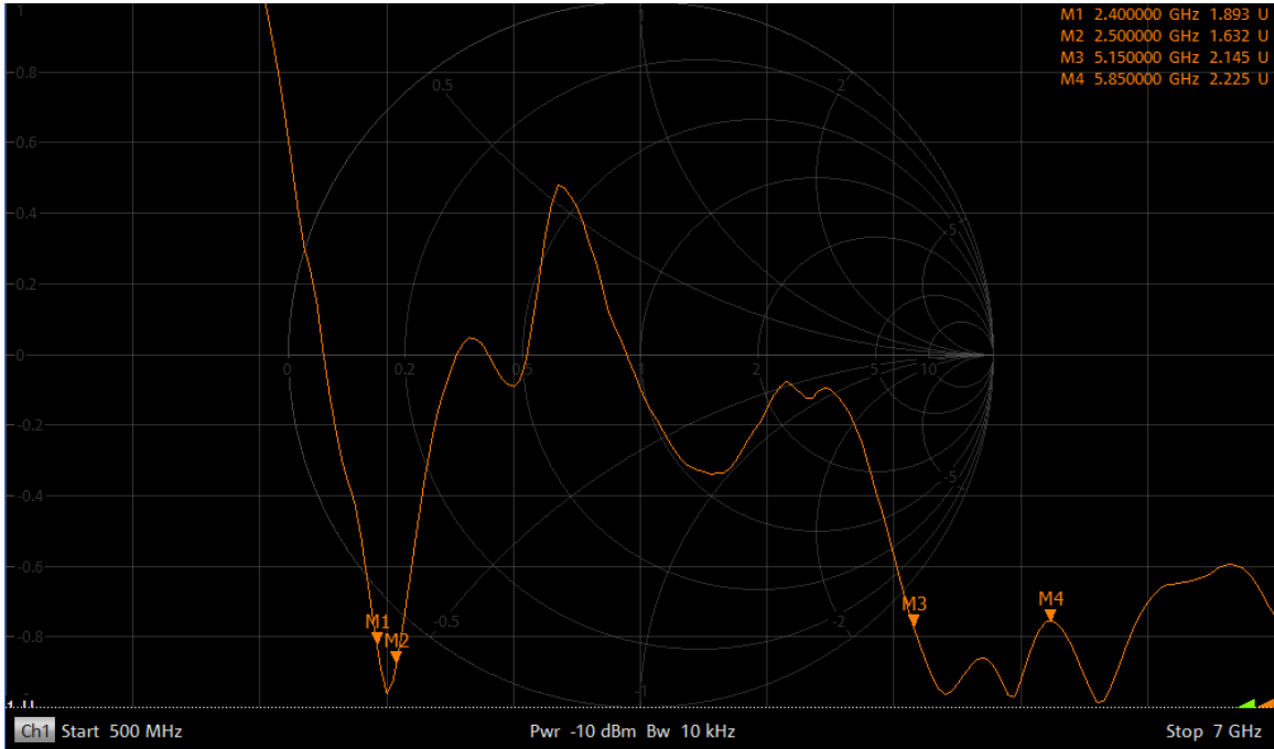
WiFi Antenna
