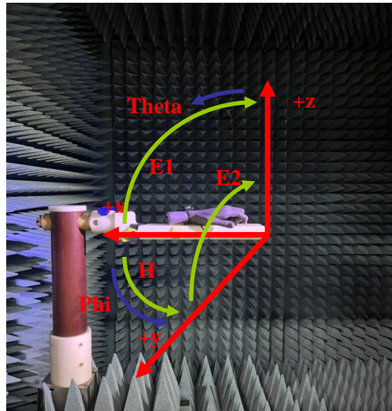
Figure 4: Geometry for SM-R965 for Radiation patterns.
