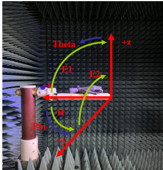
Figure 4: Geometry for SM-R945 for Radiation patterns.
