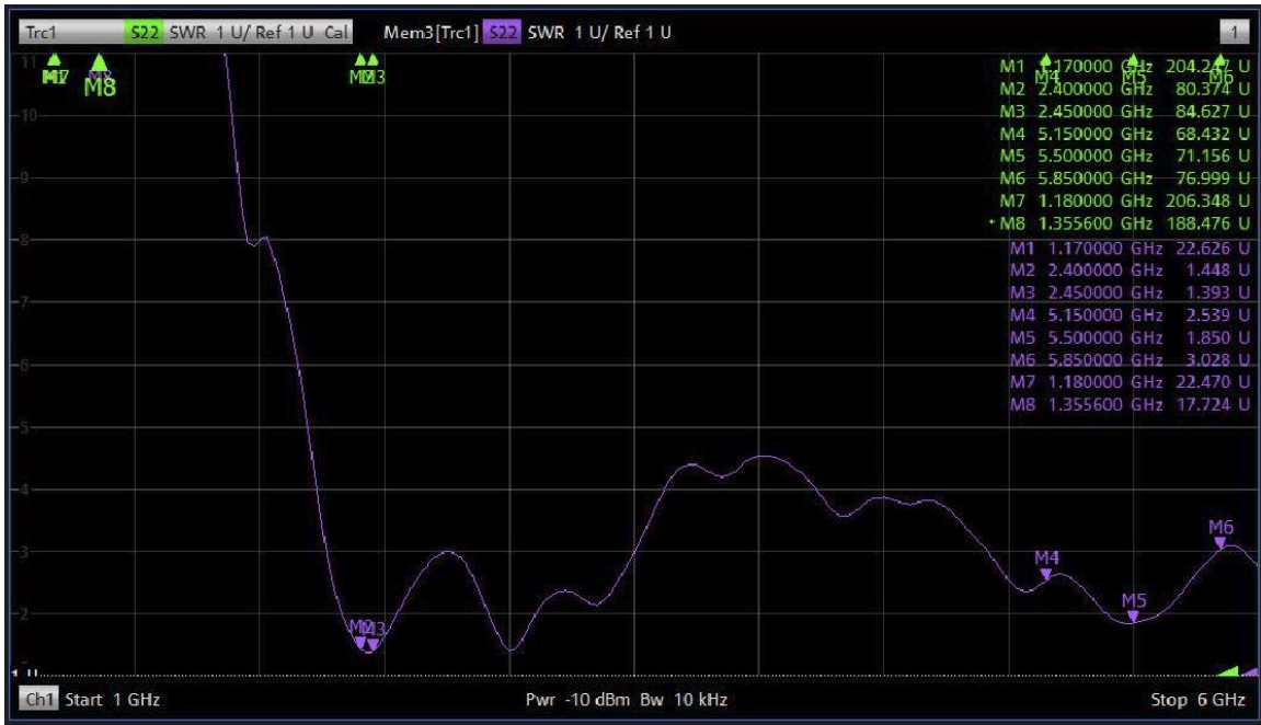
WiFi Antenna
