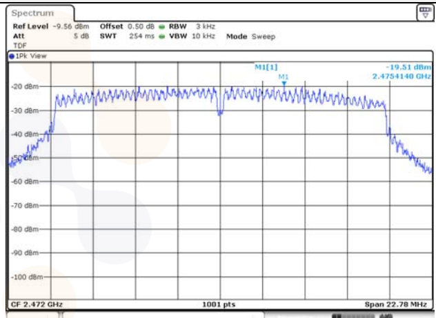
802.11n HT20 / 2 472 MHz
