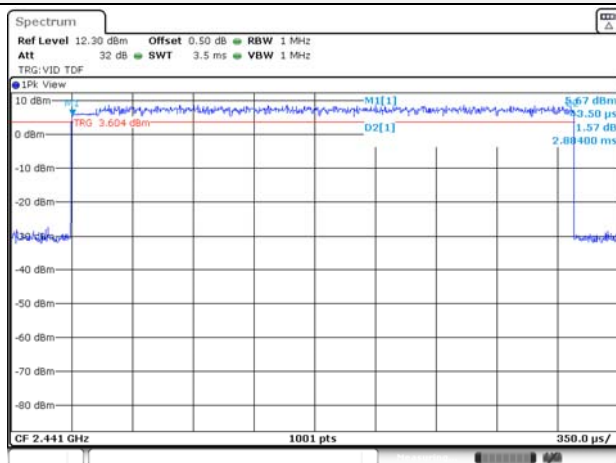
8DPSK / 3-DH5
