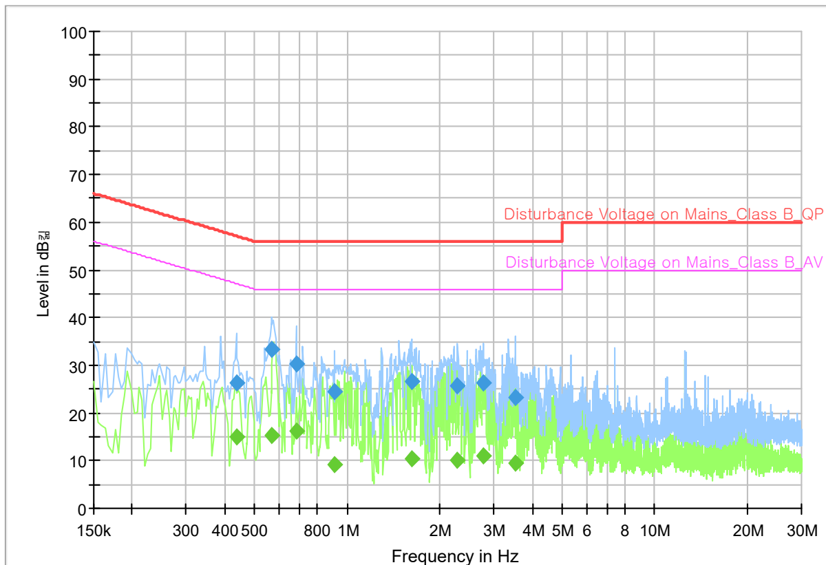
Worst Case_U-NII-3_802.11a_5745
