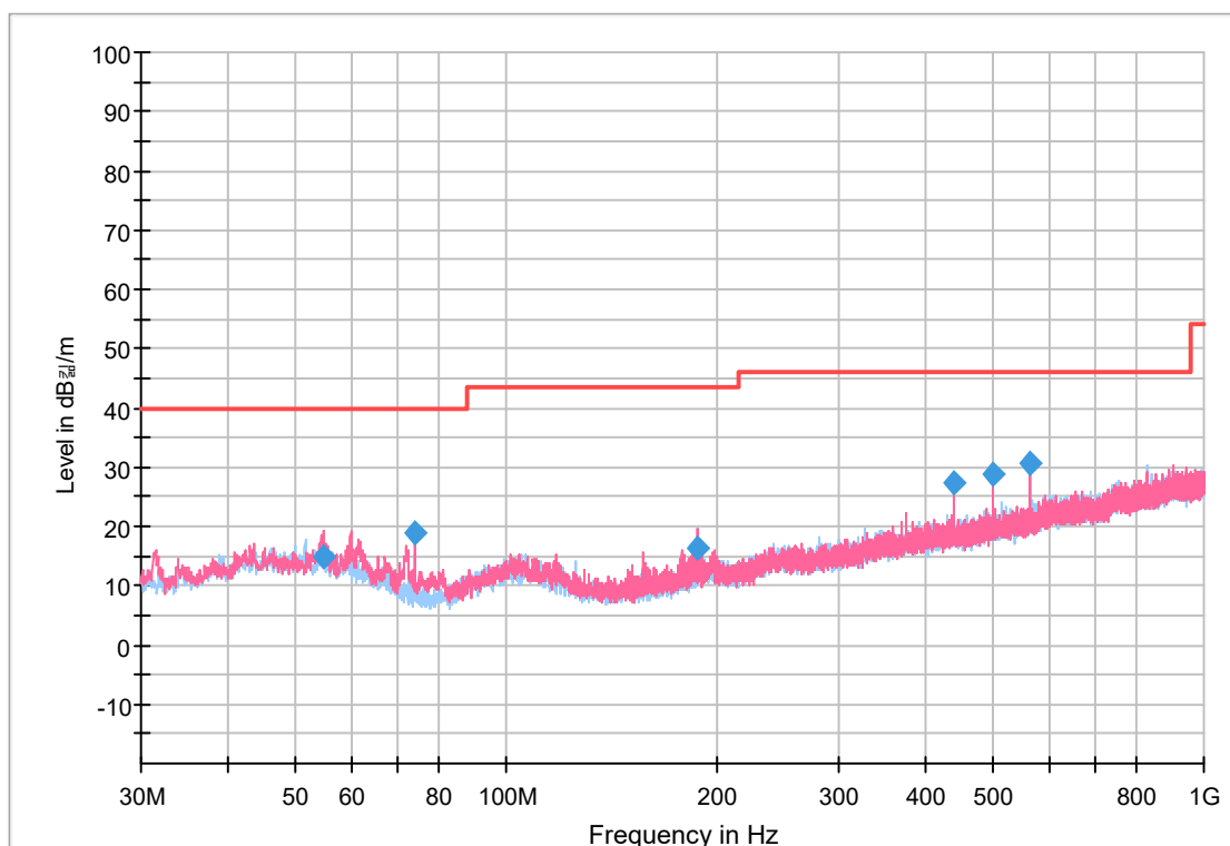
Worst case - RSE(Below 1 GHz)_2.4GHz WLAN_802.11b_2462
