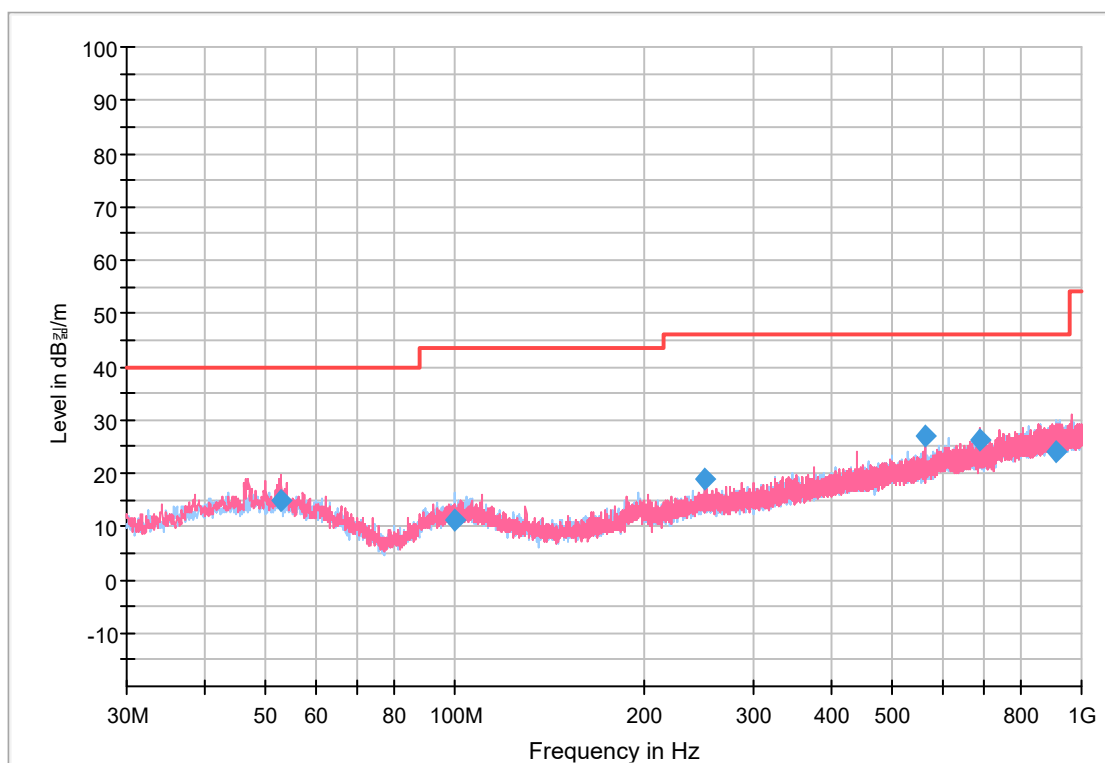
Worst case - RSE(Below 1 GHz)_Bluetooth LE 2M_GFSK_2480
