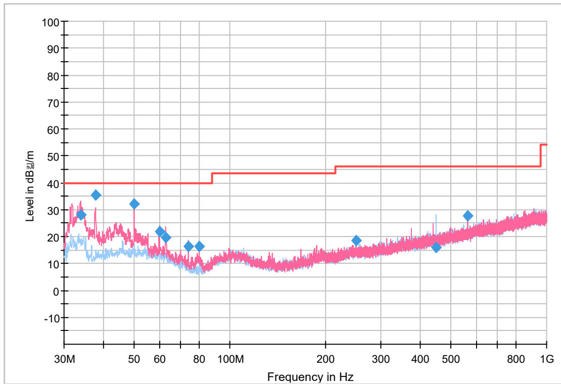
Worst case - RSE(Below 1 GHz)_Bluetooth_GFSK_2441
