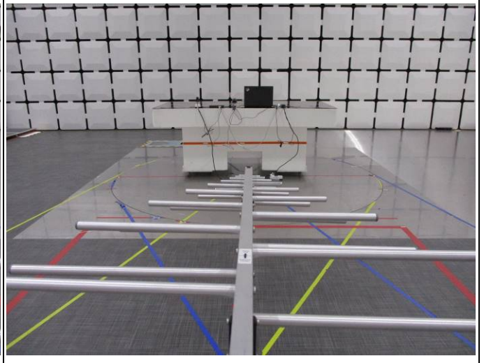
REAR VIEW #3
