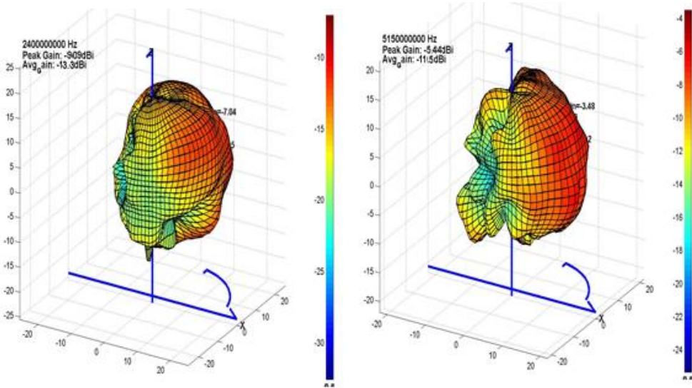
<Smart Watch mounted typical measurements>
