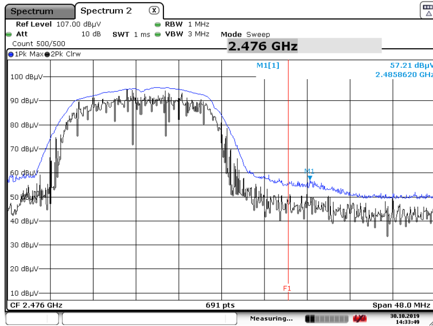
Radiated Restricted Band Edges plot – Peak Reading (802.11g_6Mbps Ch.12)
