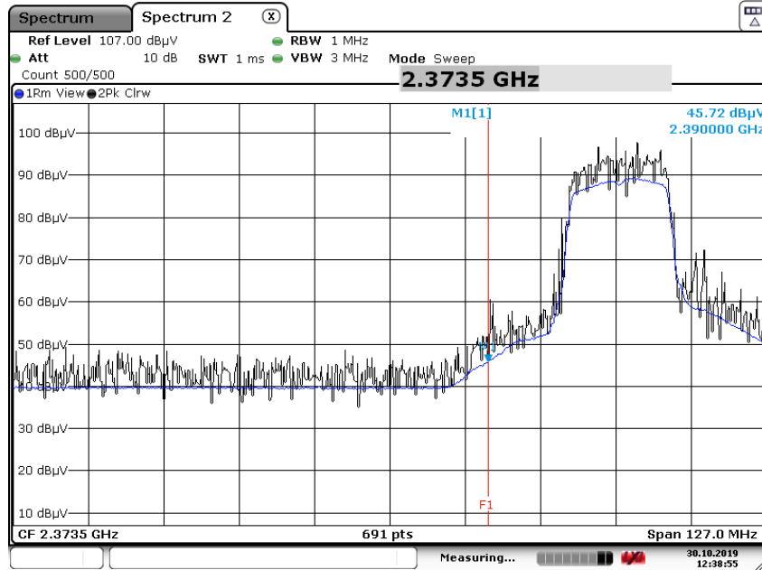
Radiated Restricted Band Edges plot – Average Reading (802.11g_6Mbps Ch.1)
