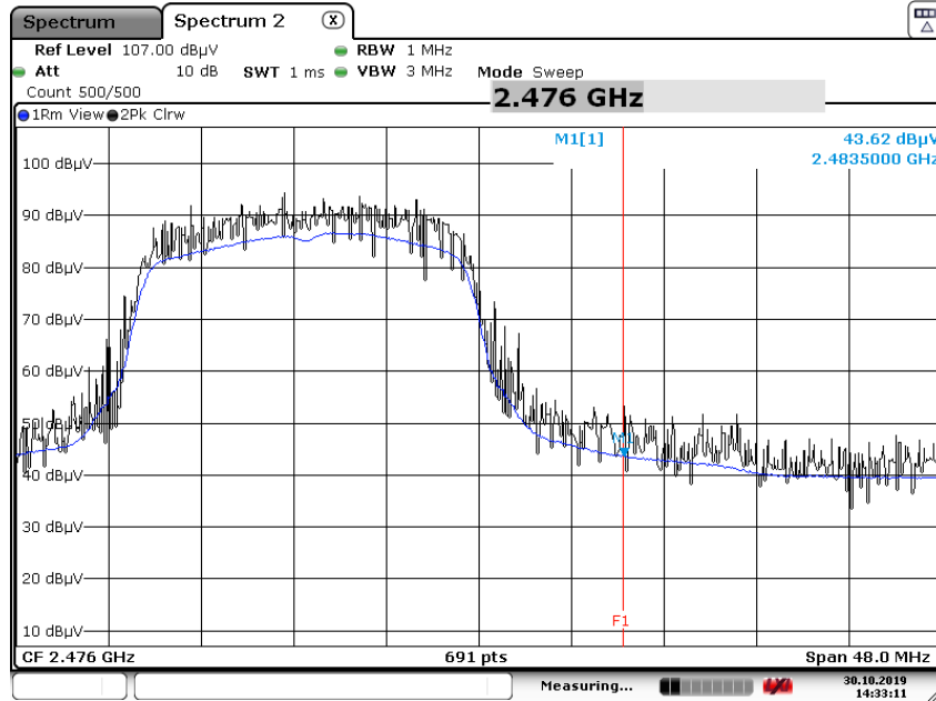
Radiated Restricted Band Edges plot – Average Reading (802.11g_6Mbps Ch.12)
