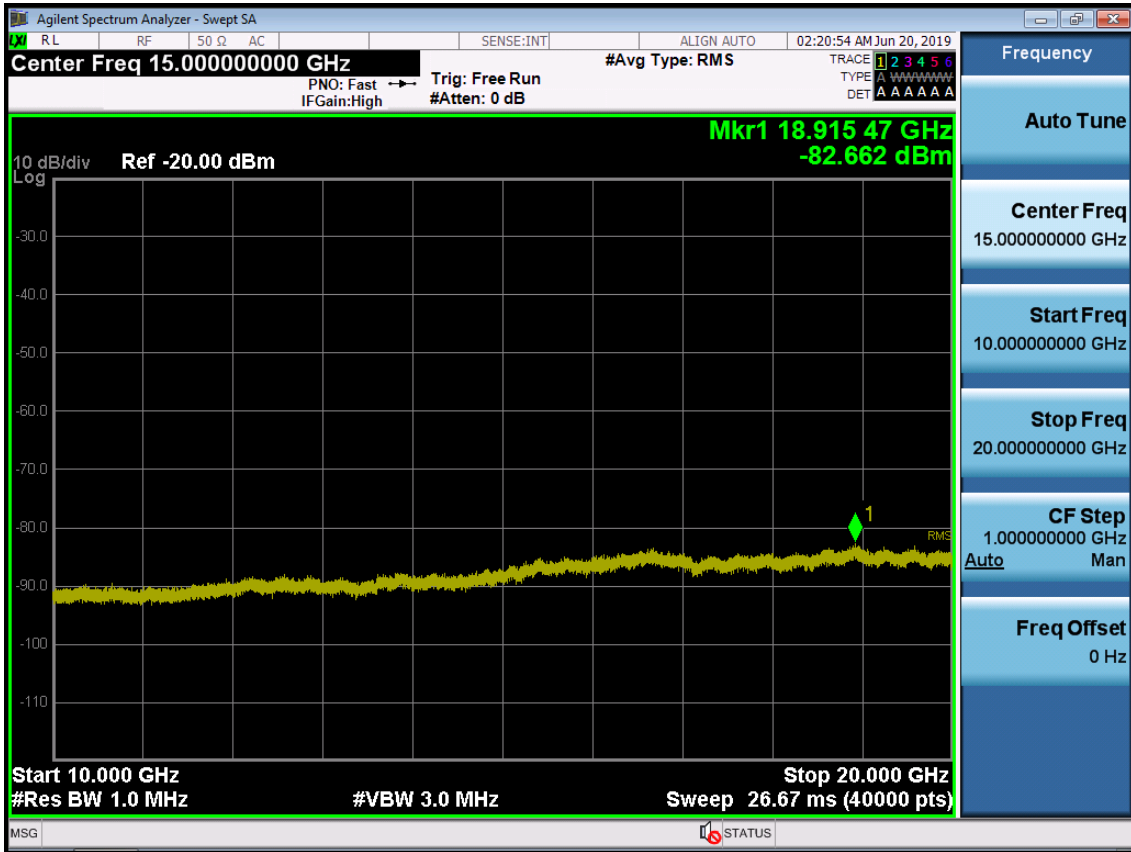
BAND 66. Conducted Spurious Plot_2 (132322ch_1.4MHz_QPSK_RB 1_0)
