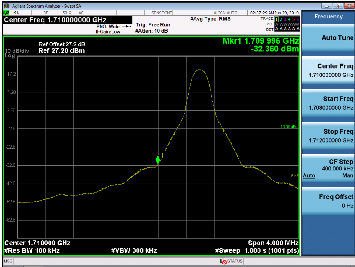
BAND 66. Lower Band Edge Plot (10M BW Ch.132022 QPSK RB 1, Offset 0) -1
