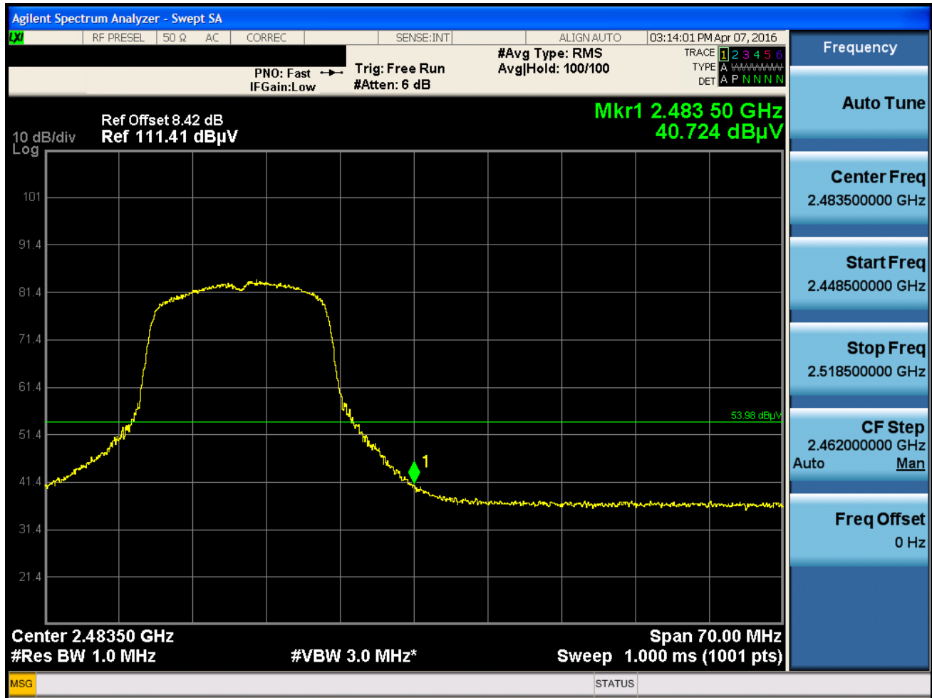
Plot 7-47. Radiated Restricted Upper Band Edge Measurement (Average)
