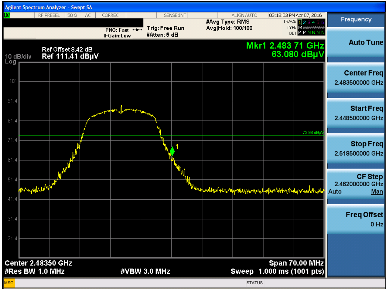
Plot 7-50. Radiated Restricted Upper Band Edge Measurement (Peak)
