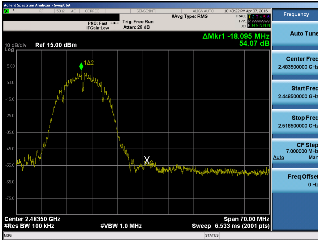
Plot 7-21. Band Edge Plot (802.11b – Ch. 12)
