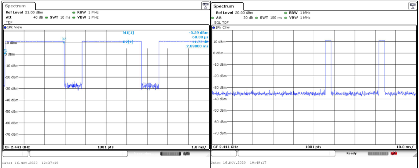
DH5 on time (One Pulse) Plot on Channel 39
