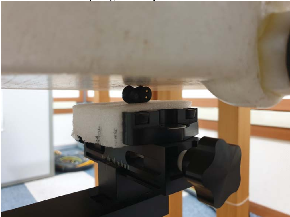
SAR Test Picture(Left), Test separation distance : 0 mm
