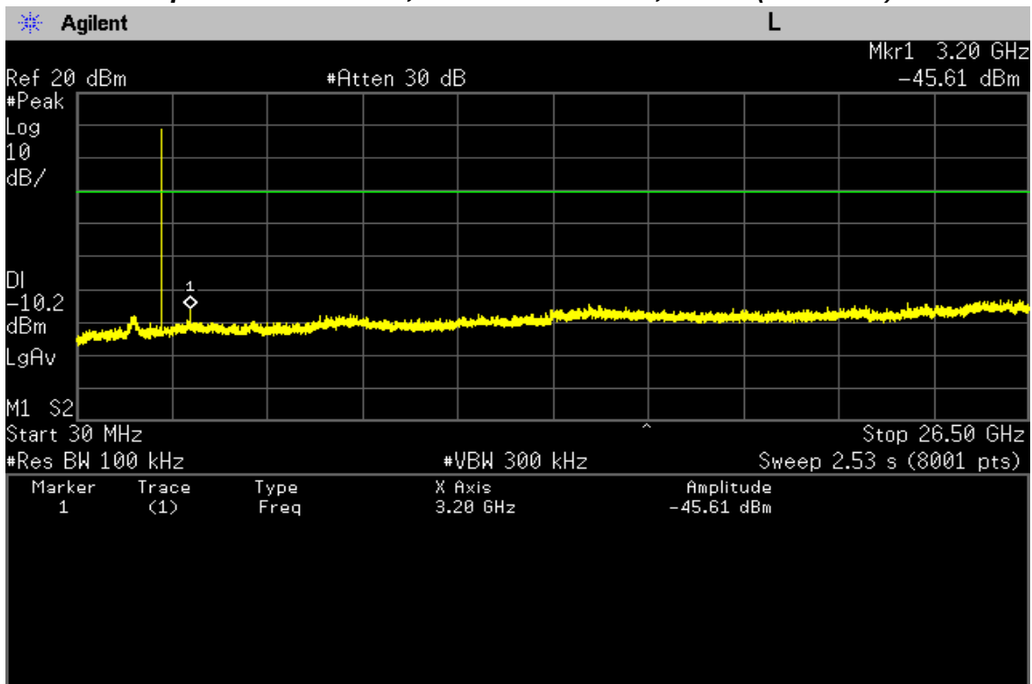
Conducted Spurious Emissions, 30 MHz ~ 26.5 GHz, LE 2M (2402 MHz)
