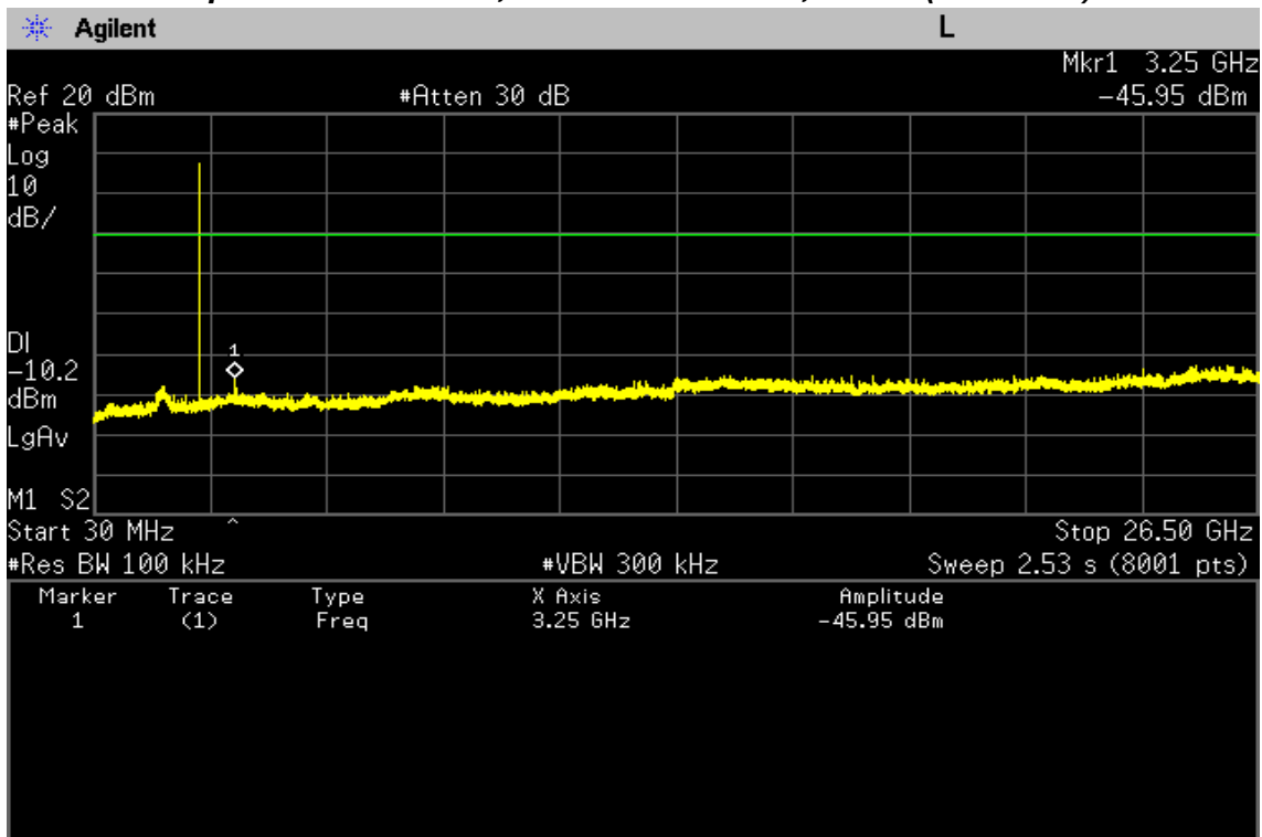
Conducted Spurious Emissions, 30 MHz ~ 26.5 GHz, LE 2M (2440 MHz)
