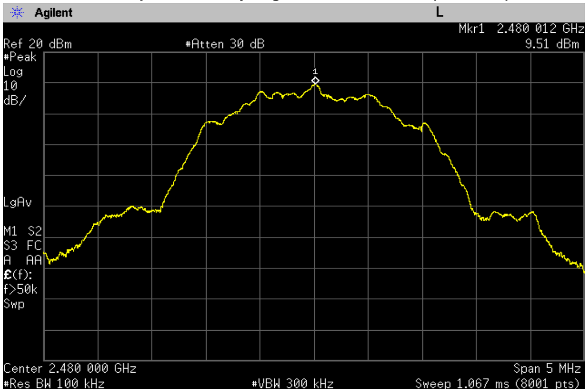
Reference Power Spectral Density, Highest Channel, LE 2M (2480 MHz)
