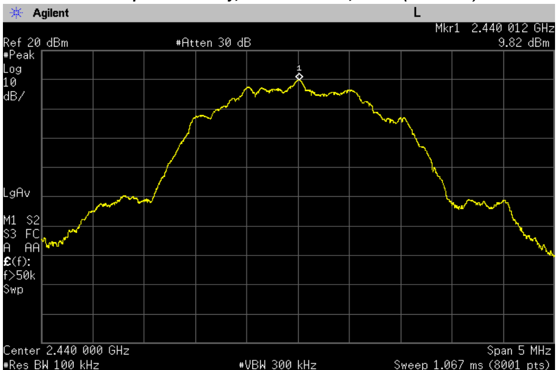
Reference Power Spectral Density, Middle Channel, LE 2M (2440 MHz)
