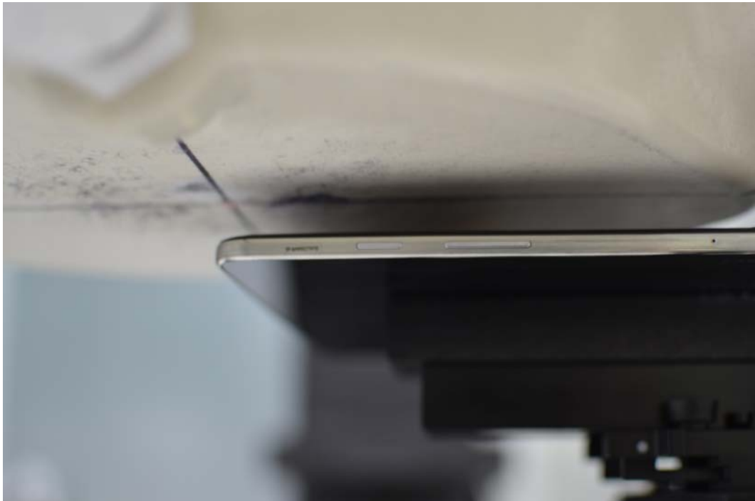
SAR Test Setup Photo 2: Back at 16 mm
