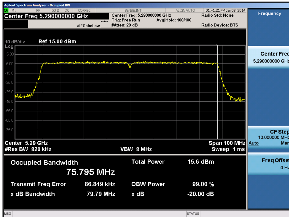
Plot 6-30. 20dB Bandwidth Plot (80MHz BW 802.11n (UNII Band 2A) – Ch. 58)
