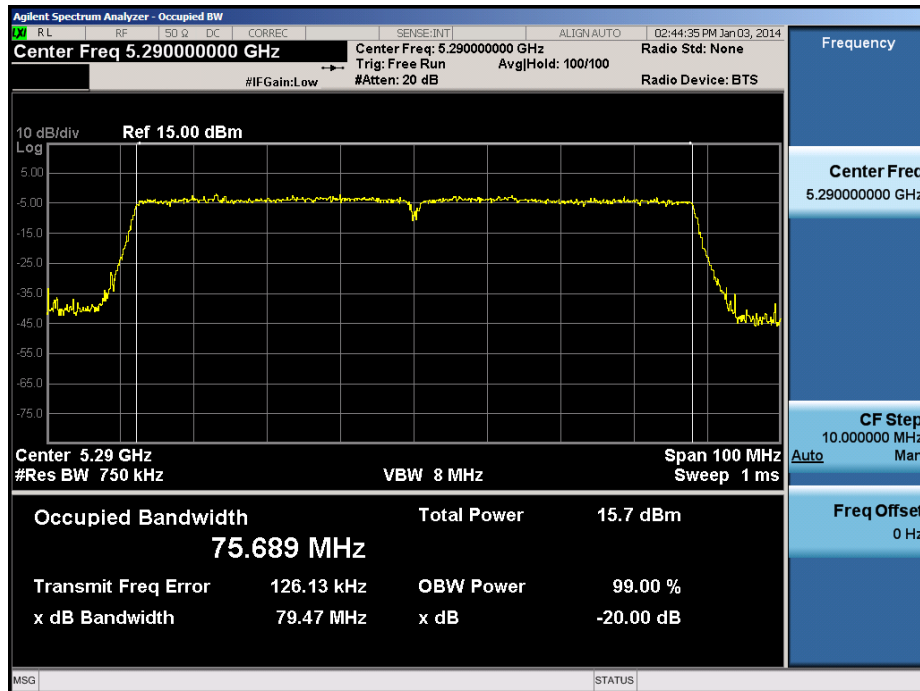
Plot 6-60. 20dB Bandwidth Plot (80MHz BW 802.11n (UNII Band 2A) – Ch. 58)
