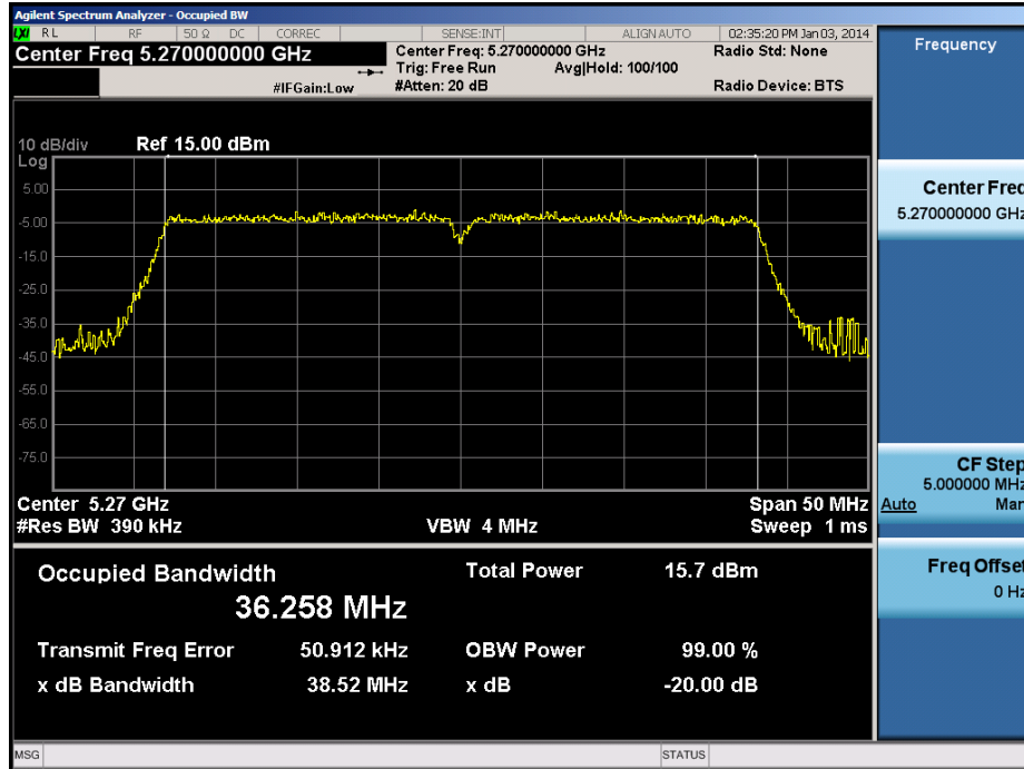
Plot 6-59. 20dB Bandwidth Plot (40MHz BW 802.11n (UNII Band 2A) – Ch. 54)
