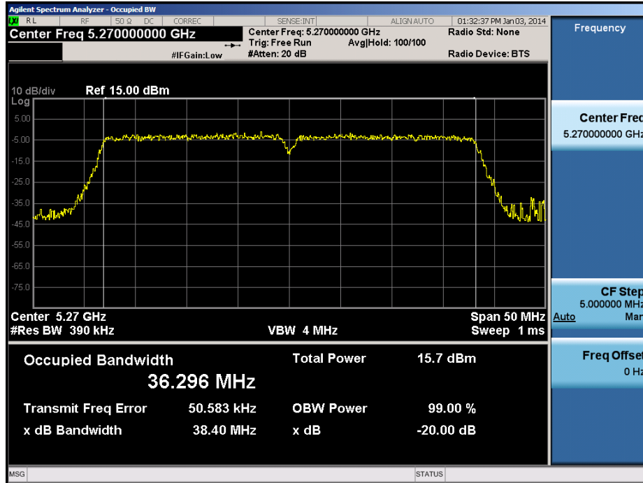
Plot 6-29. 20dB Bandwidth Plot (40MHz BW 802.11n (UNII Band 2A) – Ch. 54)
