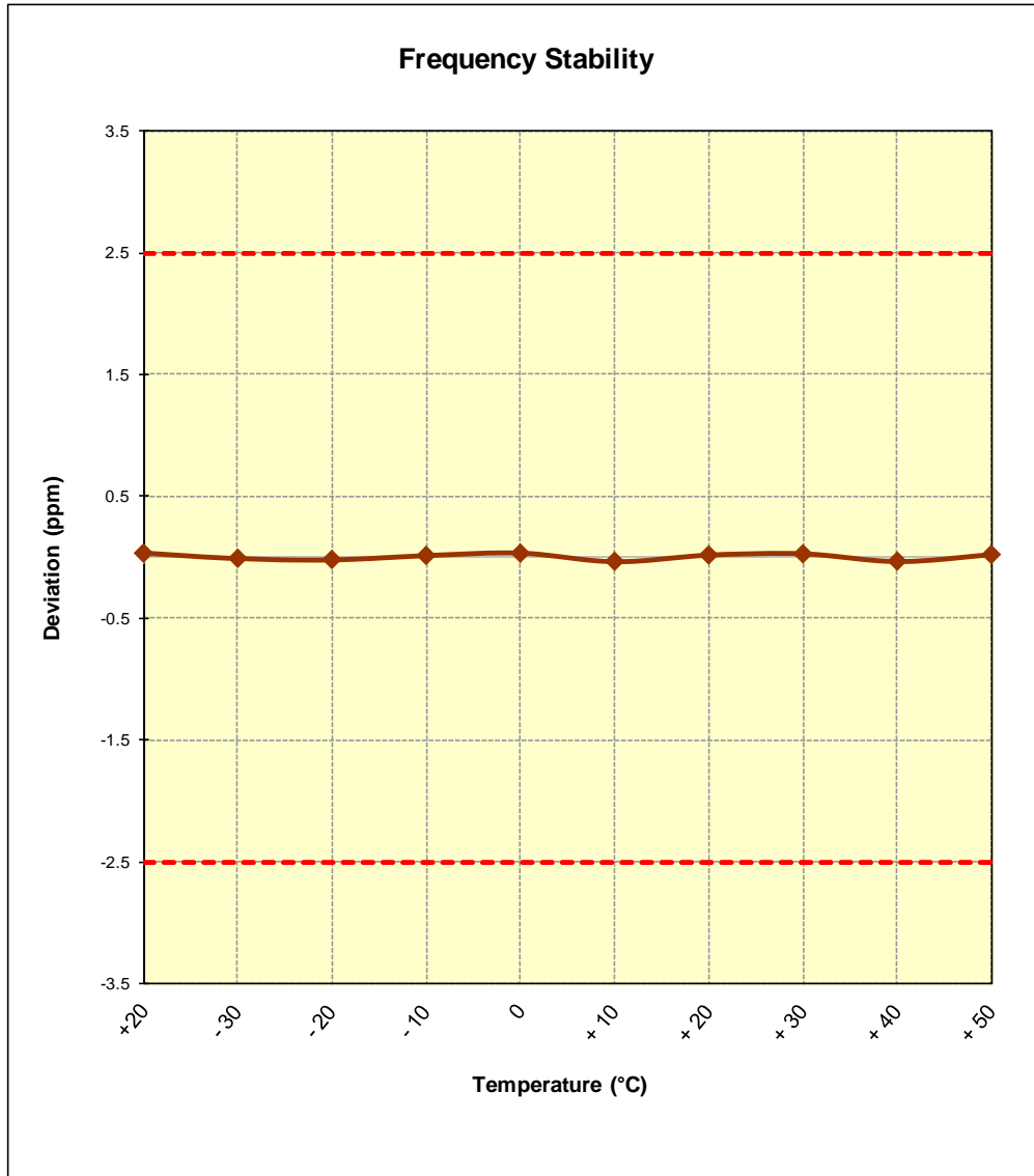
Figure 6-1. Frequency Stability Graph (Band 13)
