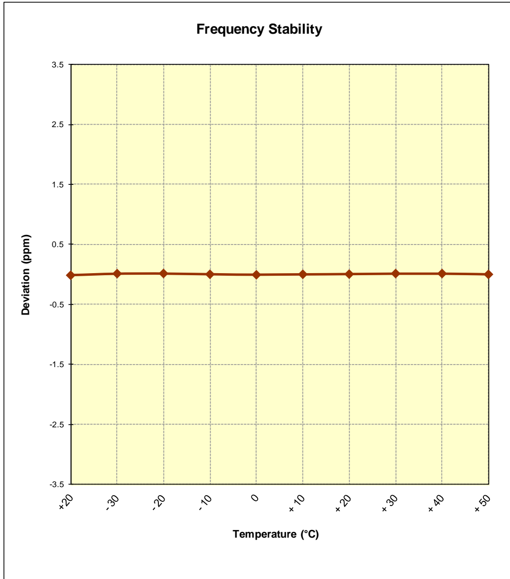
Figure 6-2. Frequency Stability Graph (Band 4)
