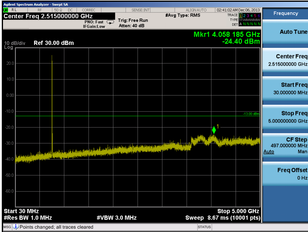
Plot 7-4. Conducted Spurious Plot (10.0MHz QPSK – RB Size 1, RB Offset 0)
