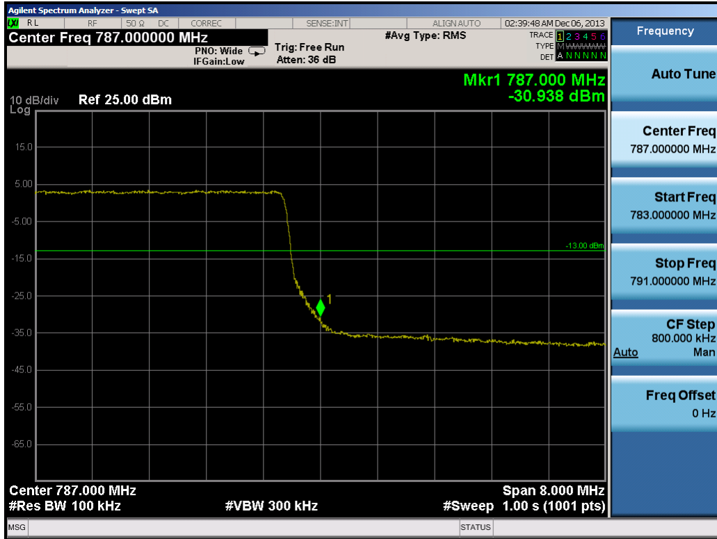
Plot 7-6. Upper Band Edge Plot (10.0MHz QPSK – RB Size 50)
