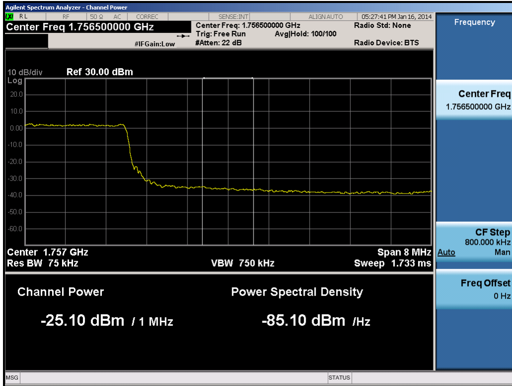
Plot 8-26. Upper Band Edge Plot (10.0MHz QPSK – RB Size 50)
