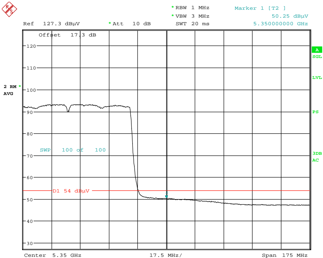
Plot 6-78. Radiated Restricted Upper Band Edge Plot (Average – UNII Band 2)
