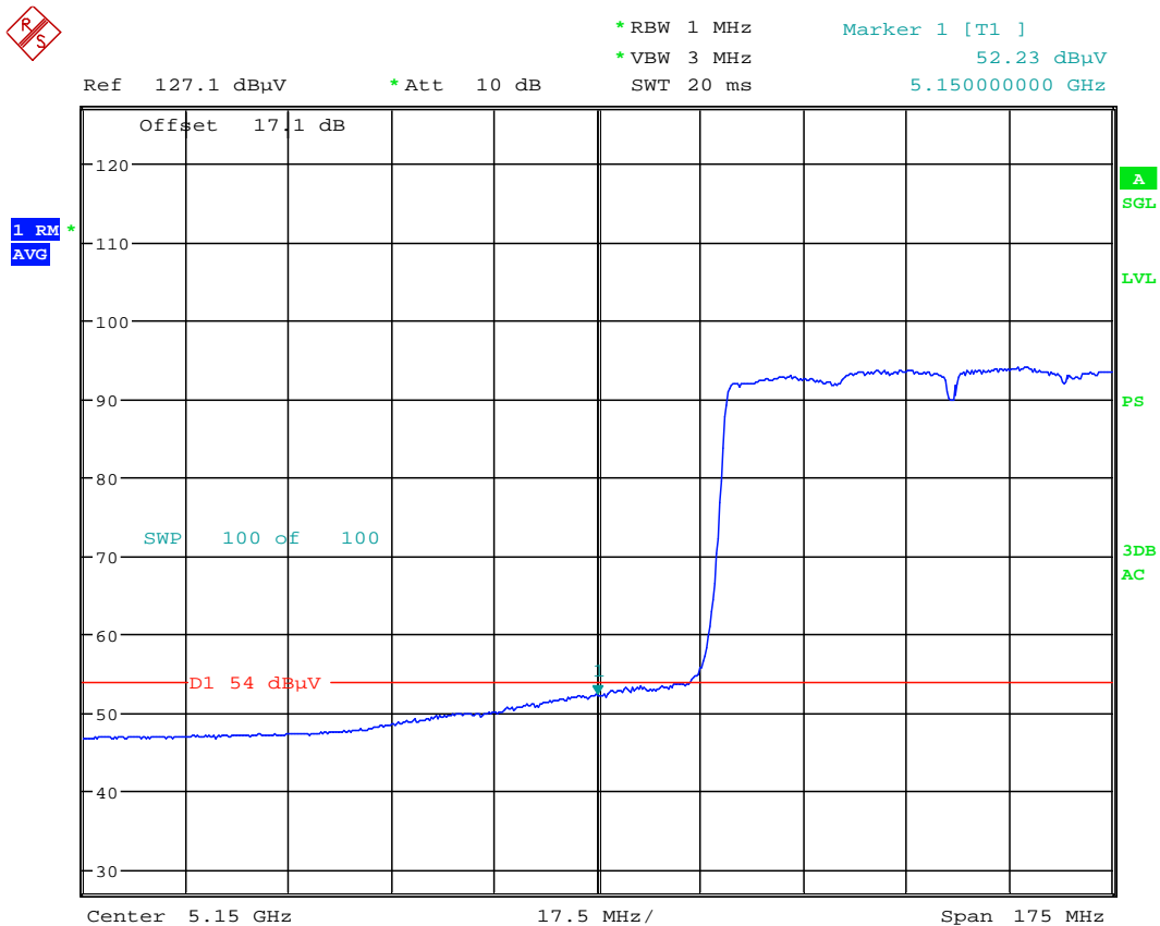
Plot 6-76. Radiated Restricted Lower Band Edge Plot (Average – UNII Band 1)
