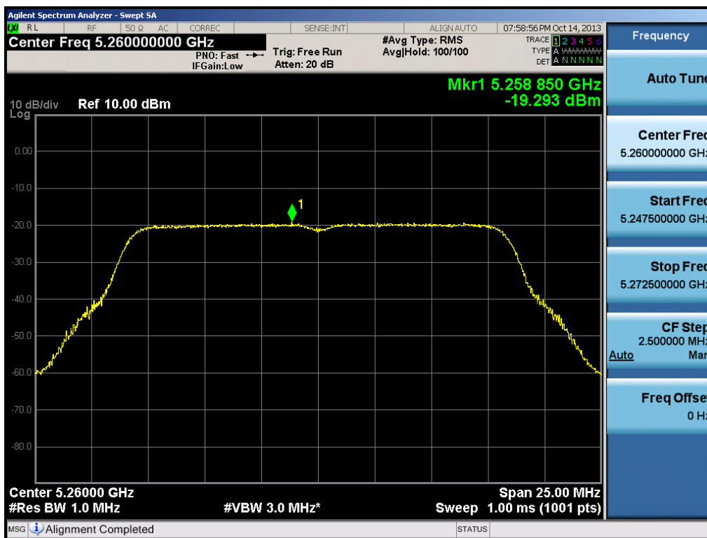
Plot 6-39. Peak Power Spectral Density Plot (802.11a (UNII Band 2) – Ch. 52)
