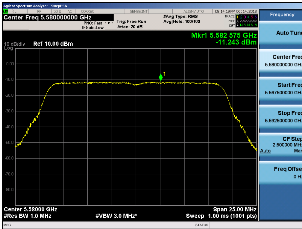
Plot 6-52. Peak Power Spectral Density Plot (20MHz BW 802.11n (UNII Band 3) – Ch. 116)
