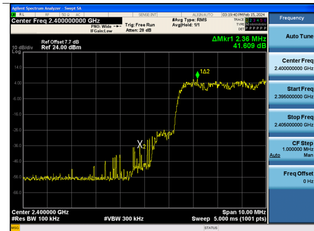
\pi/4 DQPSK Lower Band Edge(Ch. 0)
