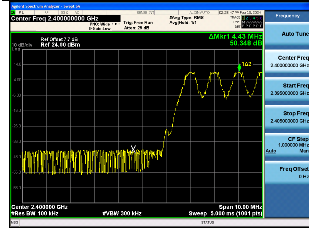
8DPSK Lower Band Edge(Ch. 0)
