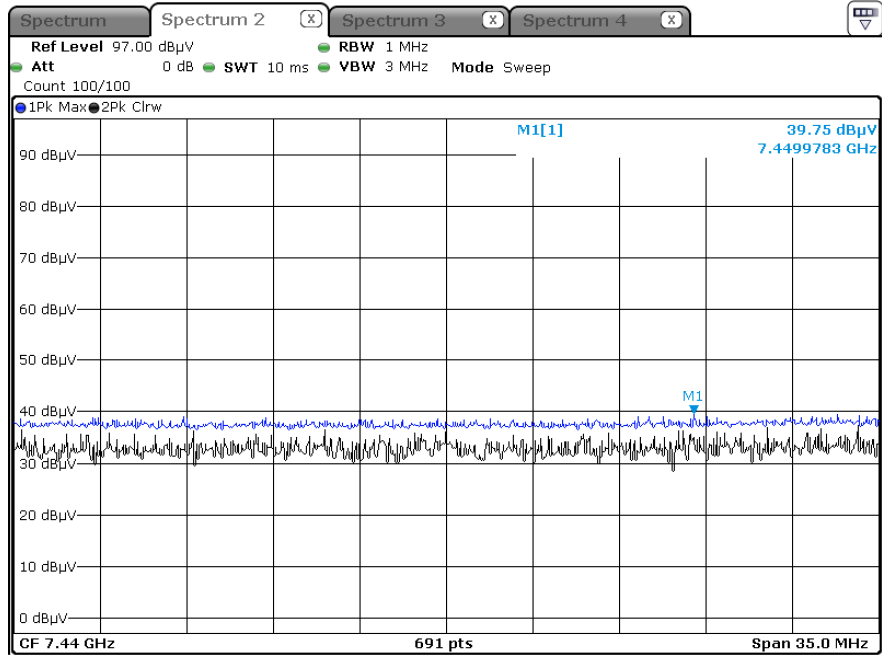
Radiated Spurious Emissions plot – Average & Peak Result (GFSK, Ch.78 3rd Harmonic, Z-H)
