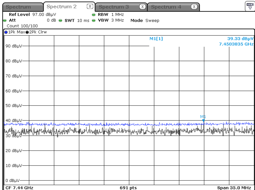
Radiated Spurious Emissions plot – Average & Peak Result ( \pi/4 DQPSK, Ch.78 3rd Harmonic, Z-H)
