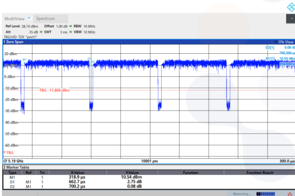
802.11ac_VHT40
