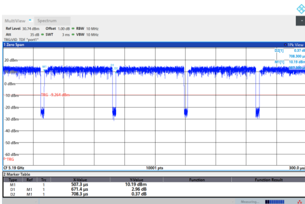
802.11ac_VHT40
