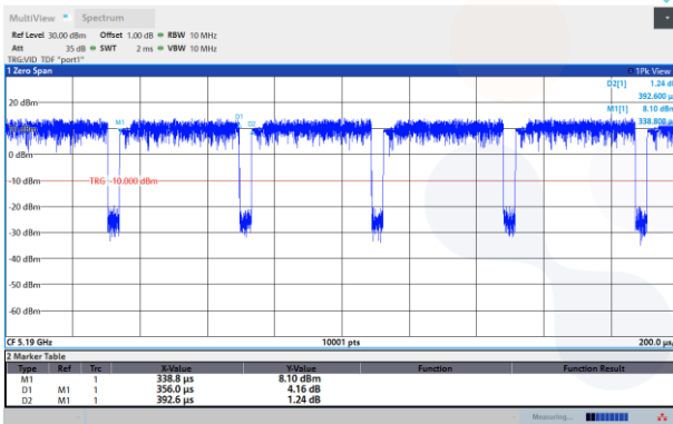
802.11ac_VHT40
