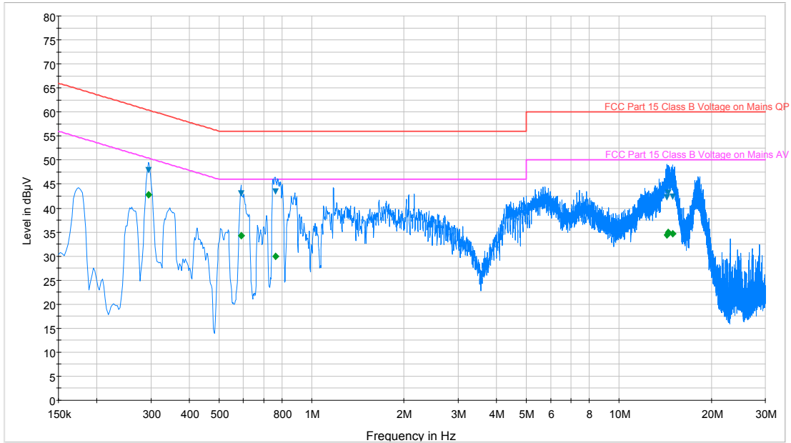
Plot 6-21. Line Conducted Plot with Bluetooth LE (N)
