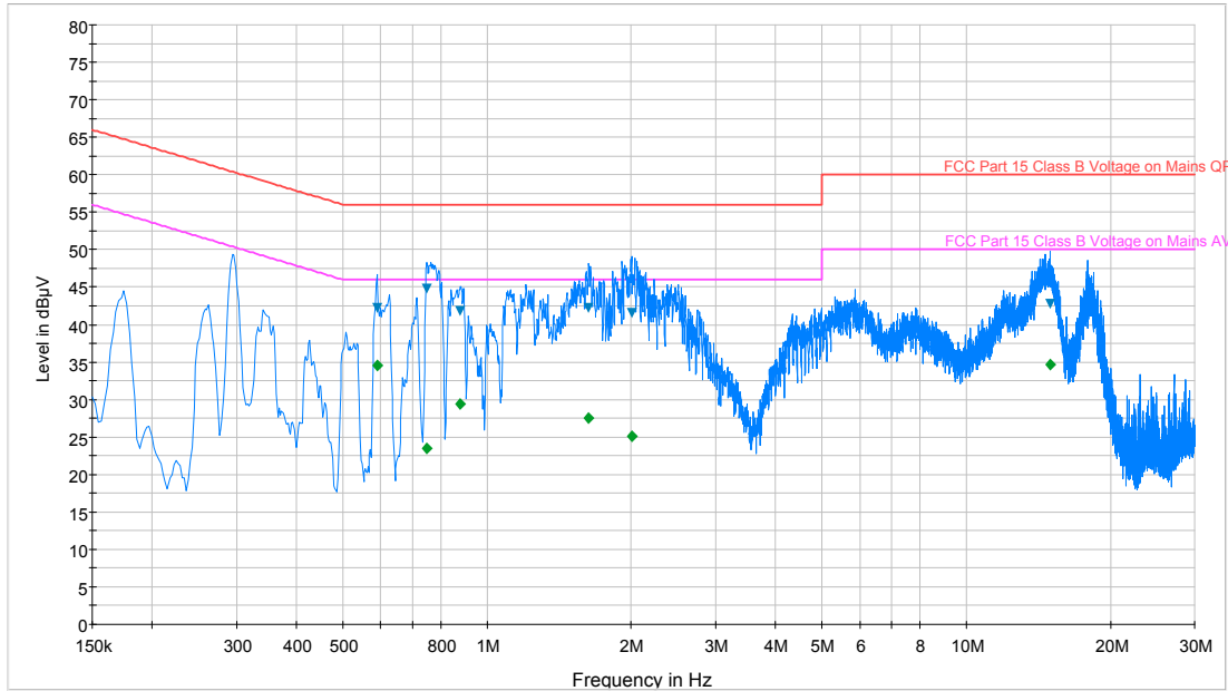
— FCC Part 15 Class B Voltage on Mains QP.LimitLine — FCC Part 15 Class B Voltage on Mains AV.LimitLine — Preview Result 1-PK+ ◆ Final Result 2-AVG
