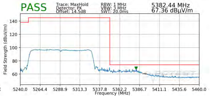
Plot 7-101. Radiated Upper Band Edge Plot – SISO (Peak – UNII Band 2A)
