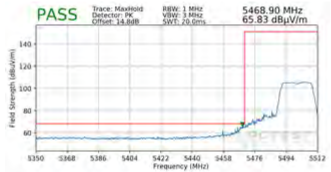
Plot 7-89. Radiated Lower Band Edge Plot SISO ANT1 (Peak – UNII Band 2C)
