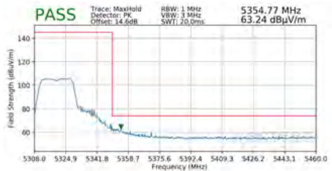
Plot 7-87. Radiated Upper Band Edge Plot SISO ANT1 (Peak – UNII Band 2A)
