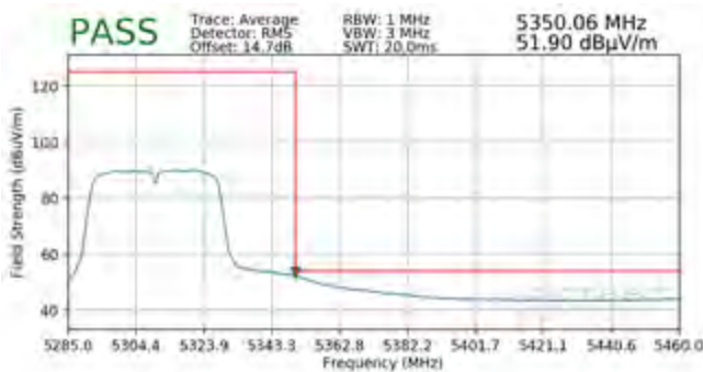
Plot 7-93. Radiated Upper Band Edge Plot SISO ANT1 (Average – UNII Band 2A)
