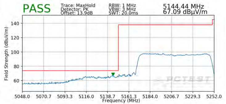
Plot 7-99. Radiated Lower Band Edge Plot – SISO (Peak – UNII Band 1)
