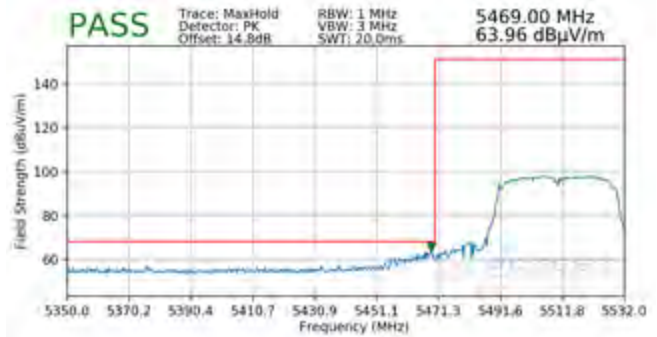
Plot 7-96. Radiated Lower Band Edge Plot SISO ANT1 (Peak – UNII Band 2C)
