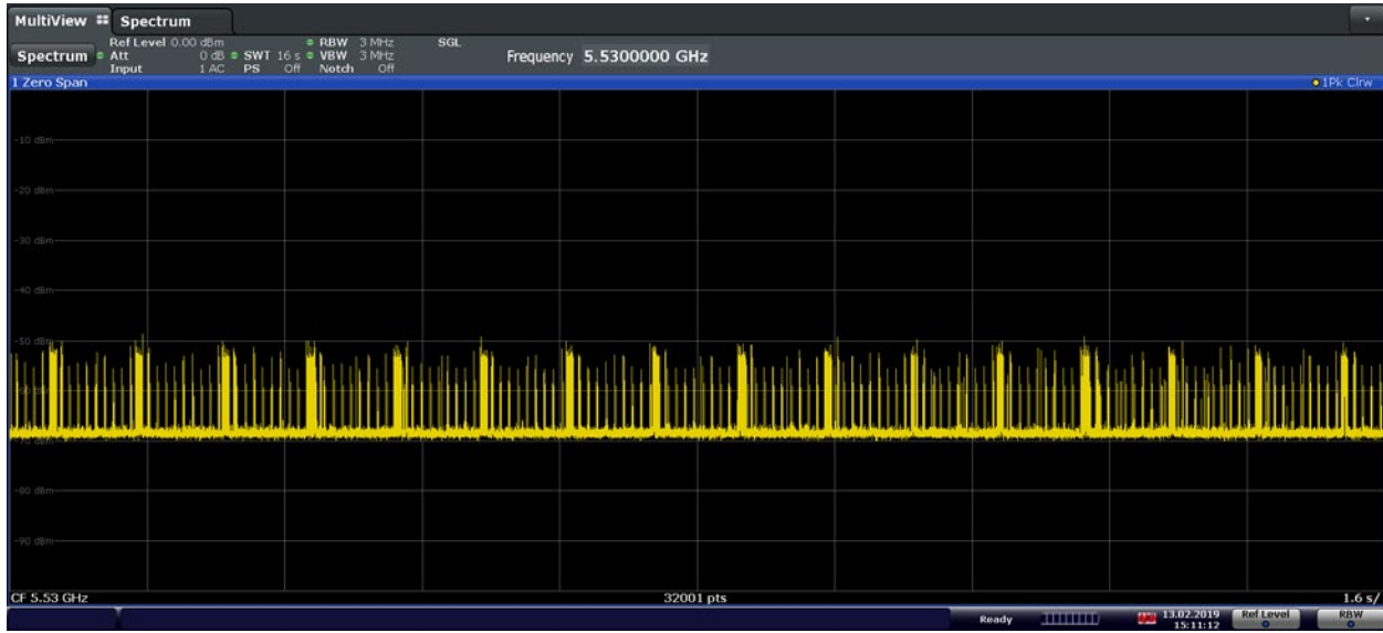
Figure 9-5. 5530MHz - Channel Loading - (80MHz)
