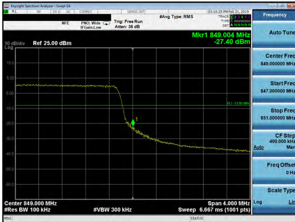
Plot 7-109. Upper Band Edge Plot (Band 5 - 5.0MHz QPSK - Full RB Configuration)
