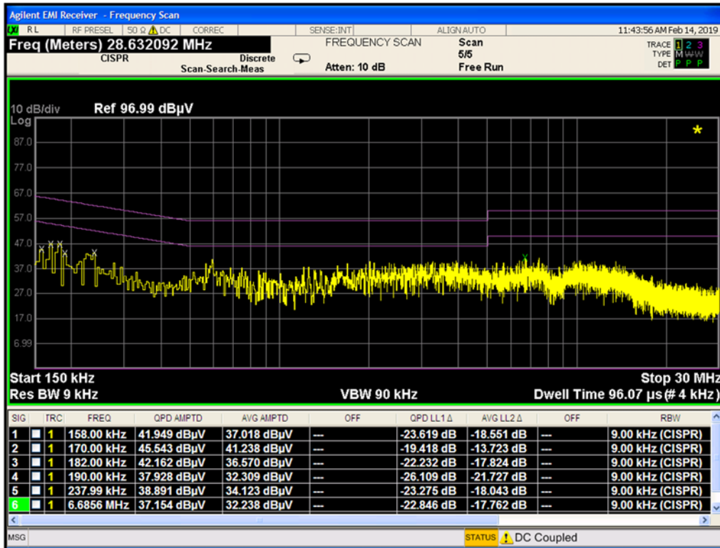
Plot 7-31. Line Conducted Plot with Bluetooth LE (L1)
