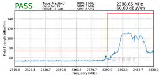
Plot 7-106. Radiated Restricted Lower Band Edge Measurement MIMO (Peak – 106 Tones)
