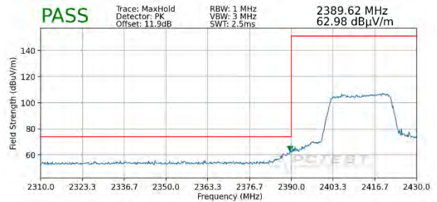
Plot 7-110. Radiated Restricted Lower Band Edge Measurement MIMO (Peak – 242 Tones)
