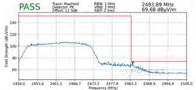
Plot 7-104. Radiated Restricted Upper Band Edge Measurement SISO ANT2 (Peak – 242 Tones)
