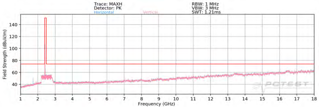
Plot 7-89. Radiated Spurious Plot above 1GHz SISO ANT2 (802.11b – Ch. 1)
