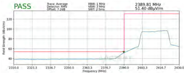
Plot 7-97. Radiated Restricted Lower Band Edge Measurement SISO ANT1 (Average)
