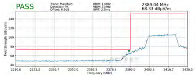
Plot 7-98. Radiated Restricted Lower Band Edge Measurement SISO ANT1 (Peak)
