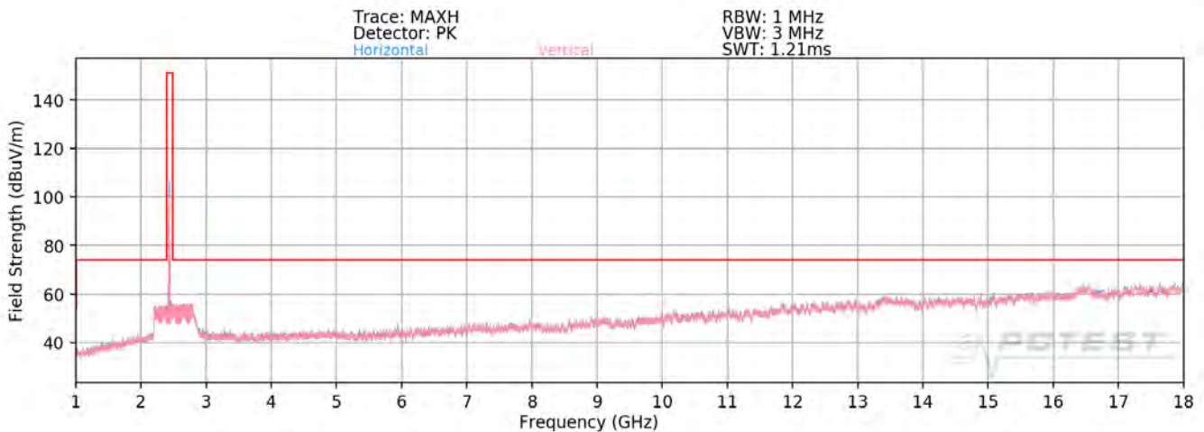
Plot 7-90. Radiated Spurious Plot above 1GHz SISO ANT2 (802.11b – Ch. 6)
