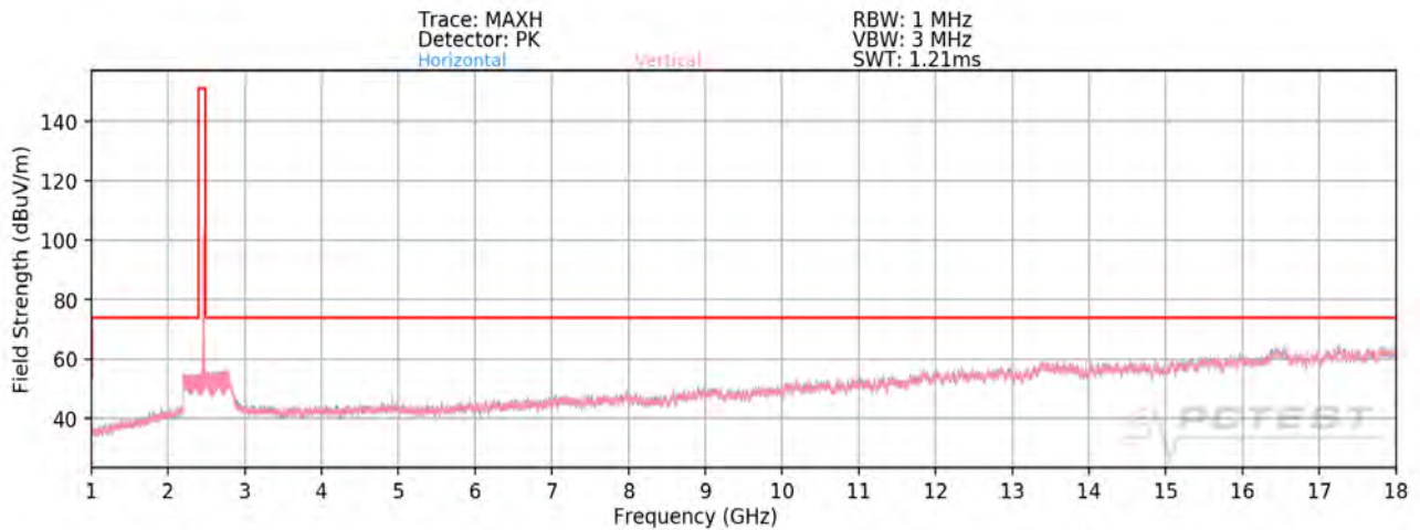
Plot 7-87. Radiated Spurious Plot above 1GHz SISO ANT1 (802.11b – Ch. 11)
