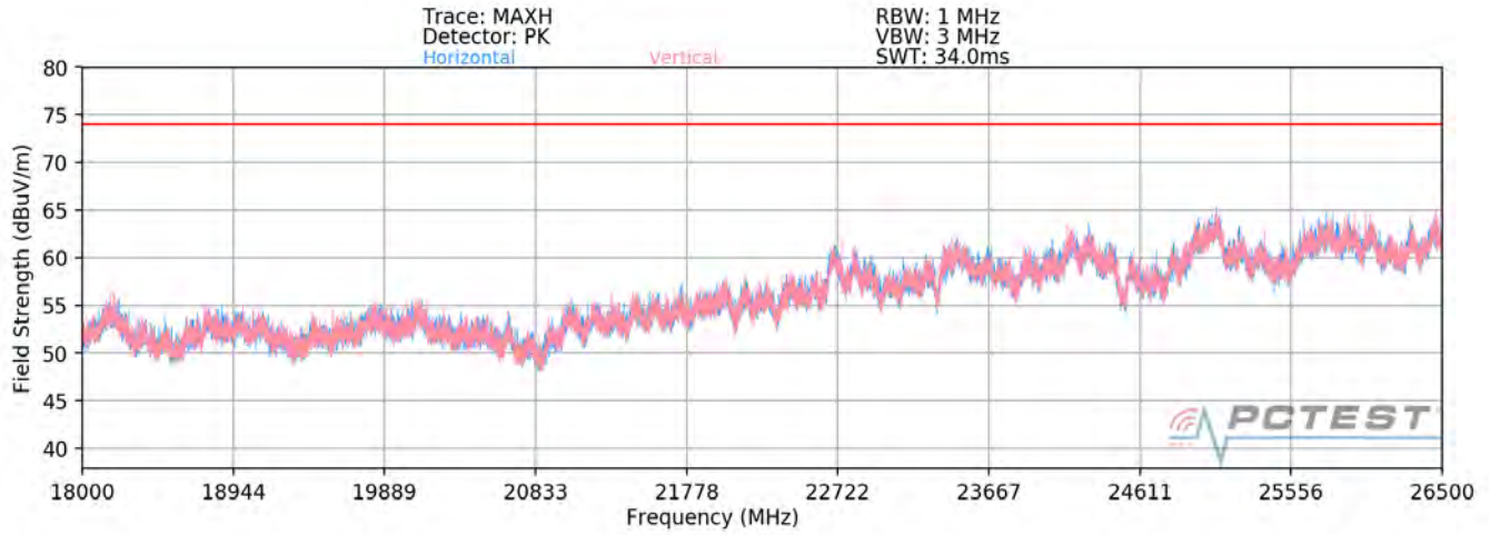
Plot 7-88. Radiated Spurious Plot above 18GHz SISO ANT1
