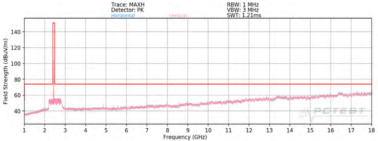
Plot 7-86. Radiated Spurious Plot above 1GHz SISO ANT1 (802.11b – Ch. 6)
