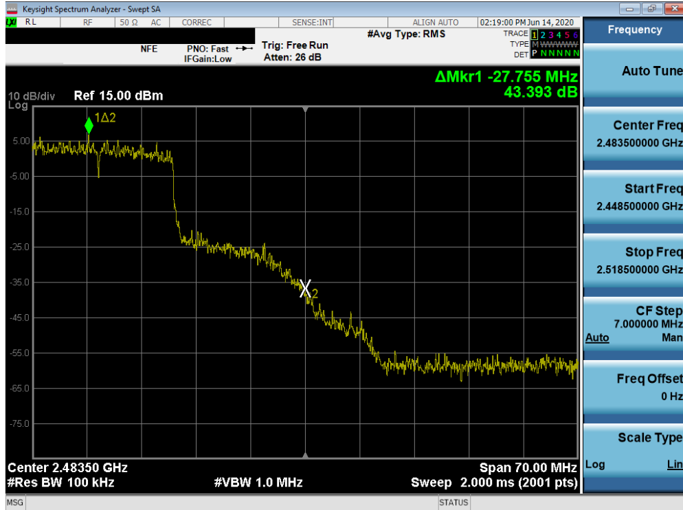
Plot 7-71. Band Edge Plot SISO ANT2 (802.11ax (2.4GHz) – Ch. 10)
