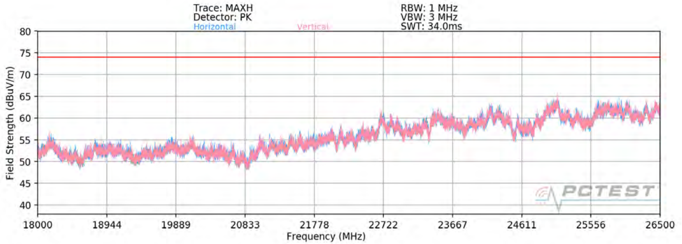
Plot 7-92. Radiated Spurious Plot above 18GHz SISO ANT2
