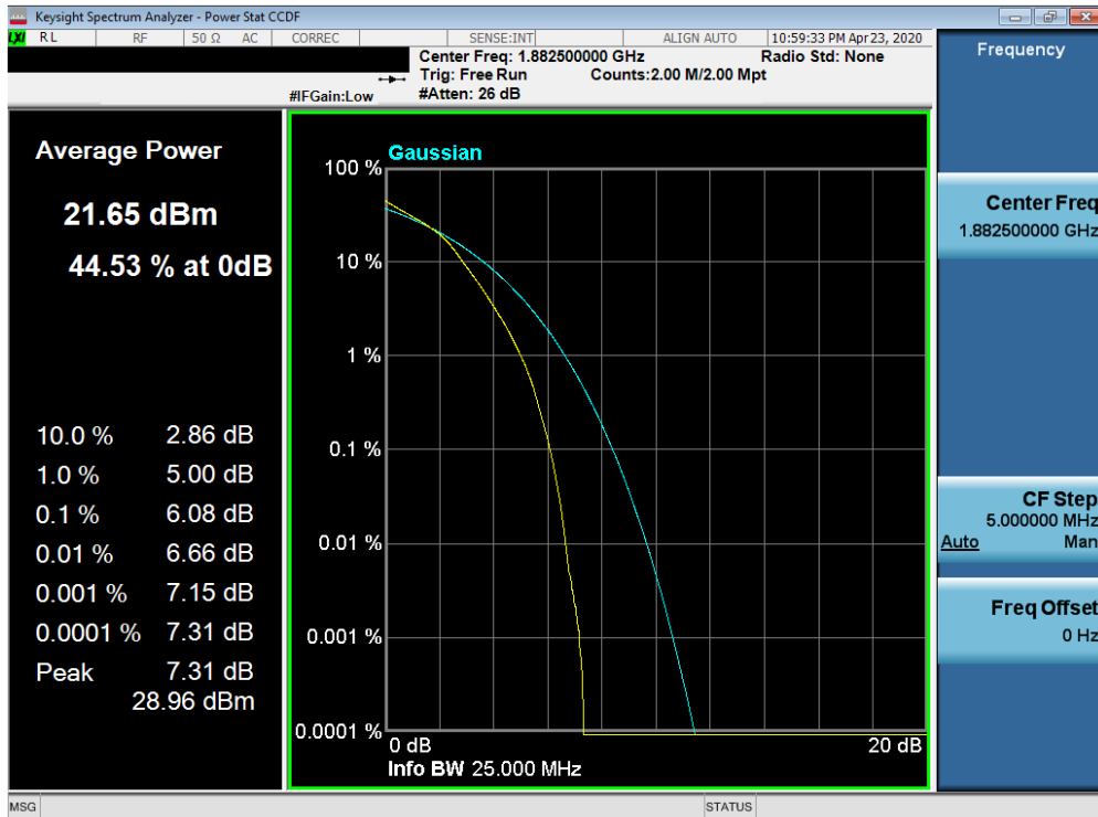
Plot 7-566. PAR Plot (Band 25/2 - 20.0MHz 16-QAM - Full RB Configuration)
