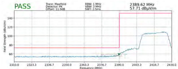
Plot 7-116. Radiated Restricted Lower Band Edge Measurement MIMO (Peak)
