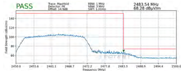
Plot 7-112. Radiated Restricted Upper Band Edge Measurement SISO ANT2 (Peak)
