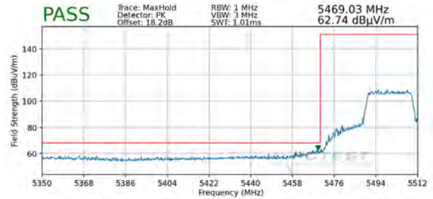
Plot 7-287. Radiated Lower Band Edge Plot SISO ANT1 (Peak – UNII Band 2C)
