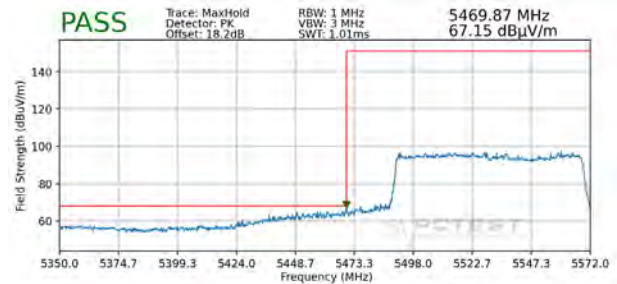
Plot 7-301. Radiated Lower Band Edge Plot SISO ANT1 (Peak – UNII Band 2C)
