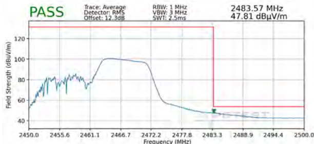
Plot 7-107. Radiated Restricted Upper Band Edge Measurement MIMO (Average – 106 Tones)
