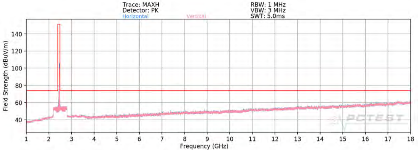
Plot 7-70. Radiated Spurious Plot above 1GHz SISO ANT2 (802.11ax OFDMA – 242 Tones – Ch. 11) SISO Antenna-2 Radiated Spurious Emissions Measurements (Above 18GHz) §15.209; RSS-Gen [8.9]
