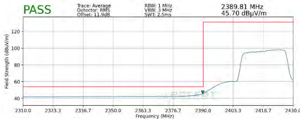
Plot 7-111. Radiated Restricted Lower Band Edge Measurement MIMO (Average – 242 Tones)
