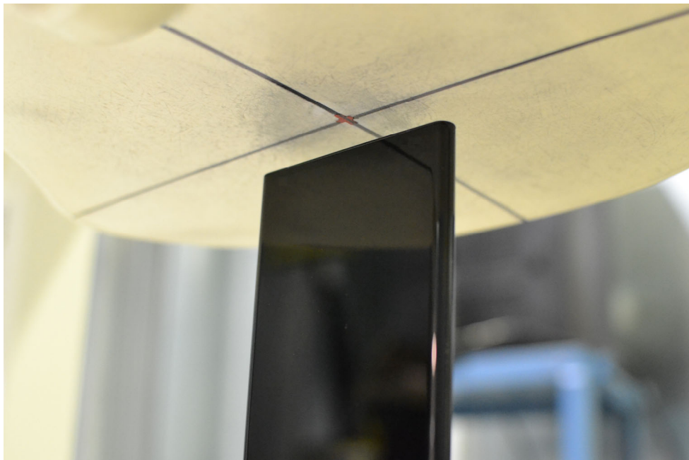
SAR Test Setup Photo 14 – Bottom Side at 10 mm
