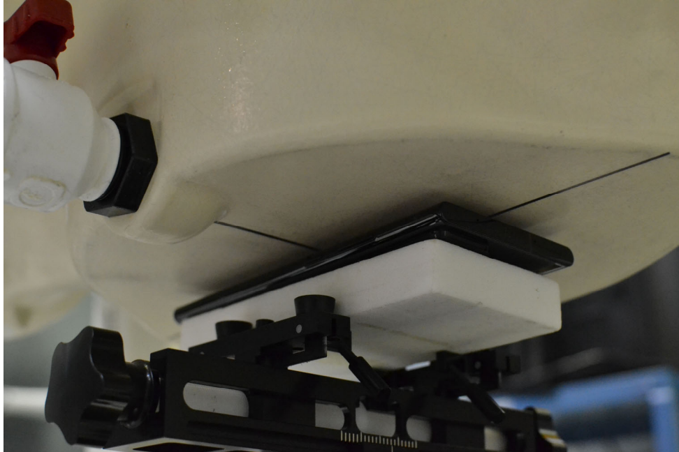
SAR Test Setup Photo 9 – Front Side at 6 mm
