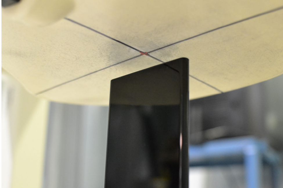
SAR Test Setup Photo 13 – Bottom Side at 13 mm
