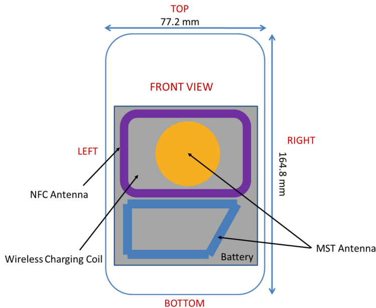
Figure E-2 NFC/MST Antenna and Wireless Charging Coil Locations
