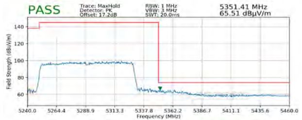
Plot 7-299. Radiated Upper Band Edge Plot SISO ANT1 (Peak – UNII Band 2A)
