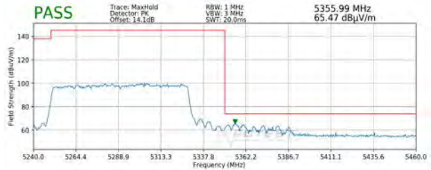
Plot 7-341. Radiated Upper Band Edge Plot MIMO (Peak – UNII Band 2A)
