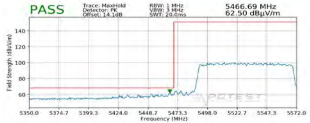
Plot 7-322. Radiated Lower Band Edge Plot SISO ANT2 (Peak – UNII Band 2C)
