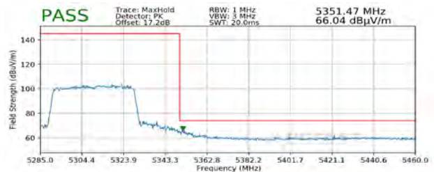
Plot 7-292. Radiated Upper Band Edge Plot SISO ANT1 (Peak – UNII Band 2A)
