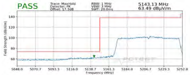
Plot 7-318. Radiated Lower Band Edge Plot SISO ANT2 (Peak – UNII Band 1)
