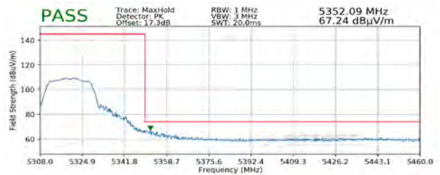
Plot 7-285. Radiated Upper Band Edge Plot SISO ANT1 (Peak – UNII Band 2A)
