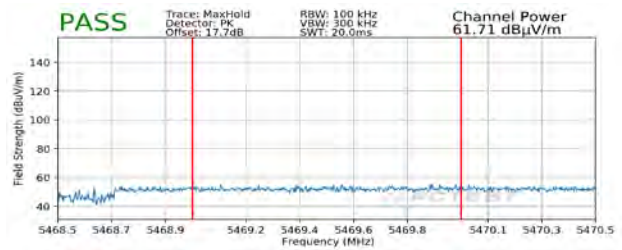
Plot 7-294. Radiated Lower Band Edge Plot SISO ANT1 (Peak – UNII Band 2C)
