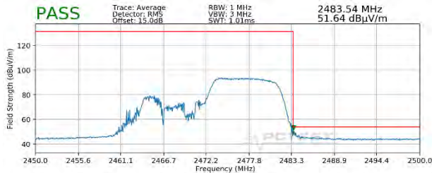
Plot 7-127. Radiated Restricted Upper Band Edge Measurement MIMO (Average – 106 Tones)
