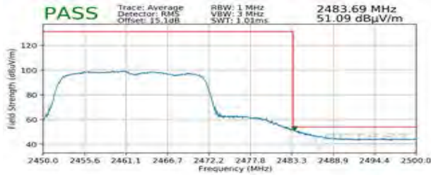
Plot 7-135. Radiated Restricted Upper Band Edge Measurement MIMO (Average – 242 Tones)
