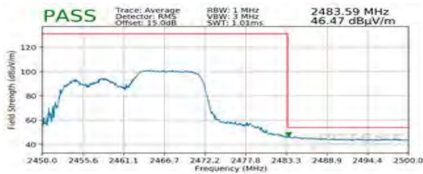
Plot 7-123. Radiated Restricted Upper Band Edge Measurement MIMO (Average – 106 Tones)
