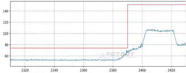
Plot 7-90. Radiated Restricted Lower Band Edge Measurement SISO ANT1 (Peak – 242 Tones)
