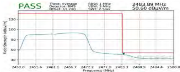
Plot 7-115. Radiated Restricted Upper Band Edge Measurement SISO ANT2 (Average – 242 Tones)
