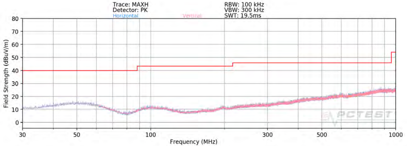
Plot 7-141. Radiated Spurious Plot below 1GHz MIMO (106 Tones)
