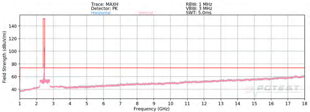
Plot 7-70. Radiated Spurious Plot above 1GHz SISO ANT2 (802.11ax OFDMA – 242 Tones – Ch. 11)
