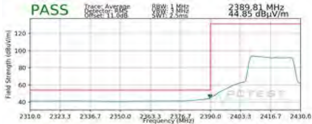
Plot 7-111. Radiated Restricted Lower Band Edge Measurement SISO ANT2 (Average – 242 Tones)
