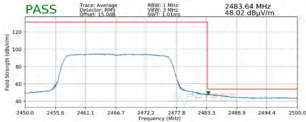
Plot 7-137. Radiated Restricted Upper Band Edge Measurement MIMO (Average – 242 Tones)
