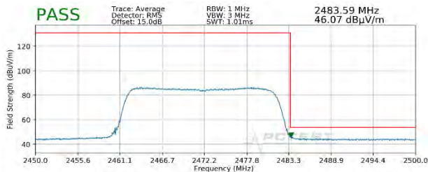
Plot 7-99. Radiated Restricted Upper Band Edge Measurement SISO ANT1 (Average – 242 Tones)
