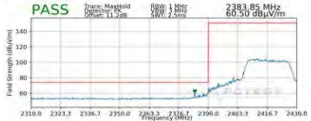
Plot 7-112. Radiated Restricted Lower Band Edge Measurement SISO ANT2 (Peak – 242 Tones)
