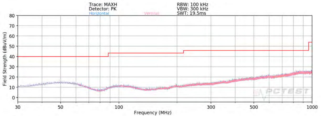
Plot 7-142. Radiated Spurious Plot below 1GHz MIMO (242 Tones)
