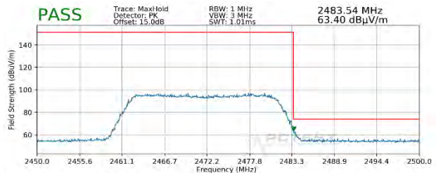
Plot 7-100. Radiated Restricted Upper Band Edge Measurement SISO ANT1 (Peak – 242 Tones)
