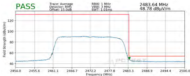
Plot 7-139. Radiated Restricted Upper Band Edge Measurement MIMO (Average – 242 Tones)
