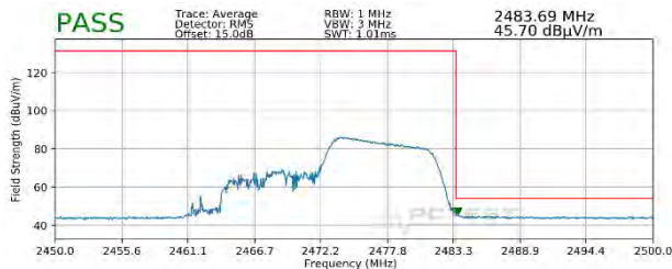
Plot 7-107. Radiated Restricted Upper Band Edge Measurement SISO ANT2 (Average – 106 Tones)
