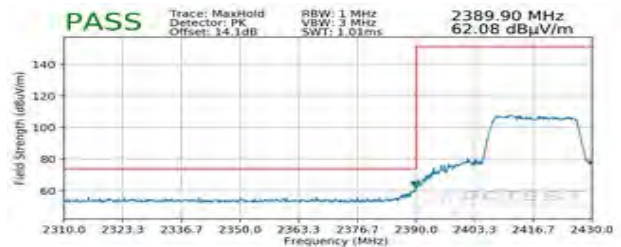
Plot 7-132. Radiated Restricted Lower Band Edge Measurement MIMO (Peak – 242 Tones)
