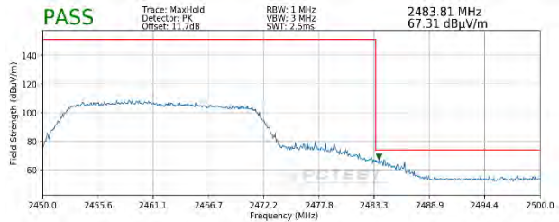
Plot 7-96. Radiated Restricted Upper Band Edge Measurement SISO ANT1 (Peak – 242 Tones)
