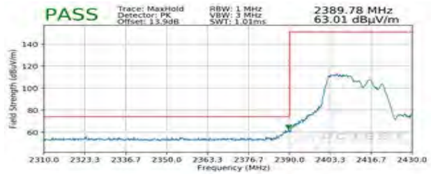
Plot 7-122. Radiated Restricted Lower Band Edge Measurement MIMO (Peak – 106 Tones)
