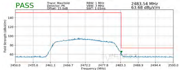
Plot 7-120. Radiated Restricted Upper Band Edge Measurement SISO ANT2 (Peak – 242 Tones)
