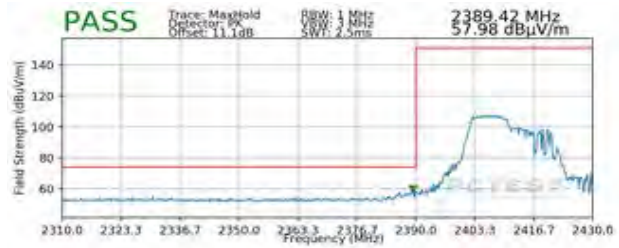
Plot 7-102. Radiated Restricted Lower Band Edge Measurement SISO ANT2 (Peak – 106 Tones)
