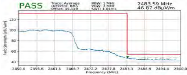
Plot 7-133. Radiated Restricted Upper Band Edge Measurement MIMO (Average – 242 Tones)
