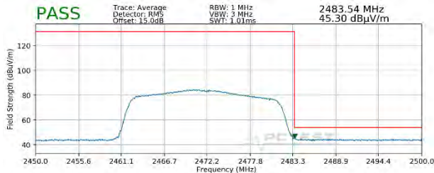
Plot 7-119. Radiated Restricted Upper Band Edge Measurement SISO ANT2 (Average – 242 Tones)
