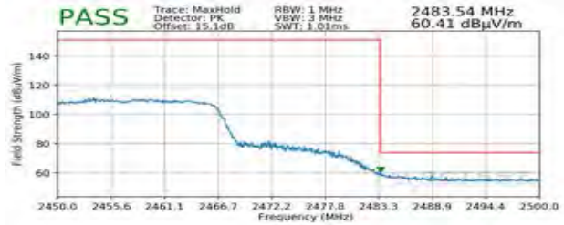
Plot 7-134. Radiated Restricted Upper Band Edge Measurement MIMO (Peak – 242 Tones)
