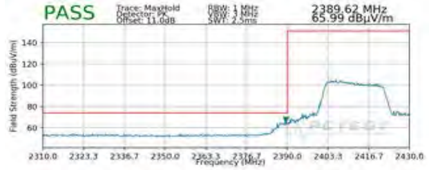
Plot 7-110. Radiated Restricted Lower Band Edge Measurement SISO ANT2 (Peak – 242 Tones)
