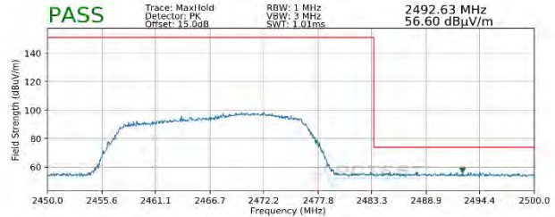
Plot 7-118. Radiated Restricted Upper Band Edge Measurement SISO ANT2 (Peak – 242 Tones)
