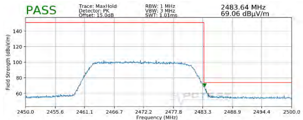
Plot 7-140. Radiated Restricted Upper Band Edge Measurement MIMO (Peak – 242 Tones)
