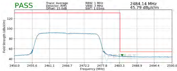
Plot 7-97. Radiated Restricted Upper Band Edge Measurement SISO ANT1 (Average – 242 Tones)
