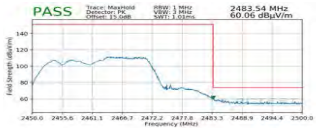
Plot 7-124. Radiated Restricted Upper Band Edge Measurement MIMO (Peak – 106 Tones)
