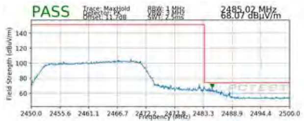
Plot 7-116. Radiated Restricted Upper Band Edge Measurement SISO ANT2 (Peak – 242 Tones)
