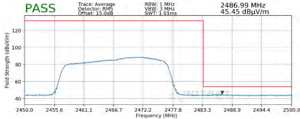
Plot 7-117. Radiated Restricted Upper Band Edge Measurement SISO ANT2 (Average – 242 Tones)
