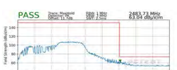
Plot 7-104. Radiated Restricted Upper Band Edge Measurement SISO ANT2 (Peak – 106 Tones)
