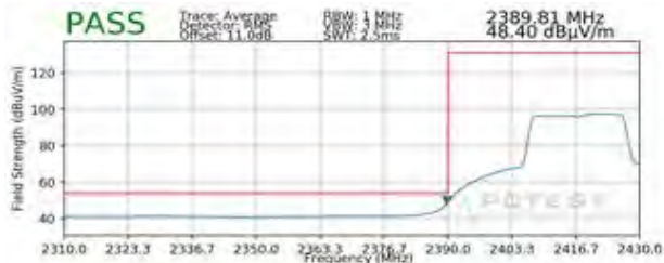
Plot 7-91. Radiated Restricted Lower Band Edge Measurement SISO ANT1 (Average – 242 Tones)
