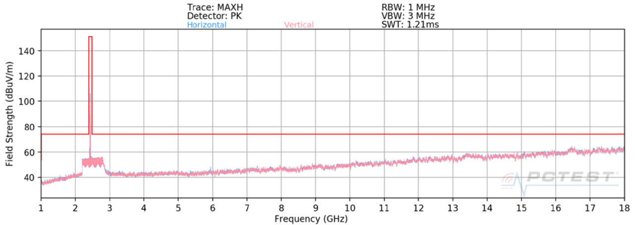
Plot 7-106. Radiated Spurious Plot above 1GHz SISO ANT2 (802.11b – Ch. 6)
