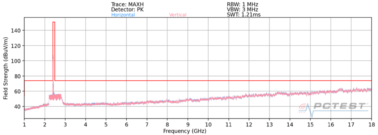
Plot 7-109. Radiated Spurious Plot above 1GHz MIMO/CDD (802.11g – Ch. 1)
