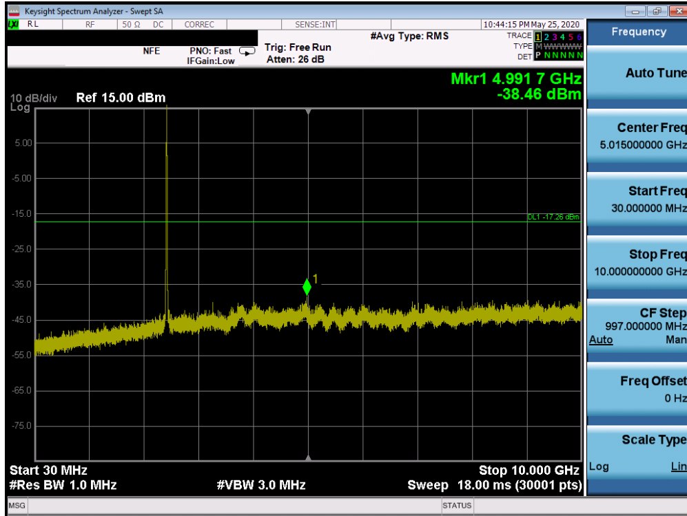
Plot 7-97. Conducted Spurious Plot SISO ANT2 (802.11b – Ch. 6)
