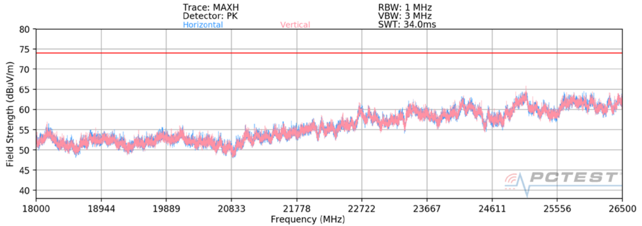
Plot 7-108. Radiated Spurious Plot above 18GHz SISO ANT2
