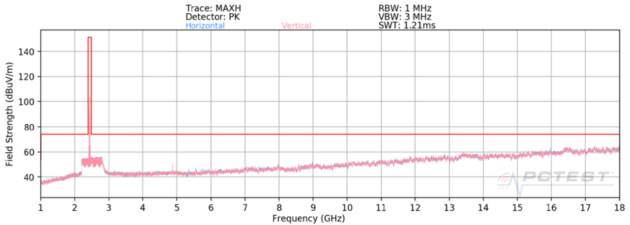
Plot 7-102. Radiated Spurious Plot above 1GHz SISO ANT1 (802.11b – Ch. 6)
