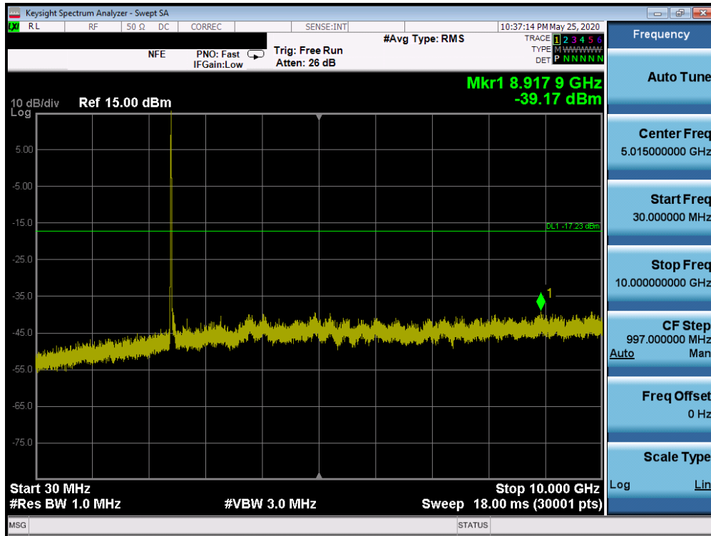
Plot 7-89. Conducted Spurious Plot SISO ANT1 (802.11b – Ch. 1)
