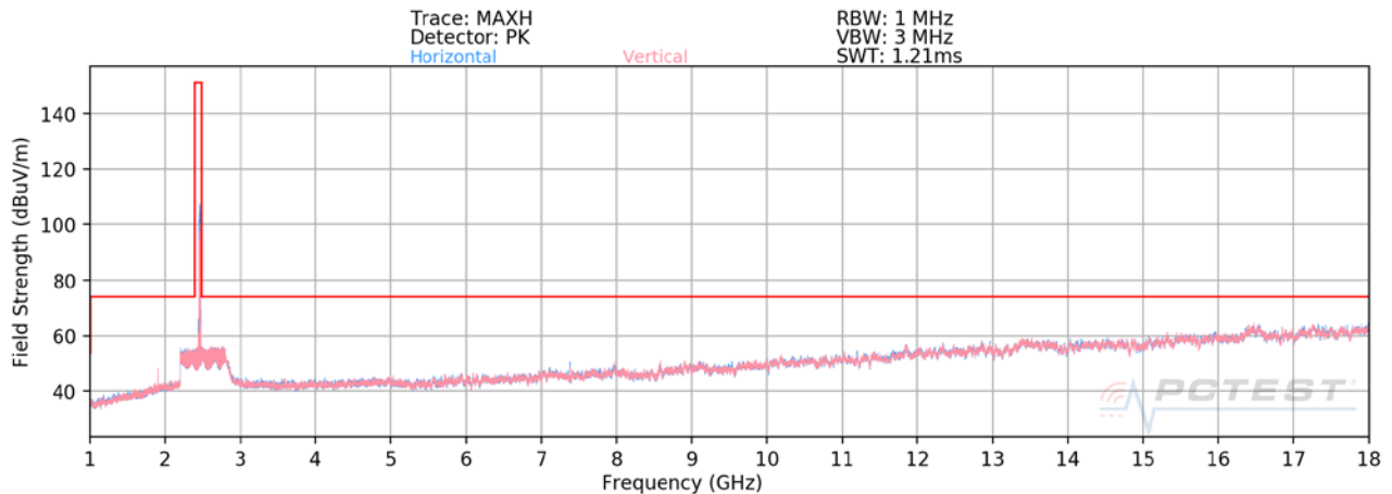
Plot 7-107. Radiated Spurious Plot above 1GHz SISO ANT2 (802.11b – Ch. 11)
