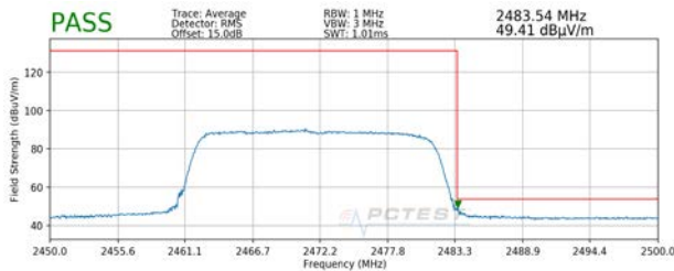
Plot 7-147. Radiated Restricted Upper Band Edge Measurement MIMO (Average)
