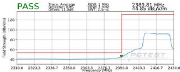
Plot 7-127. Radiated Restricted Lower Band Edge Measurement SISO ANT2 (Average)
