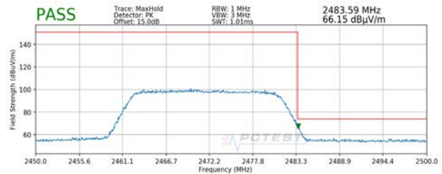
Plot 7-148. Radiated Restricted Upper Band Edge Measurement MIMO (Peak)
