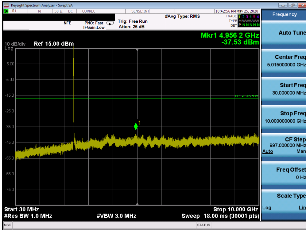
Plot 7-95. Conducted Spurious Plot SISO ANT2 (802.11b – Ch. 1)
