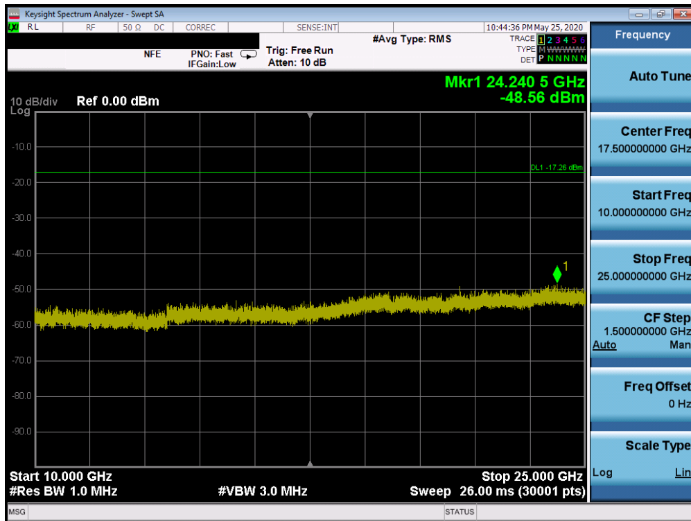
Plot 7-98. Conducted Spurious Plot SISO ANT2 (802.11b – Ch. 6)
