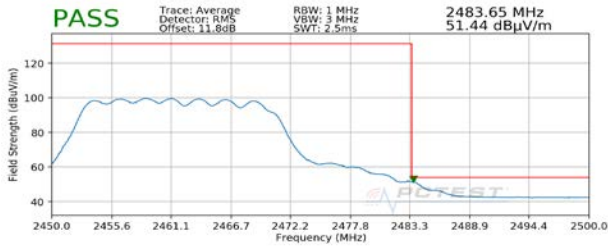
Plot 7-143. Radiated Restricted Upper Band Edge Measurement MIMO (Average)
