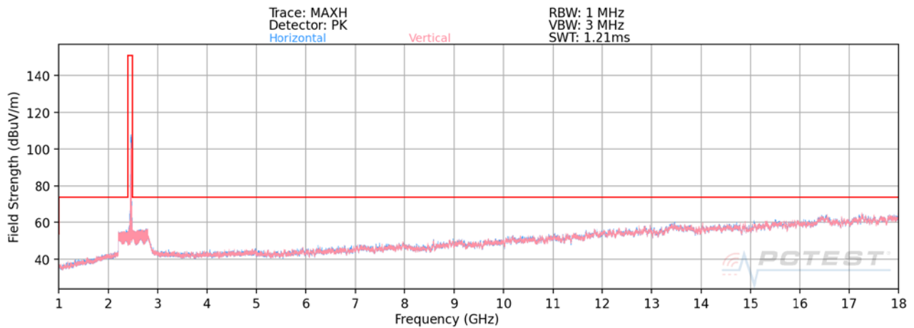
Plot 7-111. Radiated Spurious Plot above 1GHz MIMO/CDD (802.11g – Ch. 11)
