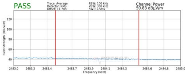
Plot 7-119. Radiated Restricted Upper Band Edge Measurement SISO ANT1 (Average)
