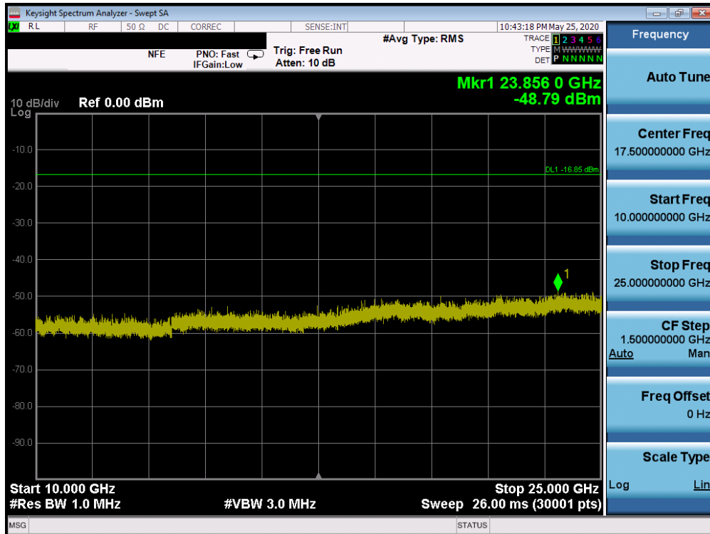
Plot 7-96. Conducted Spurious Plot SISO ANT2 (802.11b – Ch. 1)
