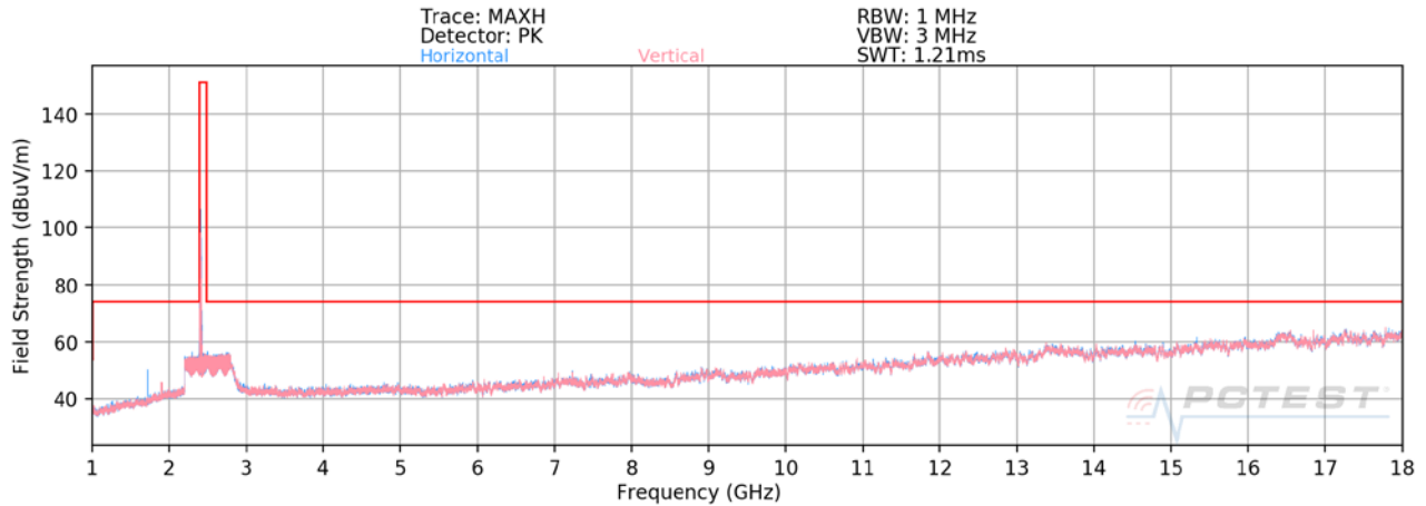
Plot 7-105. Radiated Spurious Plot above 1GHz SISO ANT2 (802.11b – Ch. 1)
