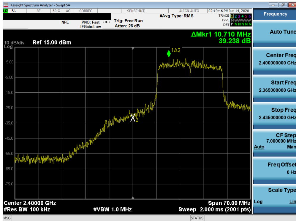
Plot 7-84. Band Edge Plot SISO ANT2 (802.11ax (2.4GHz) – Ch. 2)
