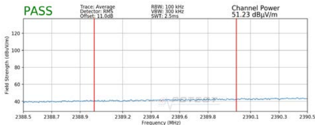
Plot 7-113. Radiated Restricted Lower Band Edge Measurement SISO ANT1 (Average)
