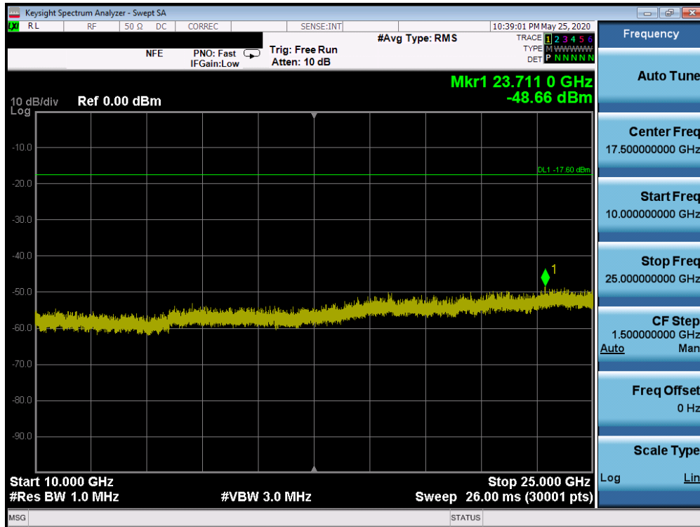
Plot 7-92. Conducted Spurious Plot SISO ANT1 (802.11b – Ch. 6)
