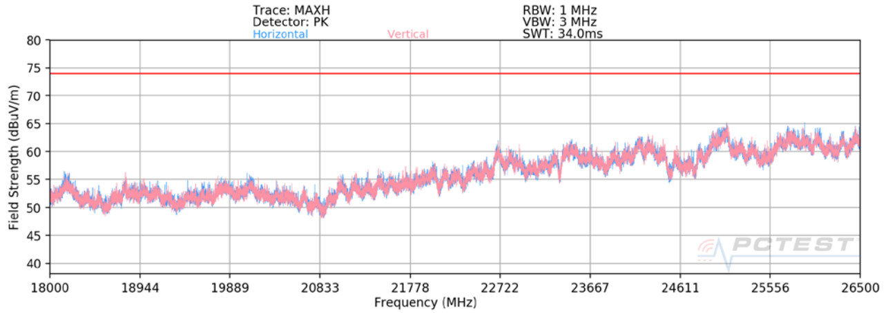
Plot 7-112. Radiated Spurious Plot above 18GHz MIMO/CDD
