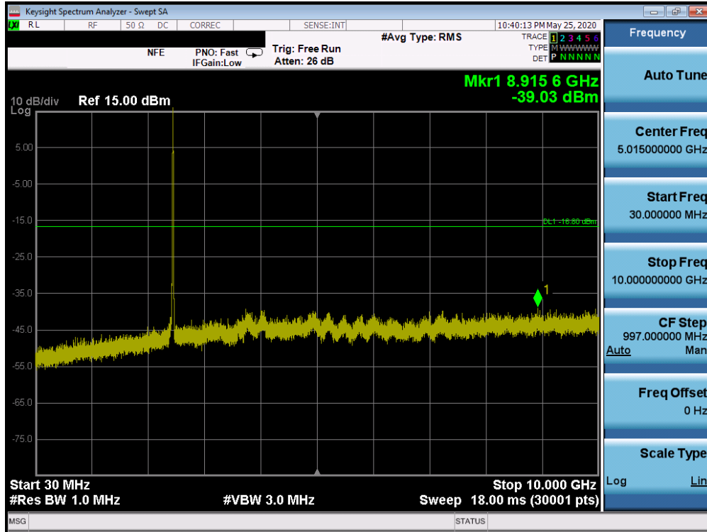
Plot 7-93. Conducted Spurious Plot SISO ANT1 (802.11b – Ch. 11)
