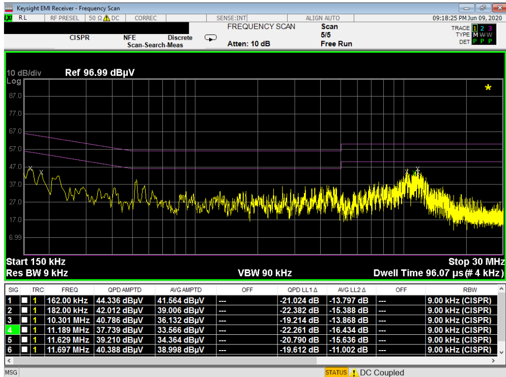
Plot 7-155. Line Conducted Plot with 802.11b (N) with WCP
