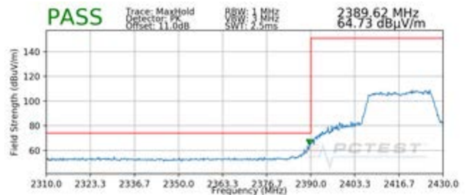
Plot 7-116. Radiated Restricted Lower Band Edge Measurement SISO ANT1 (Peak)
