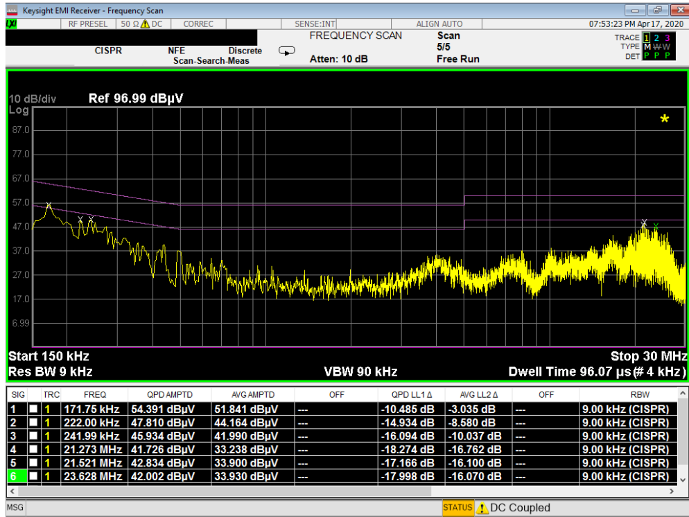
Plot 7-152. Line Conducted Plot with 802.11b (L1)
