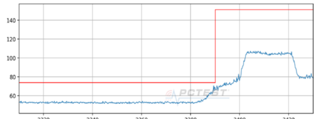
Plot 7-114. Radiated Restricted Lower Band Edge Measurement SISO ANT1 (Peak)
