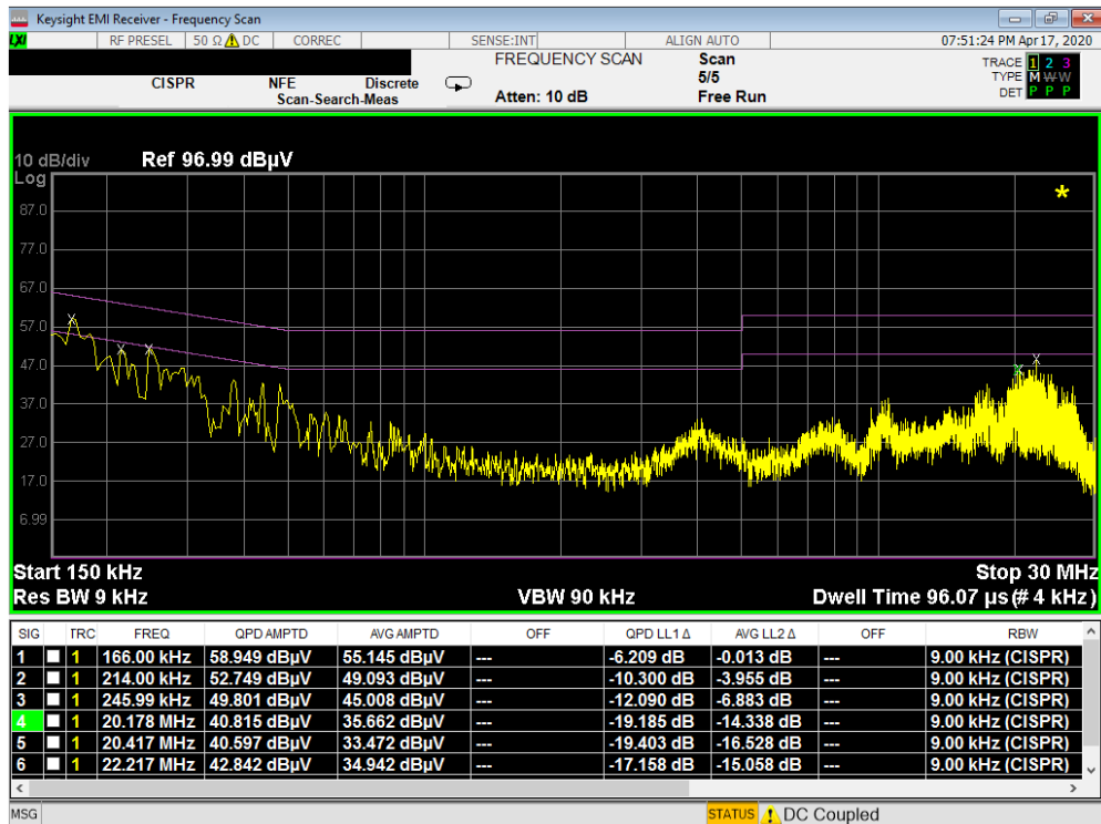
Plot 7-153. Line Conducted Plot with 802.11b (N)
