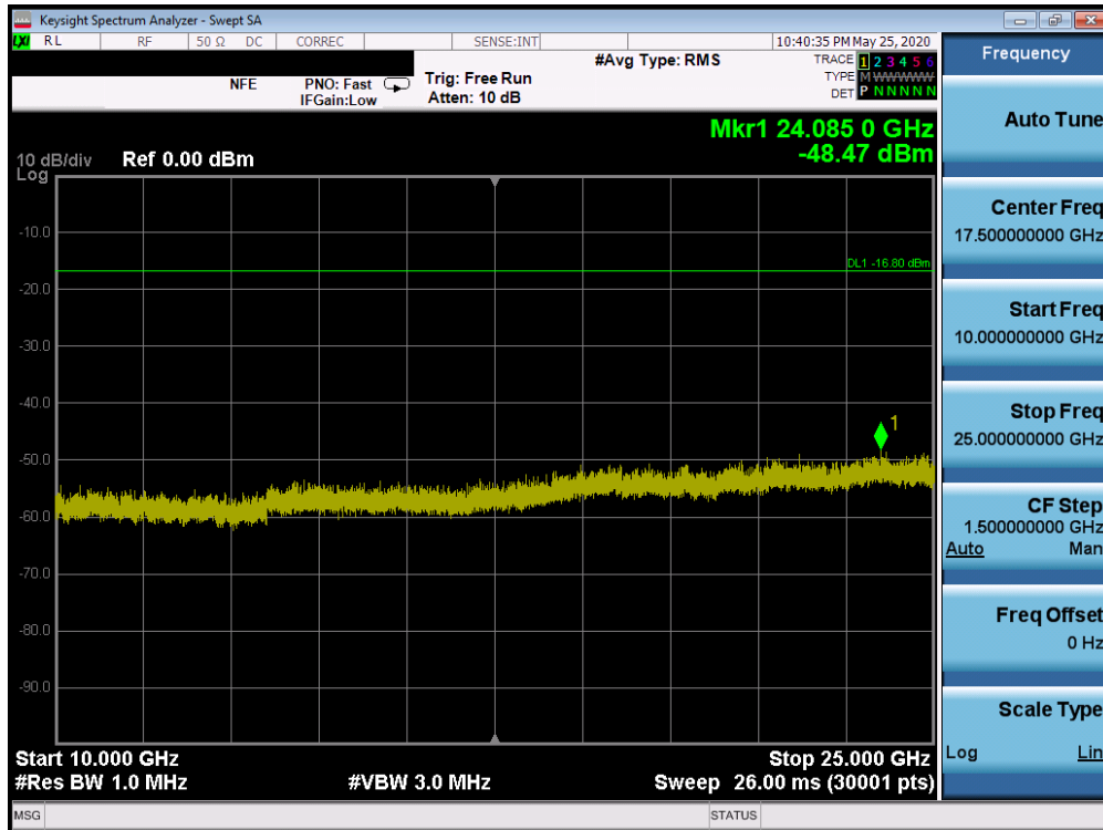
Plot 7-94. Conducted Spurious Plot SISO ANT1 (802.11b – Ch. 11)
