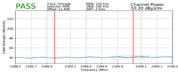
Plot 7-125. Radiated Restricted Lower Band Edge Measurement SISO ANT2 (Average)
