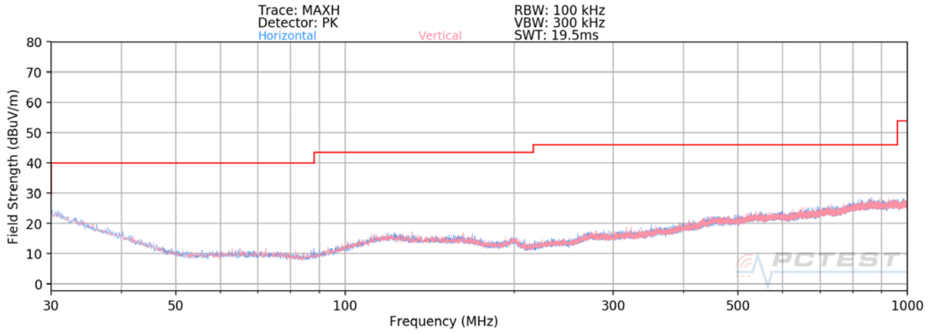
Plot 7-151. Radiated Spurious Plot below 1GHz
