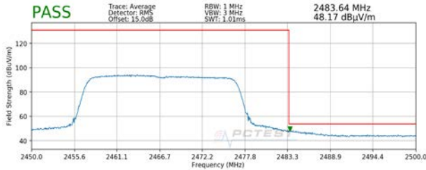
Plot 7-121. Radiated Restricted Upper Band Edge Measurement SISO ANT1 (Average)
