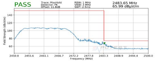
Plot 7-144. Radiated Restricted Upper Band Edge Measurement MIMO (Peak)
