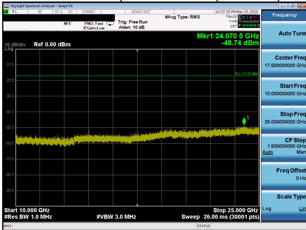
Plot 7-90. Conducted Spurious Plot SISO ANT1 (802.11b – Ch. 1)
