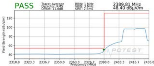
Plot 7-115. Radiated Restricted Lower Band Edge Measurement SISO ANT1 (Average)
