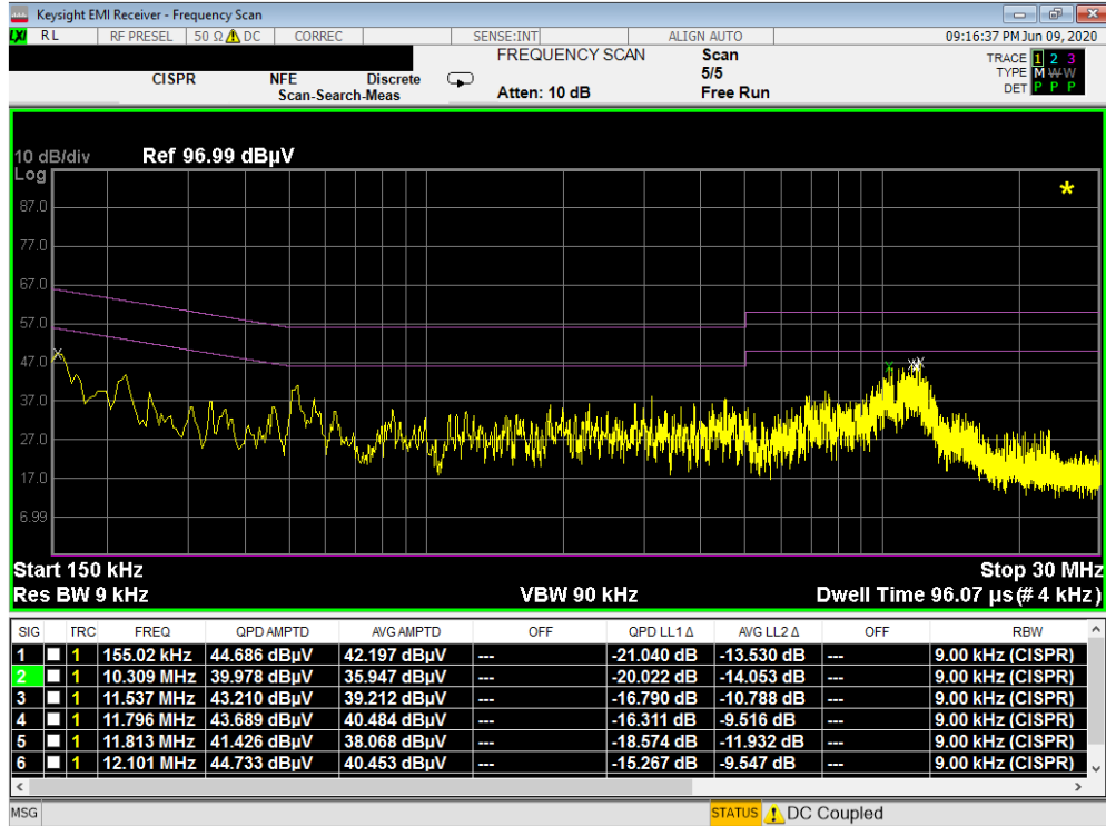
Plot 7-154. Line Conducted Plot with 802.11b (L1) with WCP
