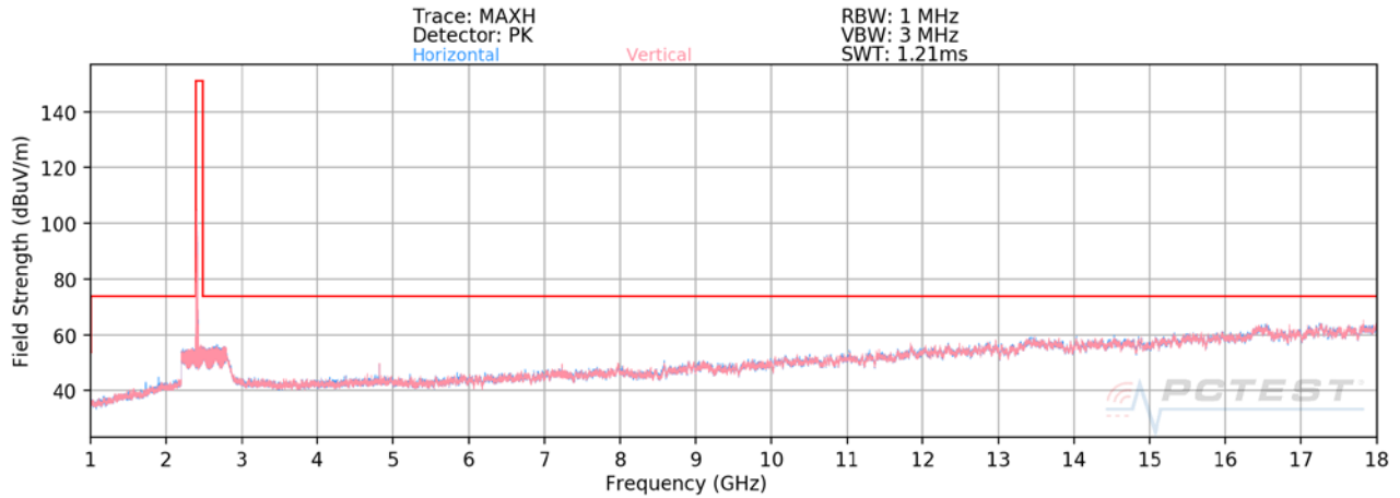
Plot 7-101. Radiated Spurious Plot above 1GHz SISO ANT1 (802.11b – Ch. 1)
