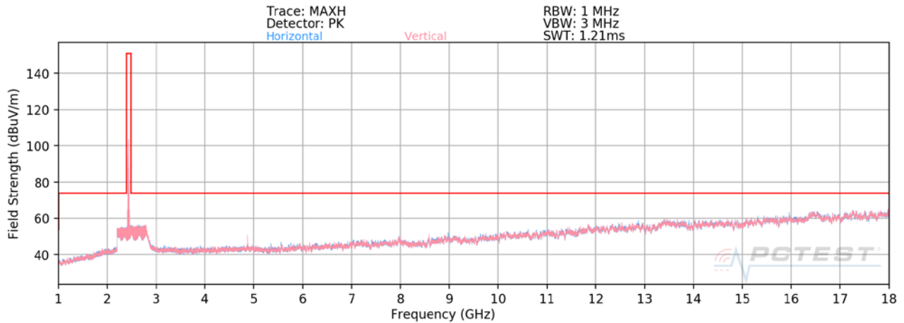
Plot 7-110. Radiated Spurious Plot above 1GHz MIMO/CDD (802.11g – Ch. 6)
