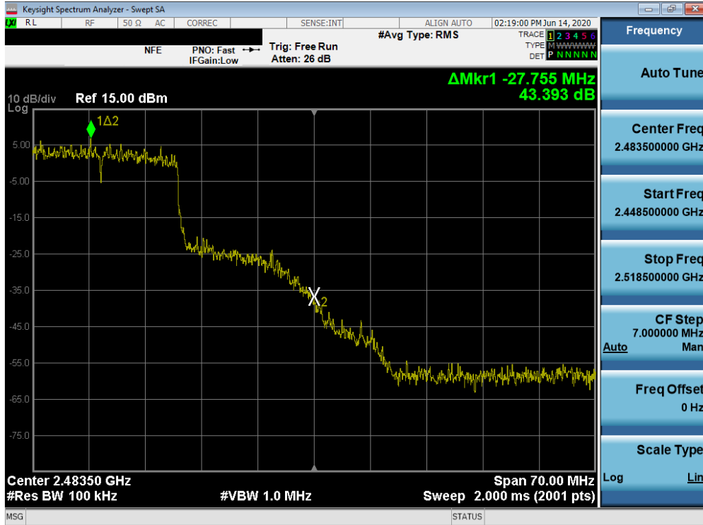
Plot 7-85. Band Edge Plot SISO ANT2 (802.11ax (2.4GHz) – Ch. 10)
