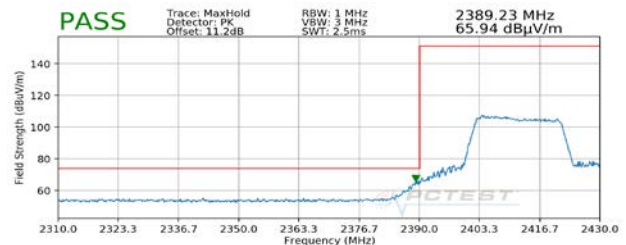
Plot 7-138. Radiated Restricted Lower Band Edge Measurement MIMO (Peak)
