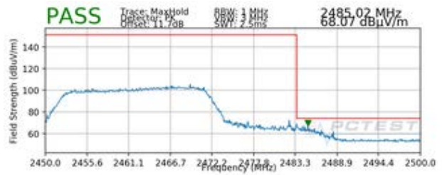
Plot 7-132. Radiated Restricted Upper Band Edge Measurement SISO ANT2 (Peak)
