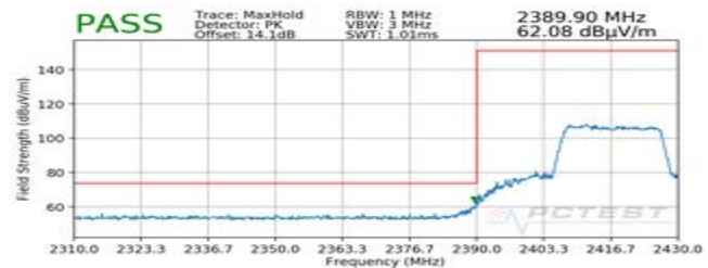
Plot 7-140. Radiated Restricted Lower Band Edge Measurement MIMO (Peak)
