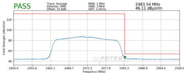
Plot 7-135. Radiated Restricted Upper Band Edge Measurement SISO ANT2 (Average)
