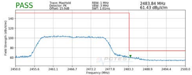
Plot 7-122. Radiated Restricted Upper Band Edge Measurement SISO ANT1 (Peak)
