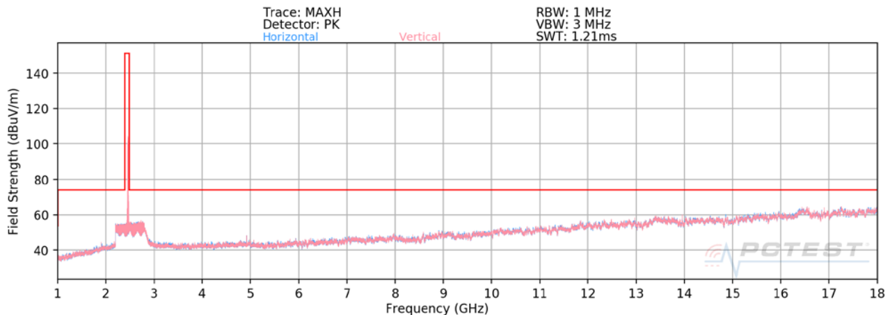
Plot 7-103. Radiated Spurious Plot above 1GHz SISO ANT1 (802.11b – Ch. 11)
