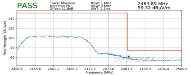
Plot 7-150. Radiated Restricted Band Edge Measurement MIMO with WCP (Peak)
