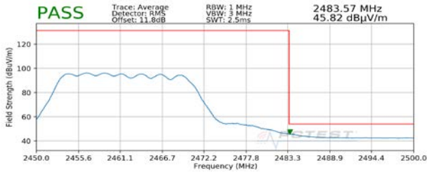
Plot 7-149. Radiated Restricted Band Edge Measurement MIMO with WCP (Average)
