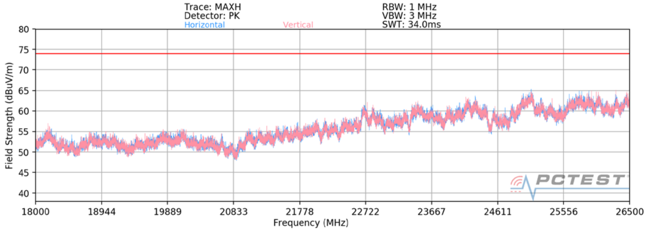
Plot 7-104. Radiated Spurious Plot above 18GHz SISO ANT1
