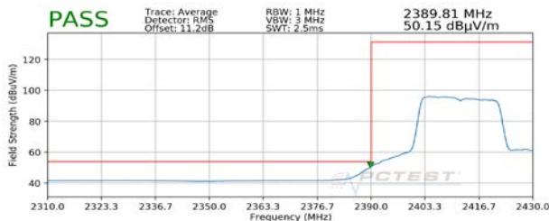
Plot 7-137. Radiated Restricted Lower Band Edge Measurement MIMO (Average)
