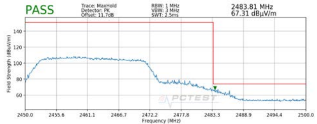
Plot 7-120. Radiated Restricted Upper Band Edge Measurement SISO ANT1 (Peak)
