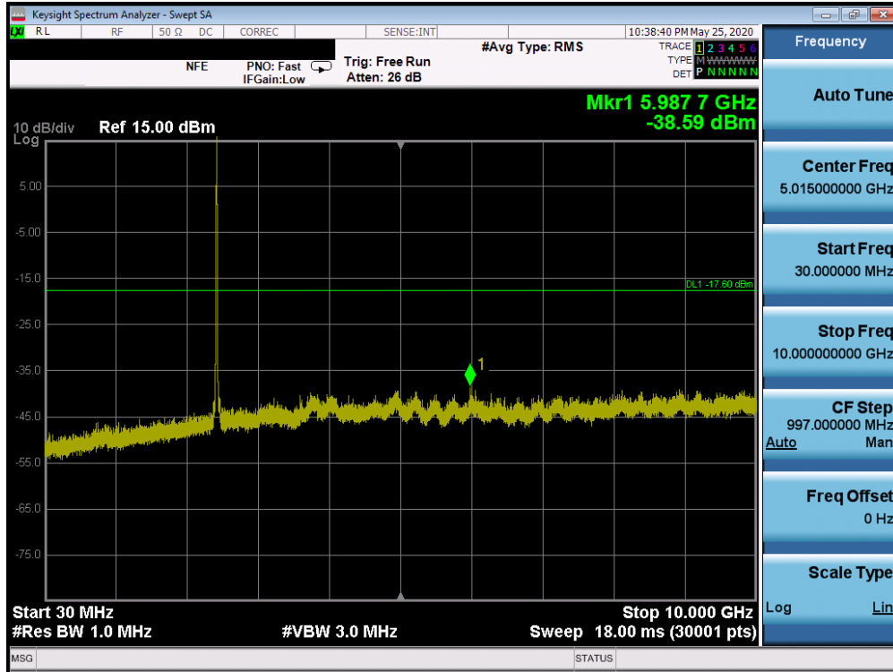
Plot 7-91. Conducted Spurious Plot SISO ANT1 (802.11b – Ch. 6)
