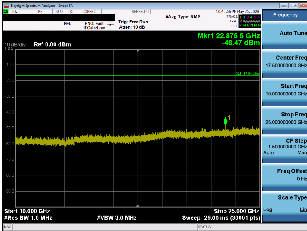
Plot 7-100. Conducted Spurious Plot SISO ANT2 (802.11b – Ch. 11)
