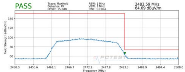
Plot 7-136. Radiated Restricted Upper Band Edge Measurement SISO ANT2 (Peak)
