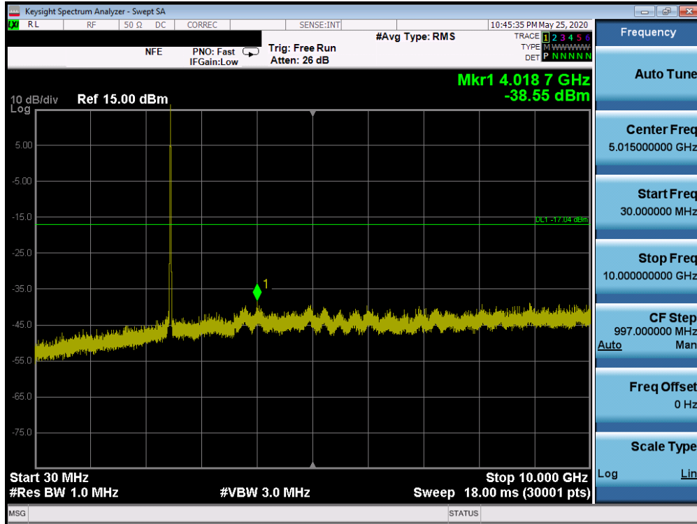
Plot 7-99. Conducted Spurious Plot SISO ANT2 (802.11b – Ch. 11)
