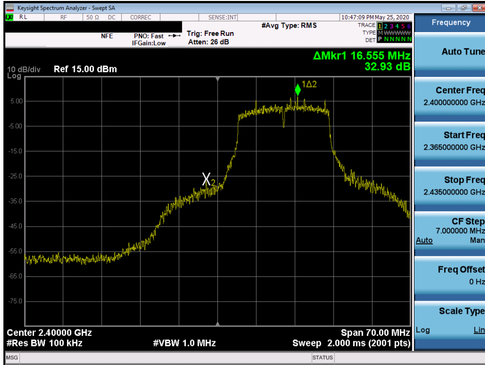
Plot 7-73. Band Edge Plot SISO ANT2 (802.11g- Ch. 1)
