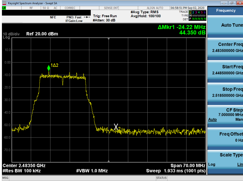
Plot 7-75. Band Edge Plot SISO ANT2 (802.11g – Ch. 12)
