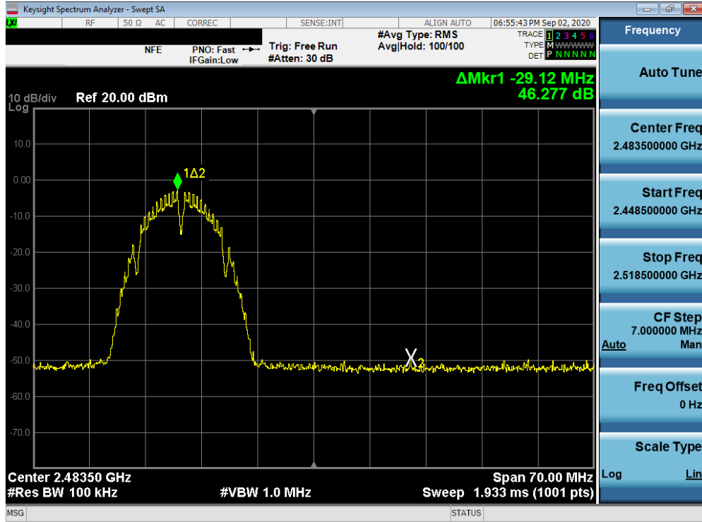
Plot 7-71. Band Edge Plot SISO ANT2 (802.11b – Ch. 12)
