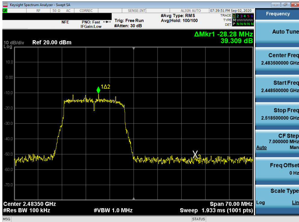
Plot 7-62. Band Edge Plot SISO ANT1 (802.11n (2.4GHz) – Ch. 13)
