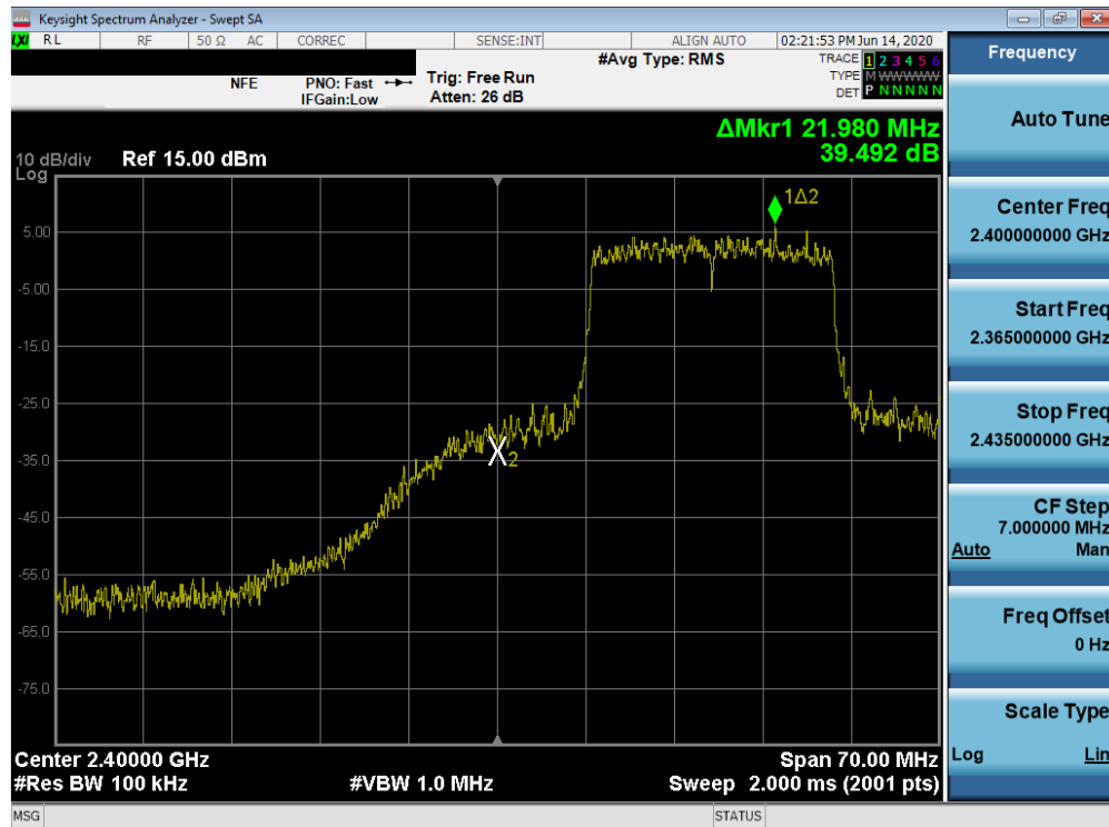
Plot 7-64. Band Edge Plot SISO ANT1 (802.11ax (2.4GHz) – Ch. 2)
