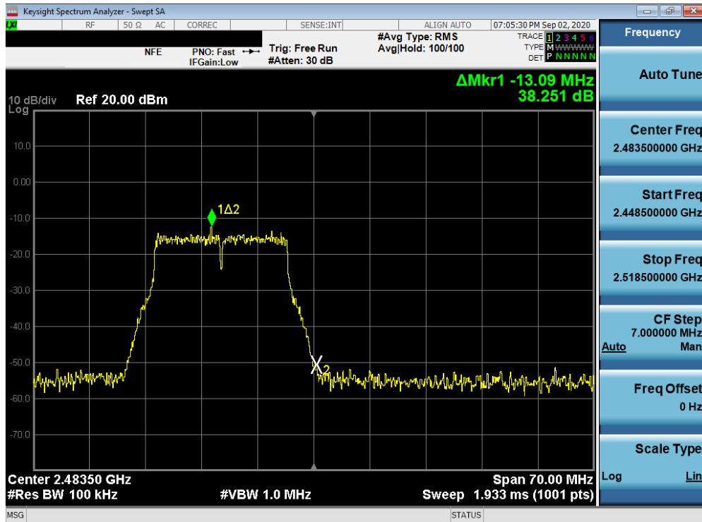
Plot 7-76. Band Edge Plot SISO ANT2 (802.11g – Ch. 13)
