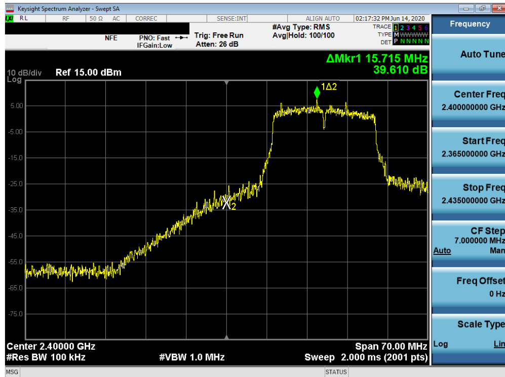
Plot 7-78. Band Edge Plot SISO ANT2 (802.11n (2.4GHz) – Ch. 2)
