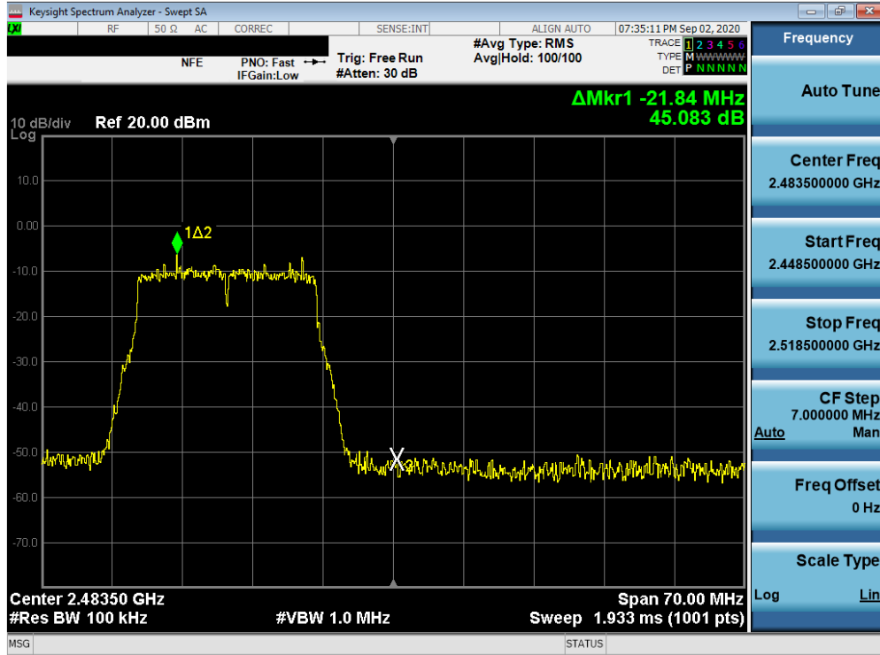
Plot 7-61. Band Edge Plot SISO ANT1 (802.11n (2.4GHz) – Ch. 12)
