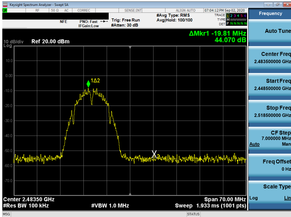
Plot 7-72. Band Edge Plot SISO ANT2 (802.11b – Ch. 13)
