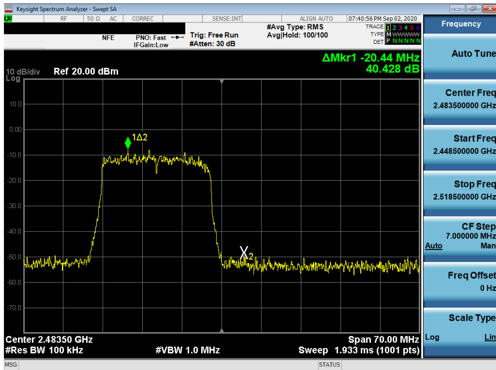
Plot 7-68. Band Edge Plot SISO ANT1 (802.11ax (2.4GHz) – Ch. 13)
