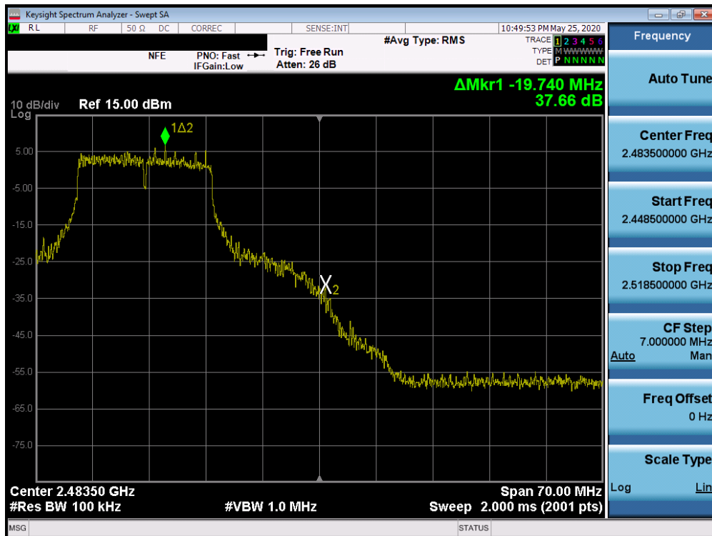
Plot 7-74. Band Edge Plot SISO ANT2 (802.11g - Ch. 11)
