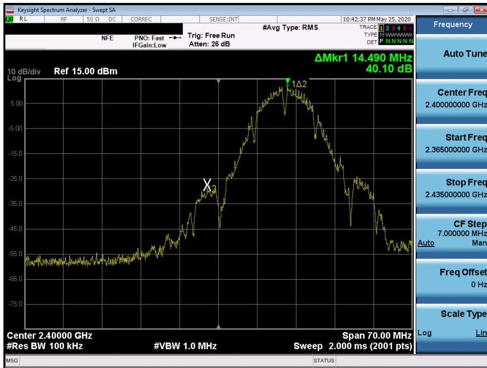
Plot 7-69. Band Edge Plot SISO ANT2 (802.11b – Ch. 1)
