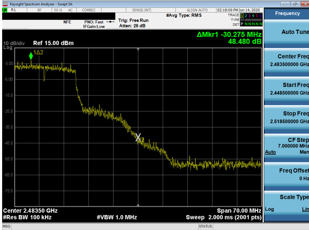
Plot 7-79. Band Edge Plot SISO ANT2 (802.11n (2.4GHz) – Ch. 10)
