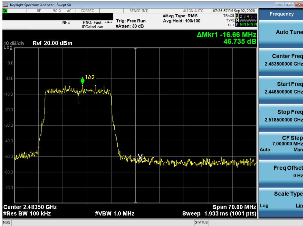
Plot 7-67. Band Edge Plot SISO ANT1 (802.11ax (2.4GHz) – Ch. 12)
