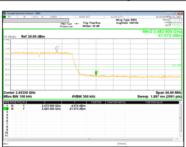
12 Channel Band-edge
