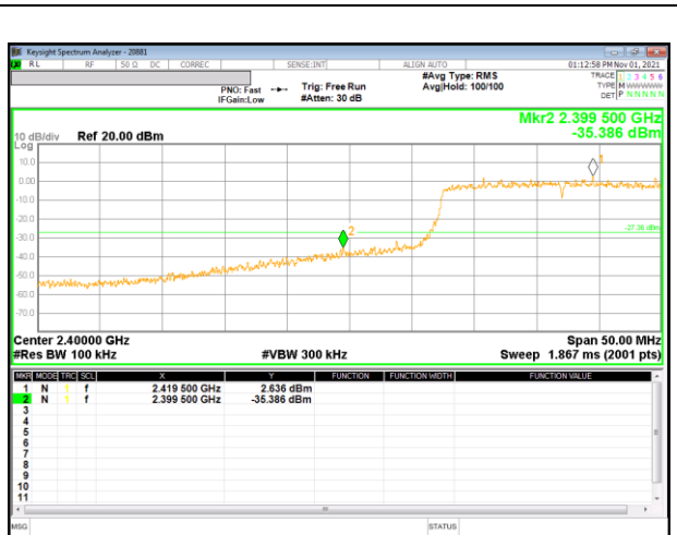
2 Channel Band-edge
