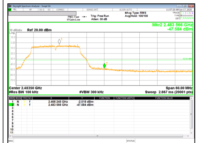
12 Channel Band-edge
