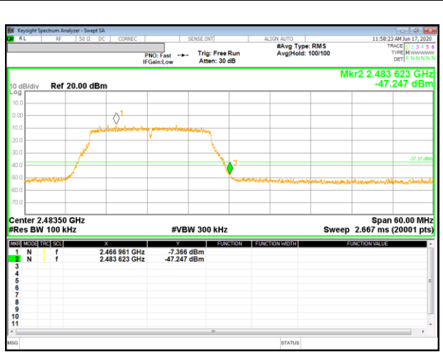
13 Channel Band-edge
