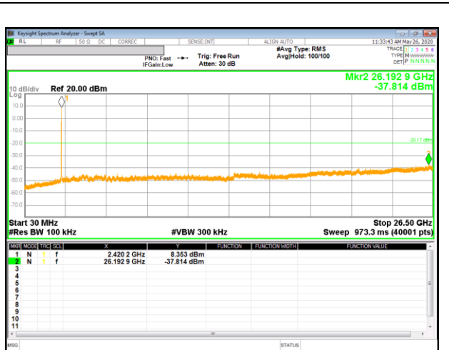
Out-Of-Band 1 Channel(8RU)
