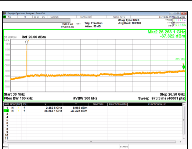
Out-Of-Band 11 Channel(4RU)
