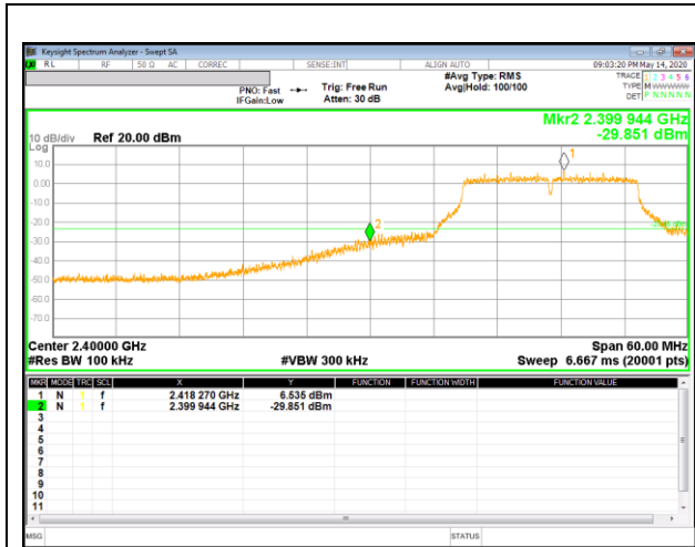
2 Channel Band-edge
