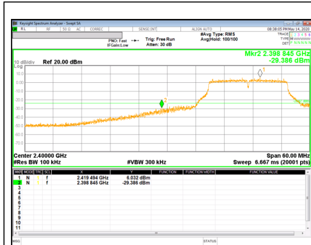
2 Channel Band-edge
