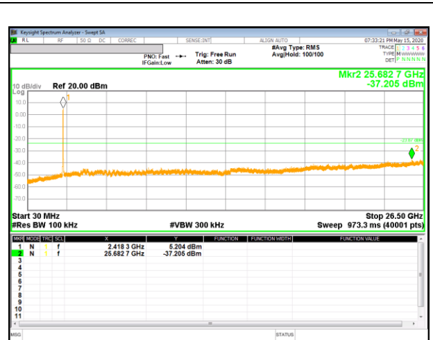
Out-Of-Band 2 Channel
