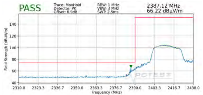
Plot 7-93. Radiated Restricted Lower Band Edge Measurement SISO ANT2 (Peak)
