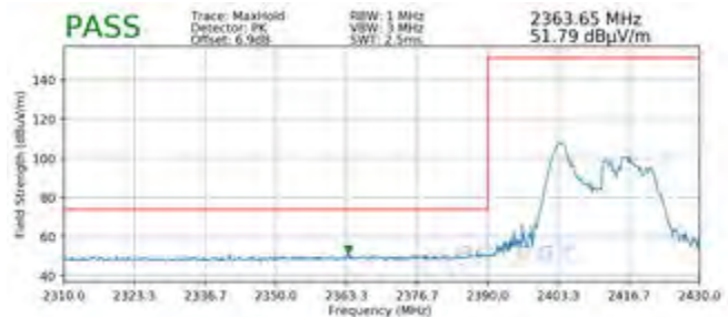
Plot 7-110. Radiated Restricted Lower Band Edge Measurement MIMO (Peak – 26 Tones)
