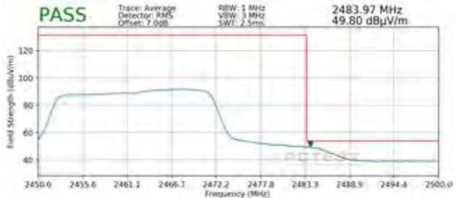
Plot 7-107. Radiated Restricted Upper Band Edge Measurement SISO ANT2 (Average – 242 Tones)
