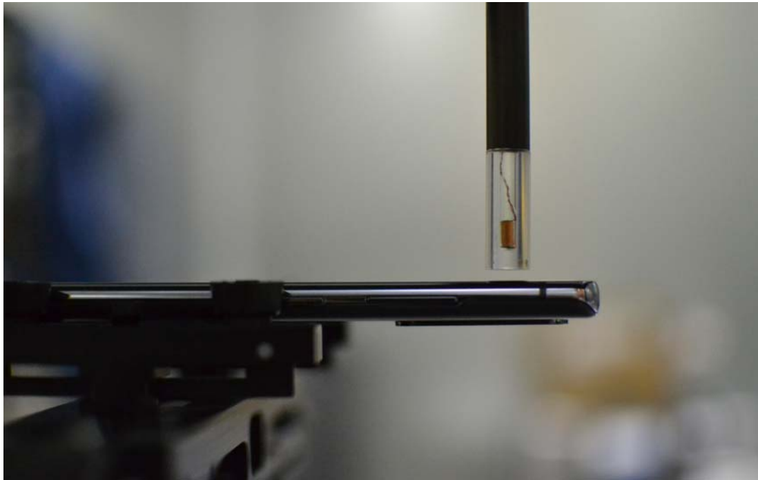
Figure 16-2 Test Setup for Wireless Device
