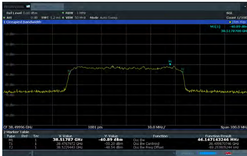
Plot 7-18. Ant 1 Occupied Bandwidth Plot (50MHz-1CC – 16QAM – Mid Channel)
